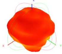
2500.0MHz H+V, Eff: 50.2%
