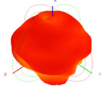
2480.0MHz H+V, Eff: 51.6%
