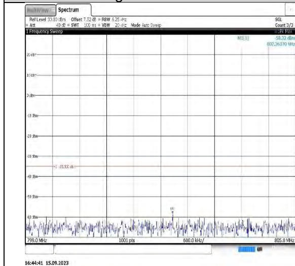
Band14-5MHz-16QAM-23305-1RB#0- Range3:799~805MHz
