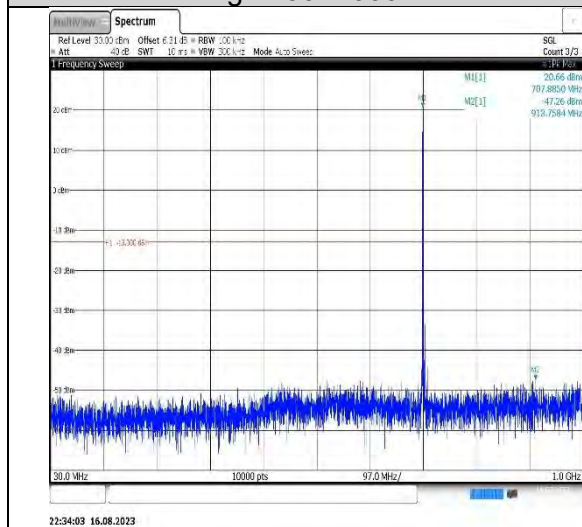
Band17-5MHz-QPSK-23790-1RB#0- Range1:30~1000MHz
