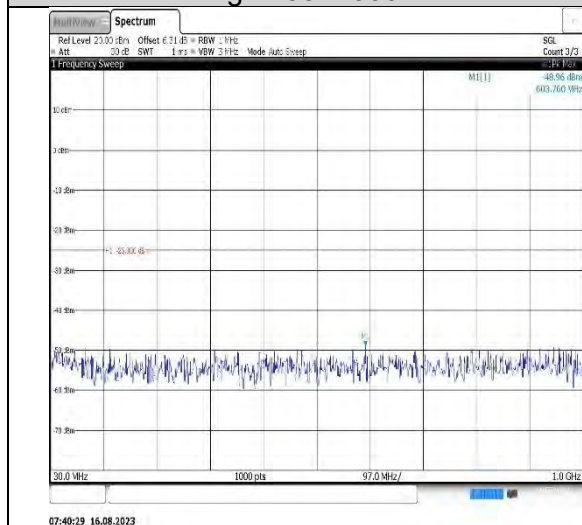
Band7-5MHz-16QAM-20775-1RB#0- Range1:30~1000MHz
