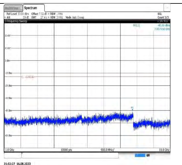
Band12-10MHz-16QAM-23130-1RB#0-Range2:1000~10000MHz
