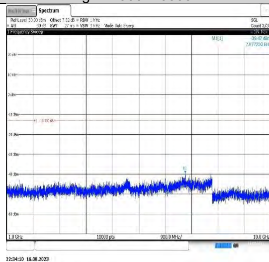
Band17-5MHz-QPSK-23790-1RB#0- Range2:1000~10000MHz
