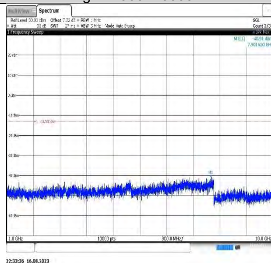
Band17-5MHz-QPSK-23790-1RB#0- Range2:1000~10000MHz
