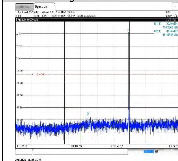
Band17-5MHz-QPSK-23790-1RB#0- Range1:30~1000MHz
