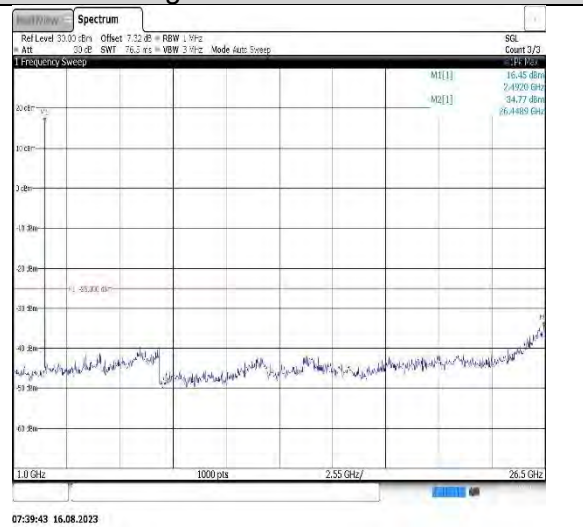
Band7-5MHz-16QAM-20775-1RB#0- Range2:1000~26500MHz
