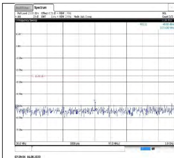
Band7-5MHz-QPSK-21425-1RB#0- Range1:30~1000MHz
