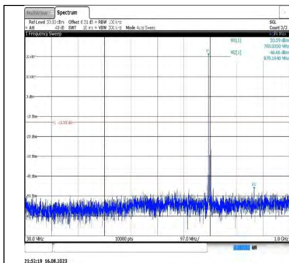
Band12-10MHz-16QAM-23130-1RB#0-Range1:30~1000MHz
