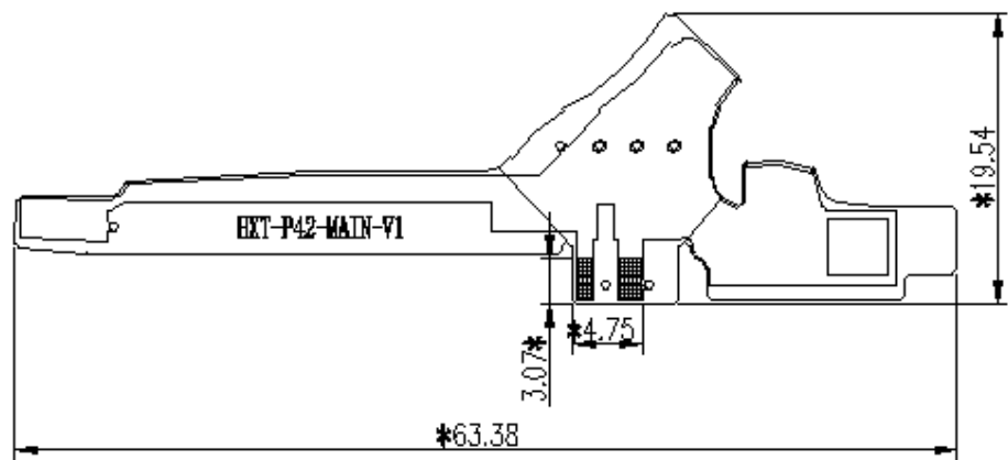
WWAN MAIN ANT
