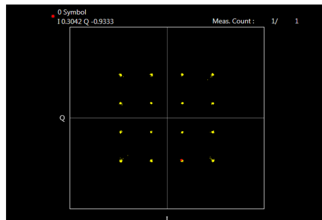
16QAM
