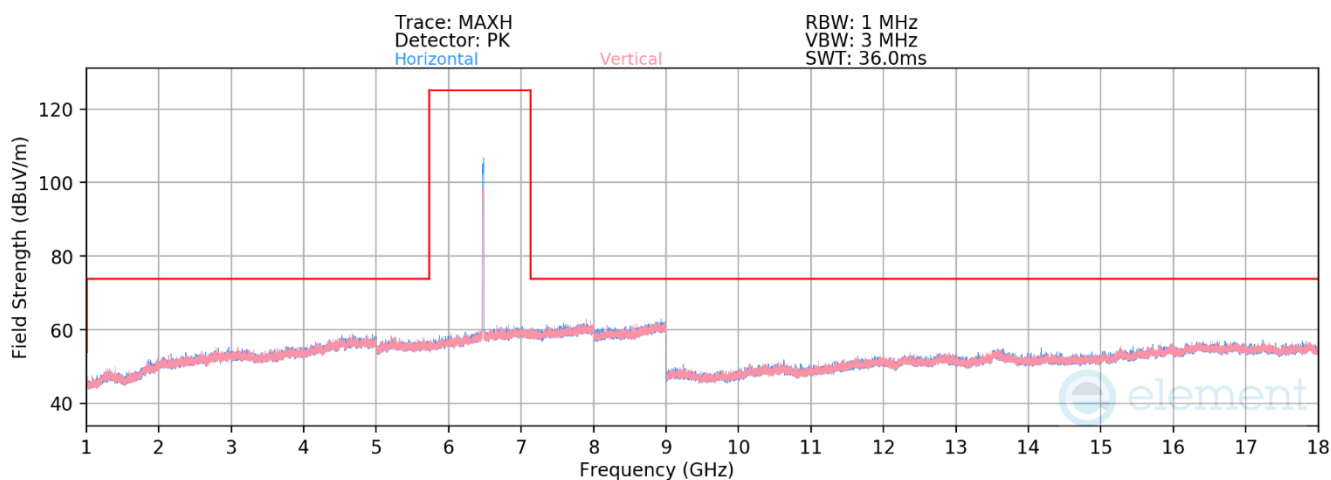
Plot 7-2. Radiated Spurious Emissions above 1GHz SDM (802.11ax – Ch. 105, MCS2)
