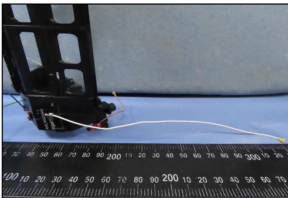
Antenna NO.3
