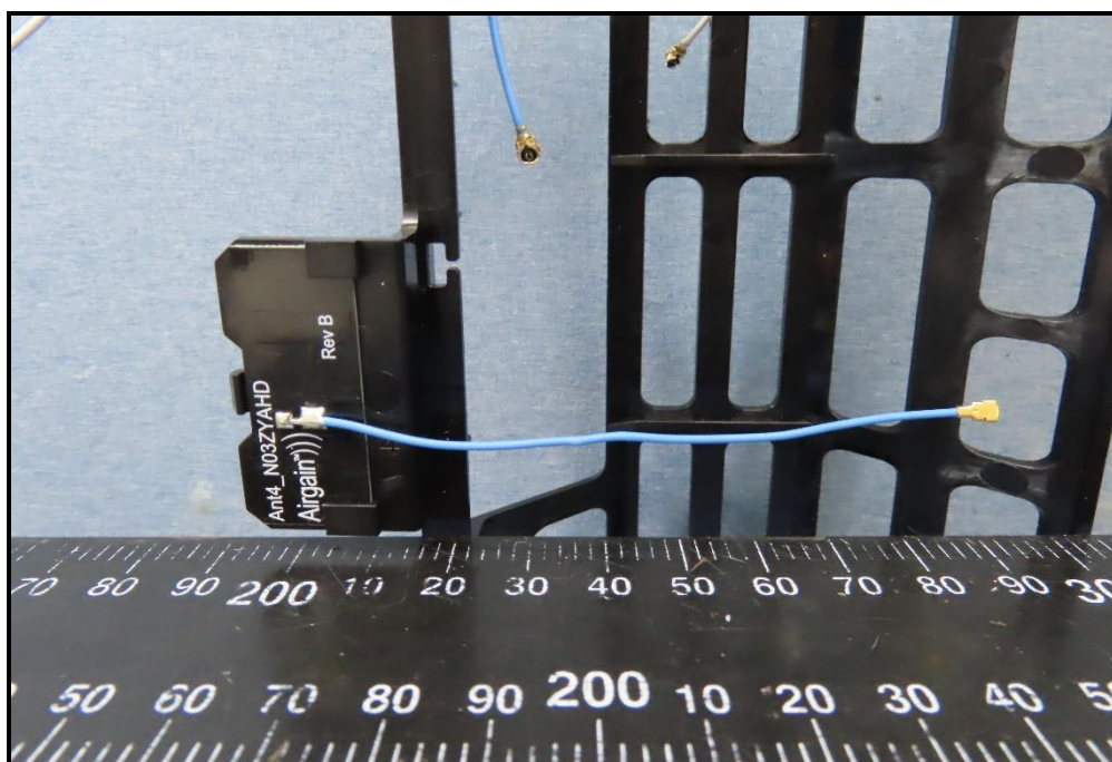
Antenna NO.4
