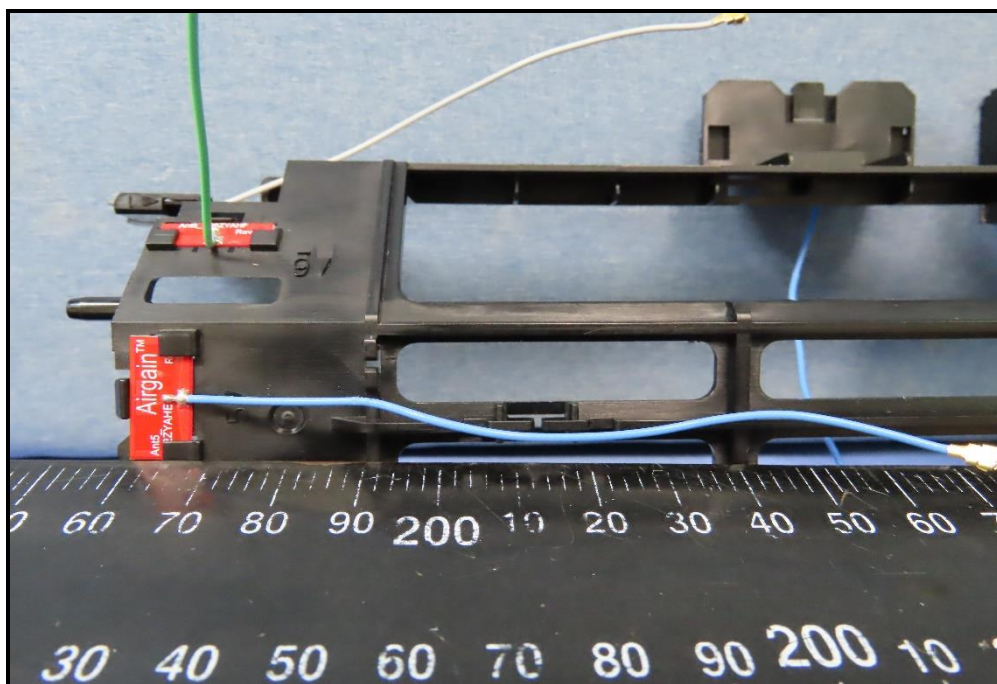
Antenna NO.5
