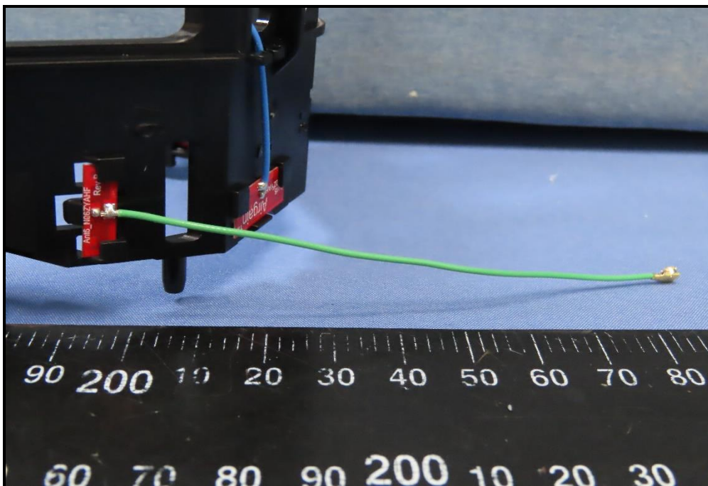
Antenna NO.6
