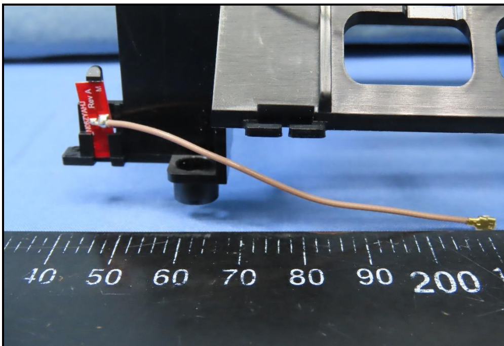
Antenna NO.9
