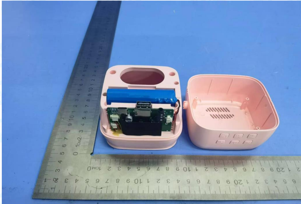
Photo 31 Internal of EUT
