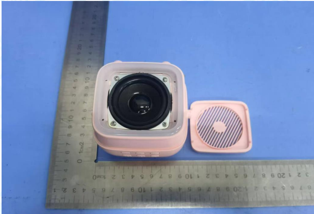
Photo 30 Internal of EUT
