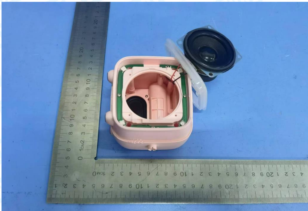
Photo 30 Internal of EUT
