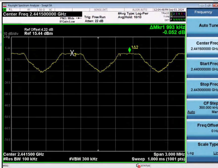
Carrier_Frequencies_Separation_(Hopping)_NVNT_ANT1_2-DH5_Hopping
