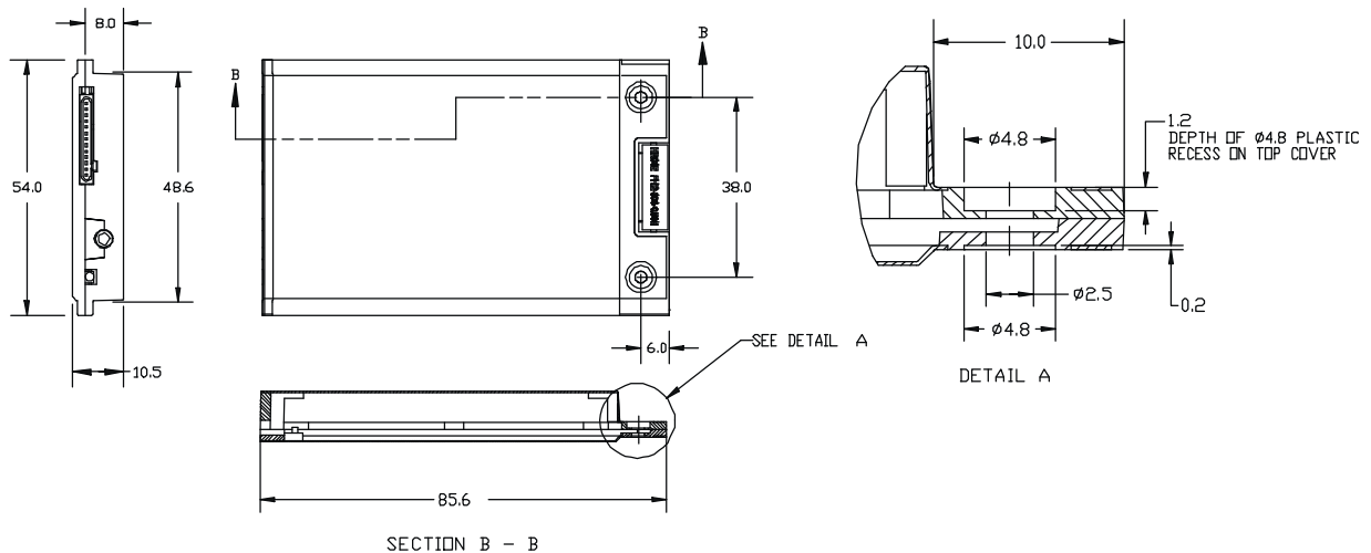
Figure 9-1: SB300 Physical Dimensions [mm].
