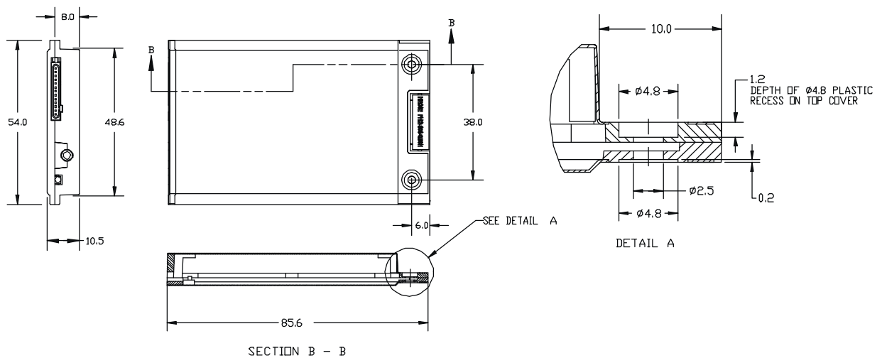
Figure 9-5: SB320 Physical Dimensions [mm].
