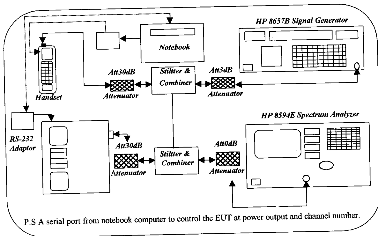
Fig 13. Test Configuration of processing gain for base station
