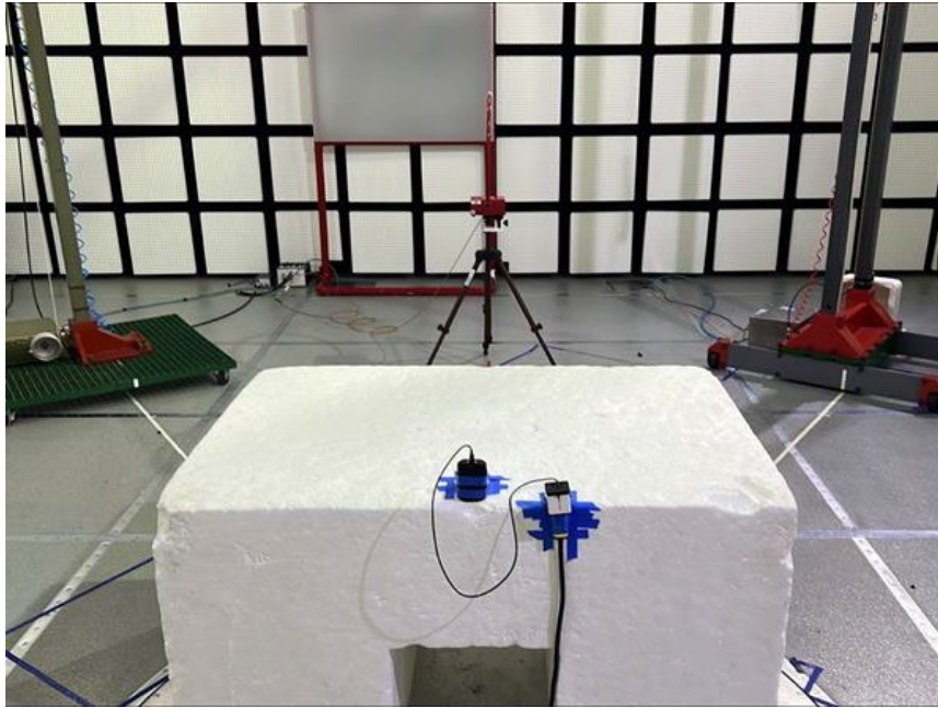
RADIATED PHOTO (<30 MHz 2.4 WLAN)
