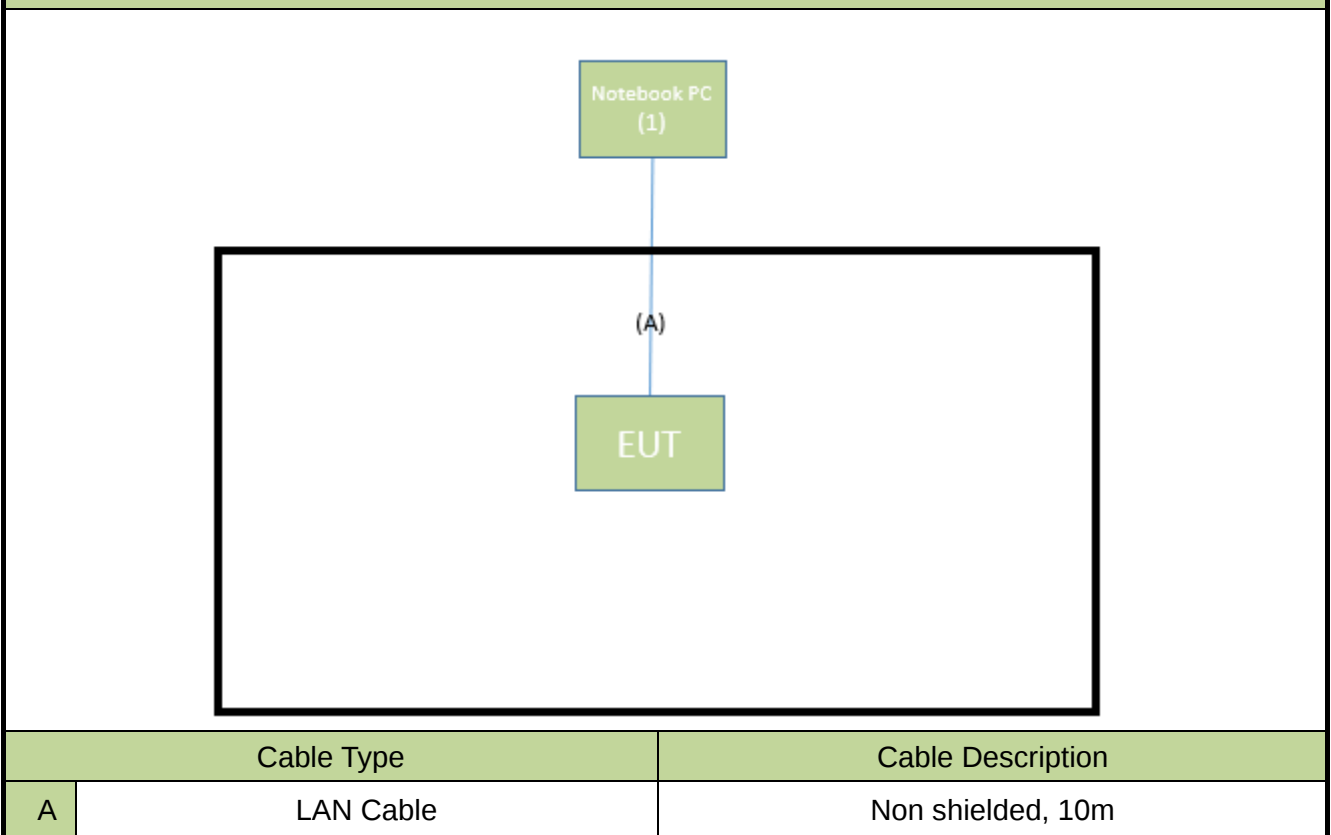
Connection Diagram
