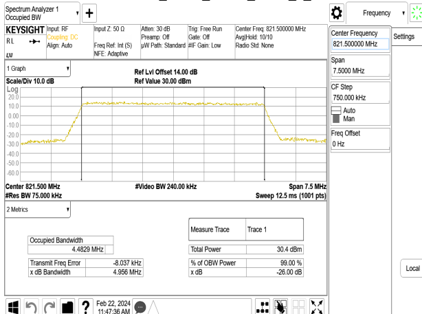
Band26-Part90s_5MHz_QPSK_RB25_0_CH26765
