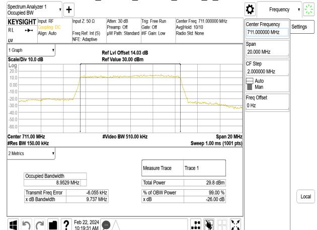
Band17_10MHz_64QAM_RB50_0_CH23800
