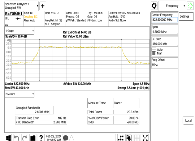
Band26-Part90s_3MHz_64QAM_RB15_0_CH26775
