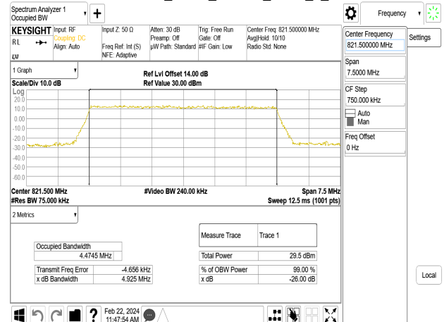
Band26-Part90s_5MHz_16QAM_RB25_0_CH26765
