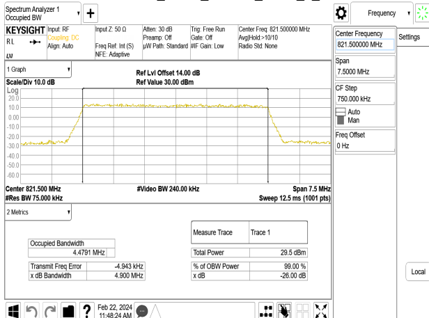
Band26-Part90s_5MHz_64QAM_RB25_0_CH26765
