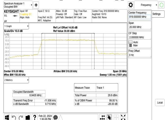
Band26-Part90s_10MHz_64QAM_RB50_0_CH26740
