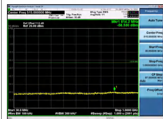
Band4-15MHz-QPSK-20025-75RB#0-30~1000-P ASS
