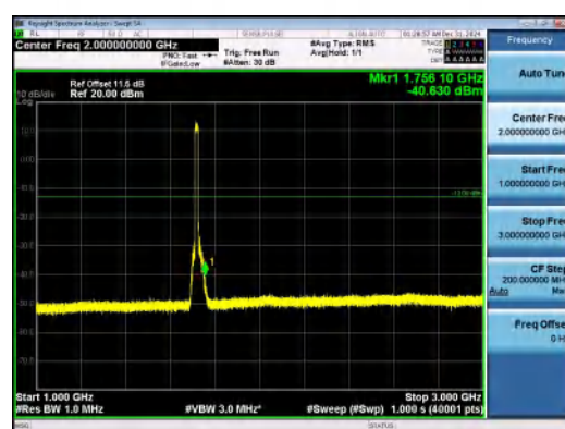
Band4-15MHz-QPSK-20025-75RB#0-1000~300 0-PASS
