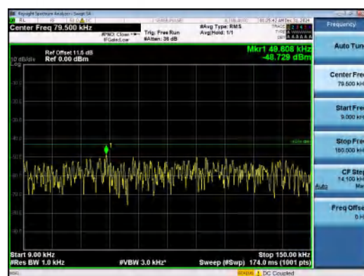
Band4-15MHz-16QAM-20025-1RB#0-0.009~0.1 5-PASS
