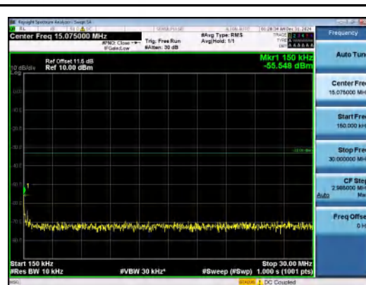
Band4-15MHz-QPSK-20025-75RB#0-0.15~30-P ASS
