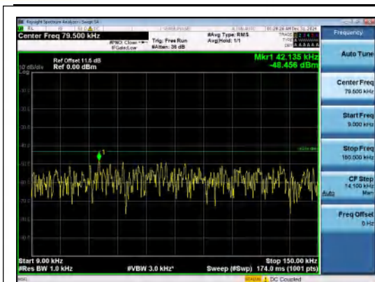
Band4-15MHz-QPSK-20025-75RB#0-0.009~0.1 5-PASS
