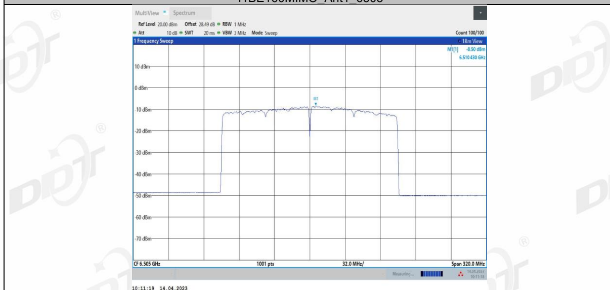
11BE160MIMO Ant2 6505
