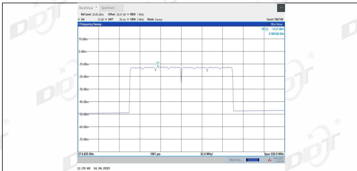
11BE160MIMO Ant2_6825
