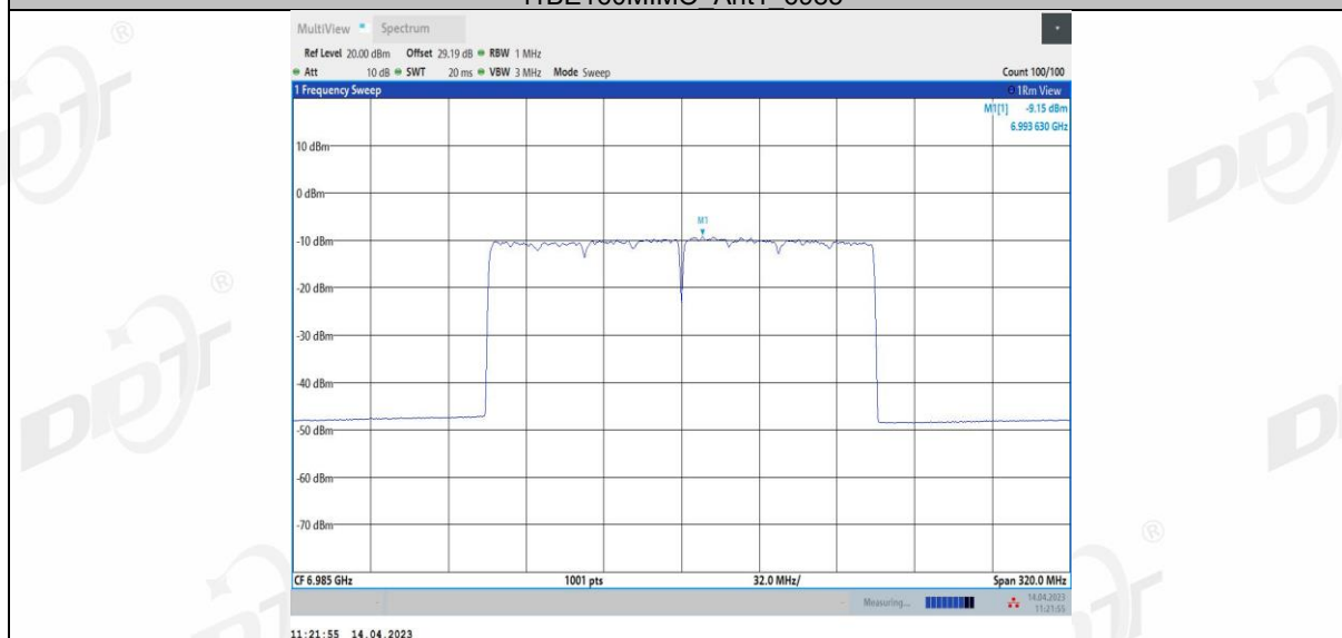
11BE160MIMO Ant2 6985
