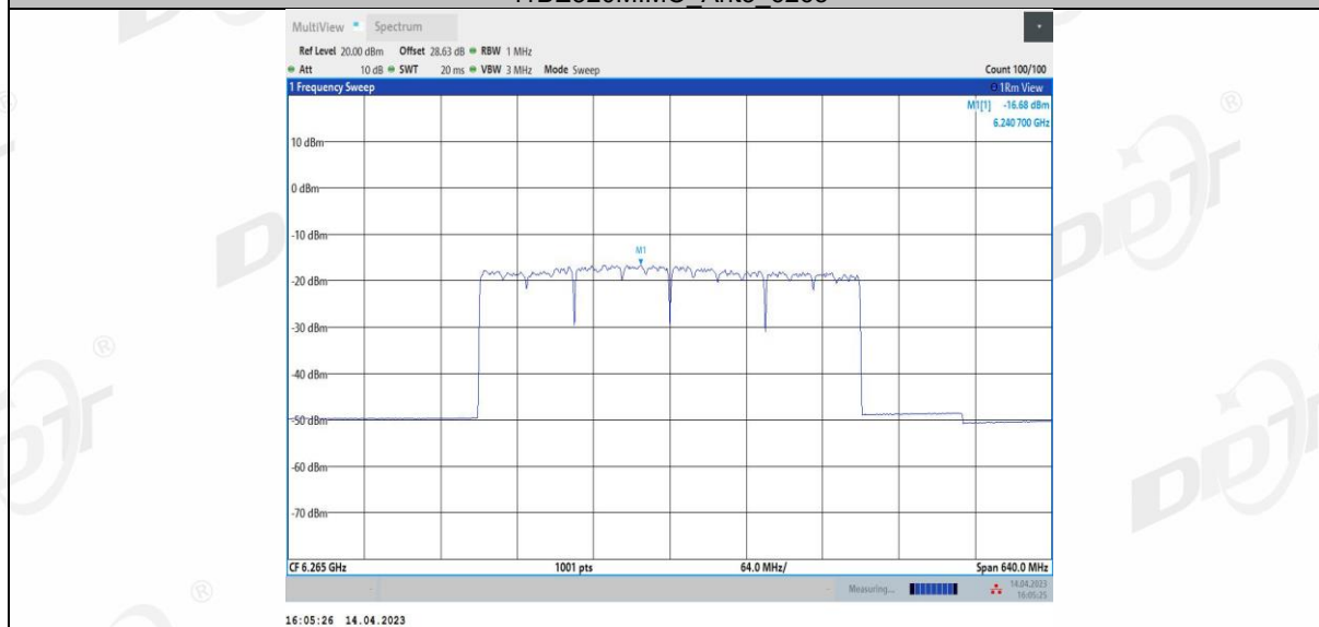
11BE320MIMO Ant4_6265
