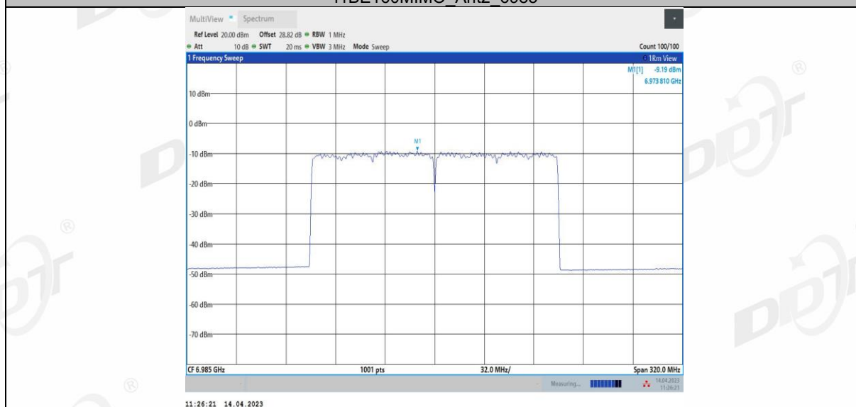
11BE160MIMO Ant3 6985
