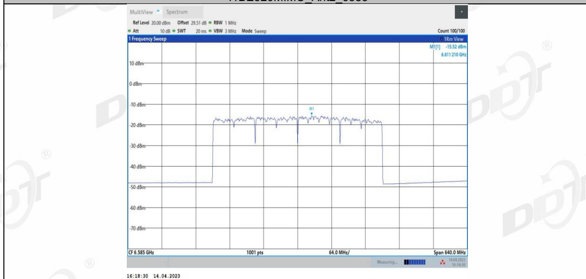
11BE320MIMO Ant3_6585
