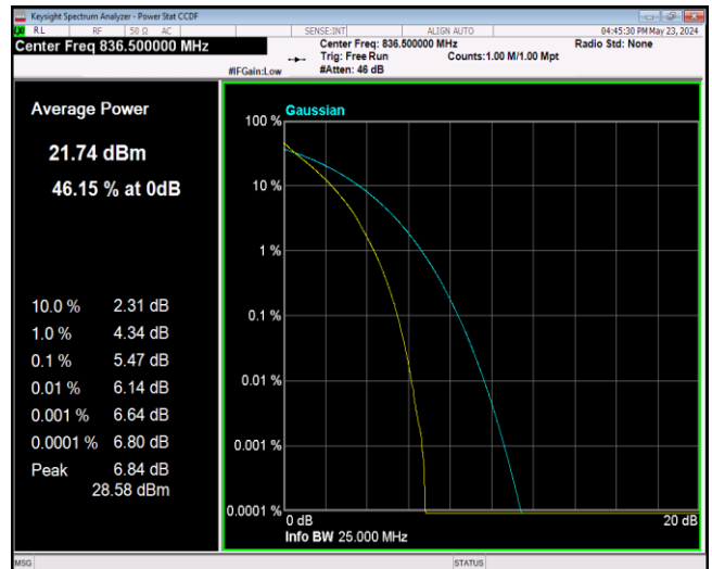
Band5-10MHz-64QAM-20525-50RB#0
