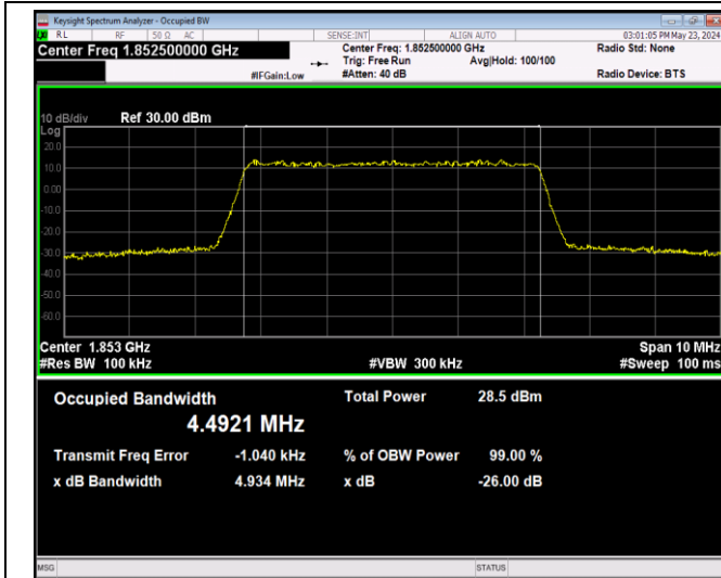
Band2-5MHz-64QAM-19175-25RB#0
