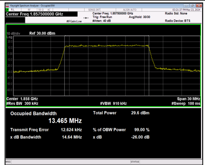
Band2-15MHz-16QAM-19125-75RB#0
