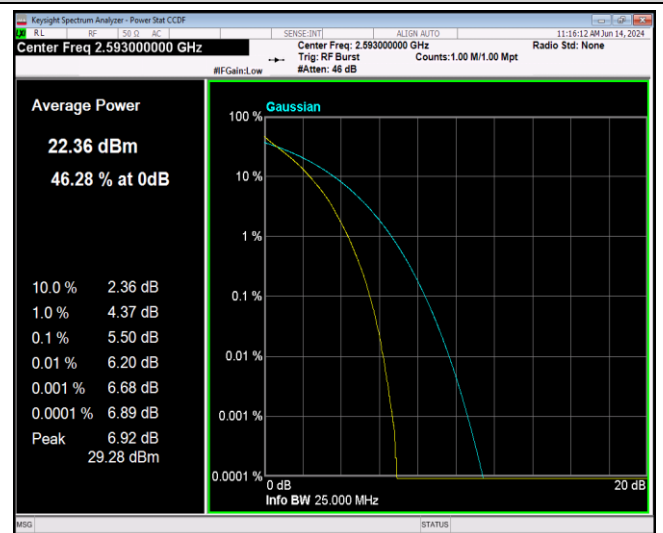
Band41-20MHz-64QAM-40620-100RB#0
