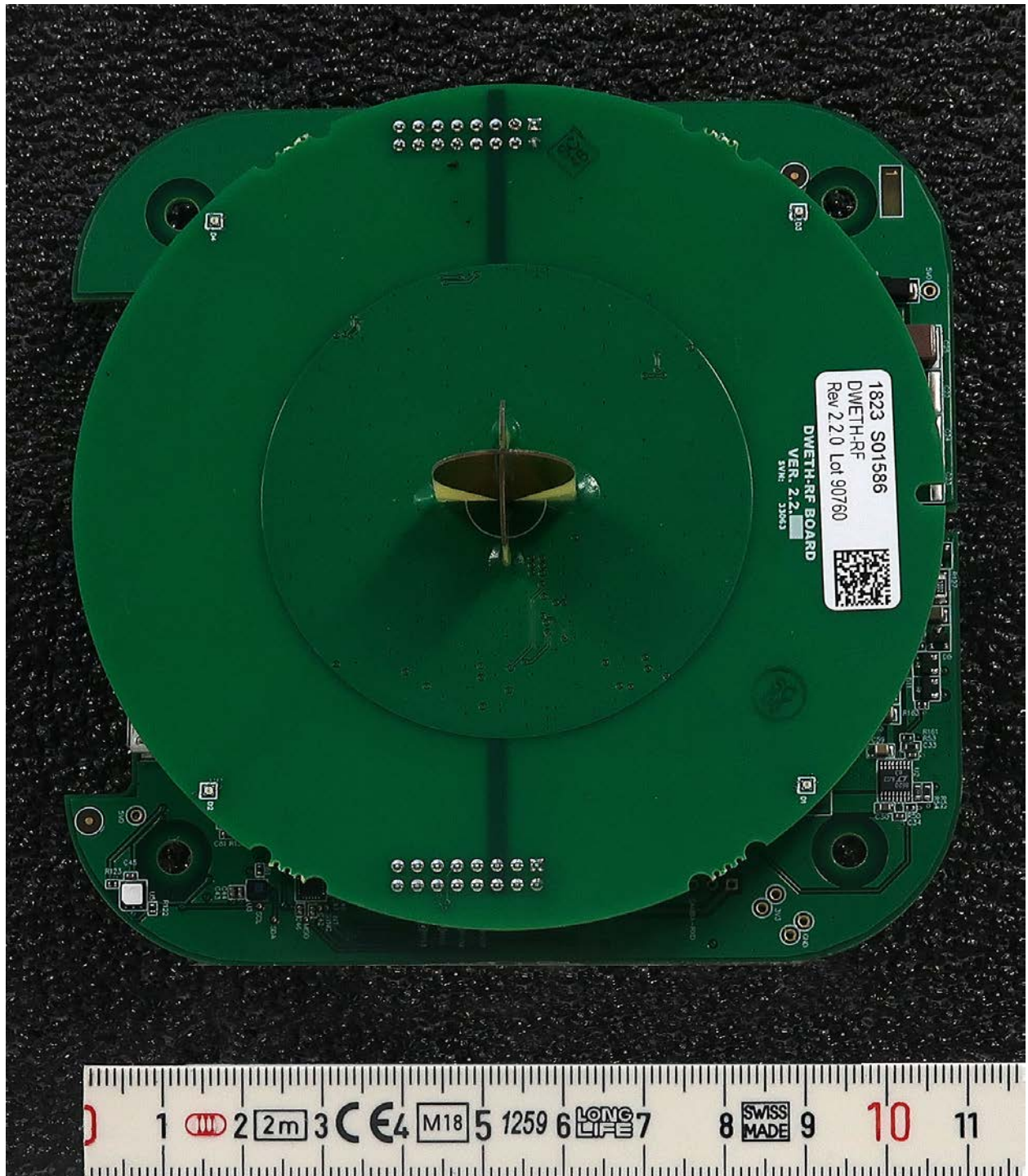
Main Board with Antenna Attached
