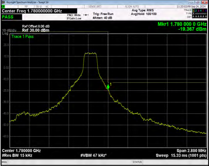
Band66 QPSK BW=1.4MHz Channel=132665 RB Size=6 Position=#0 Extended
