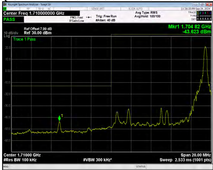
Band66 QPSK BW=10MHz Channel=132022 RB Size=50 Position=#0 Extended
