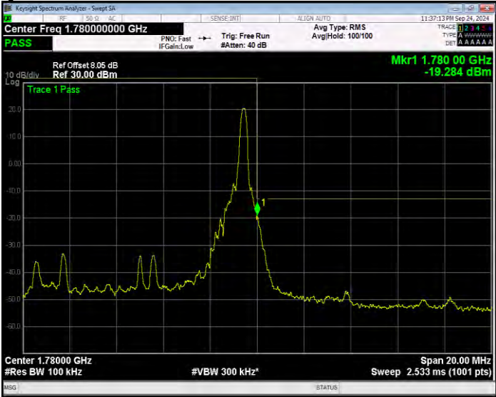
Band66 QPSK BW=10MHz Channel=132622 RB Size=50 Position=#0 Extended
