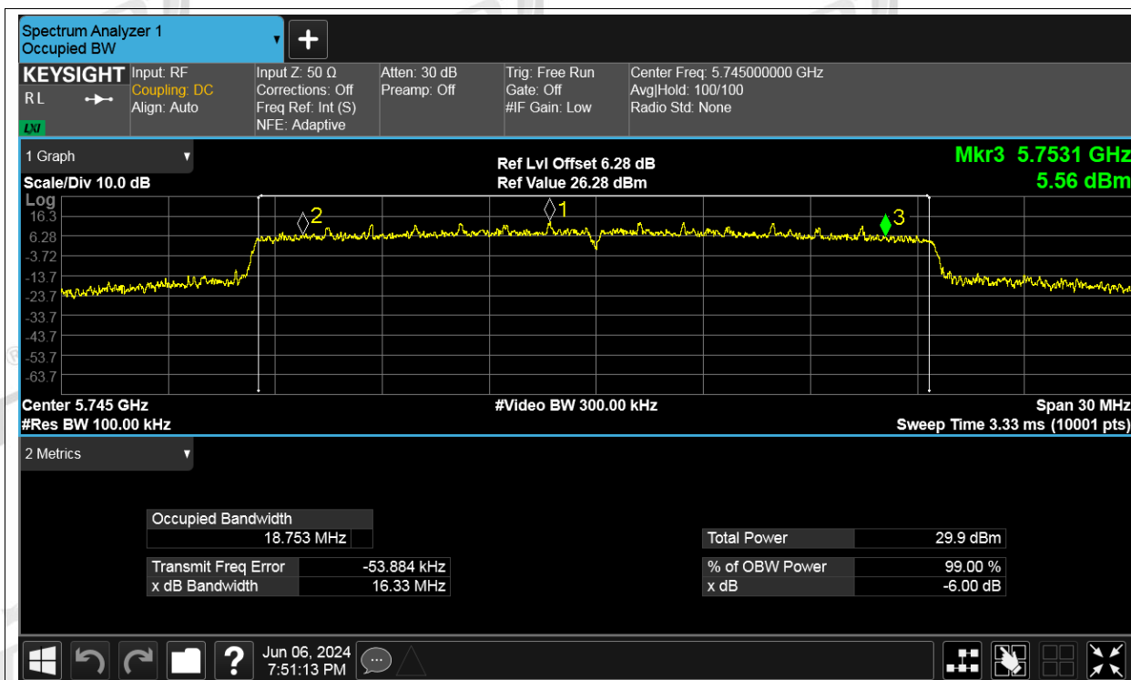
-6dB Bandwidth NVNT be20 5745MHz Ant3
