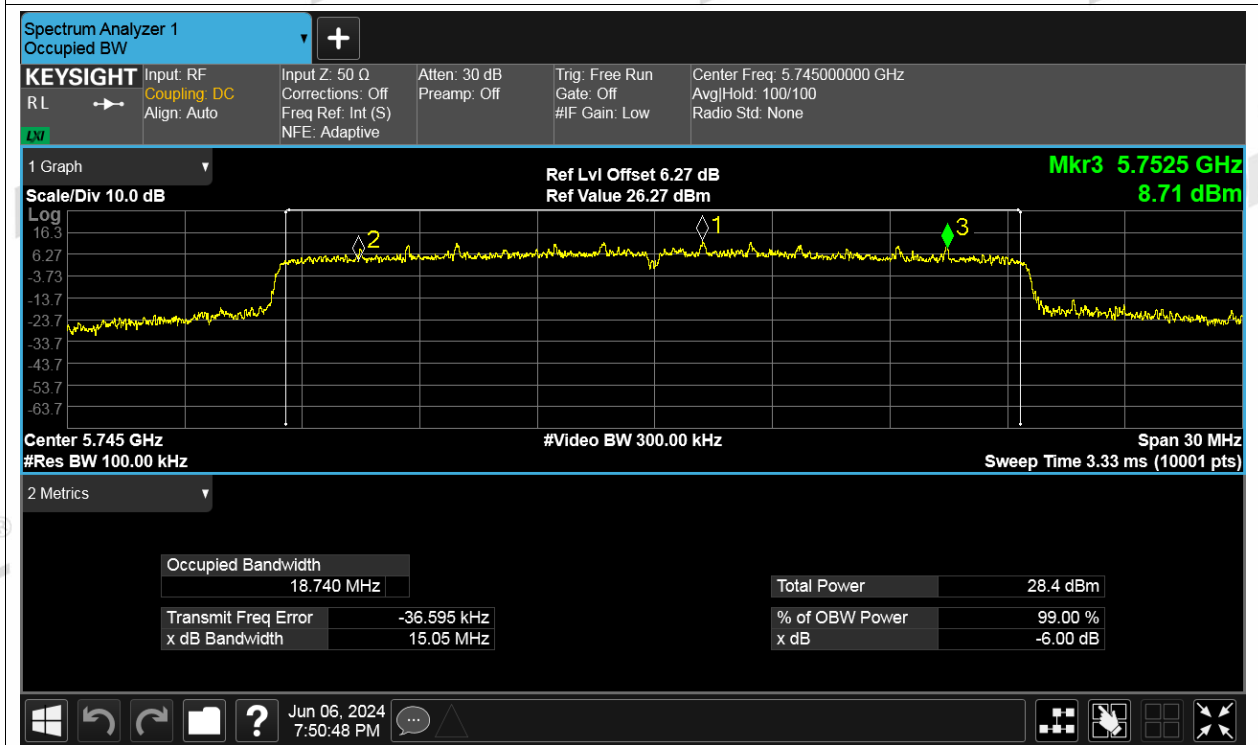
-6dB Bandwidth NVNT be20 5745MHz Ant2
