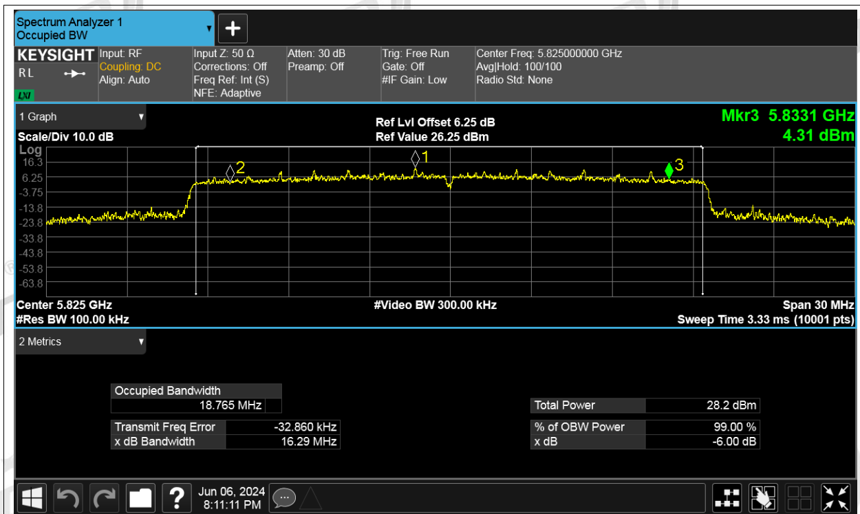
-6dB Bandwidth NVNT be20 5825MHz Ant3
