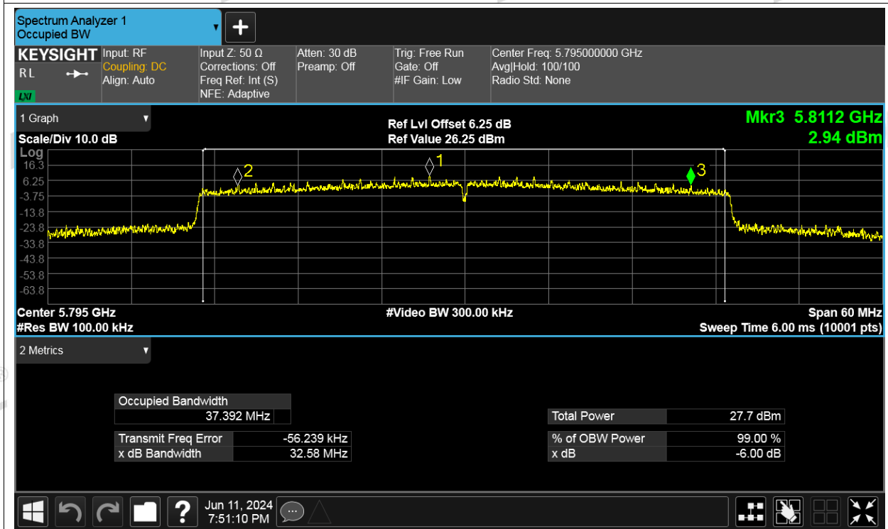
-6dB Bandwidth NVNT be40 5795MHz Ant2
