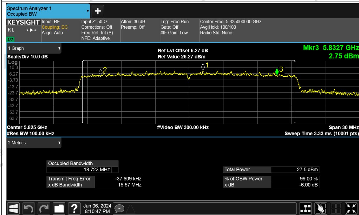
-6dB Bandwidth NVNT be20 5825MHz Ant2
