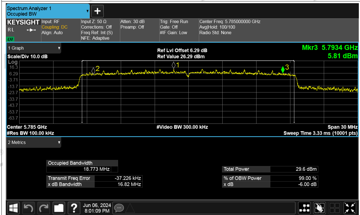
-6dB Bandwidth NVNT be20 5785MHz Ant3
