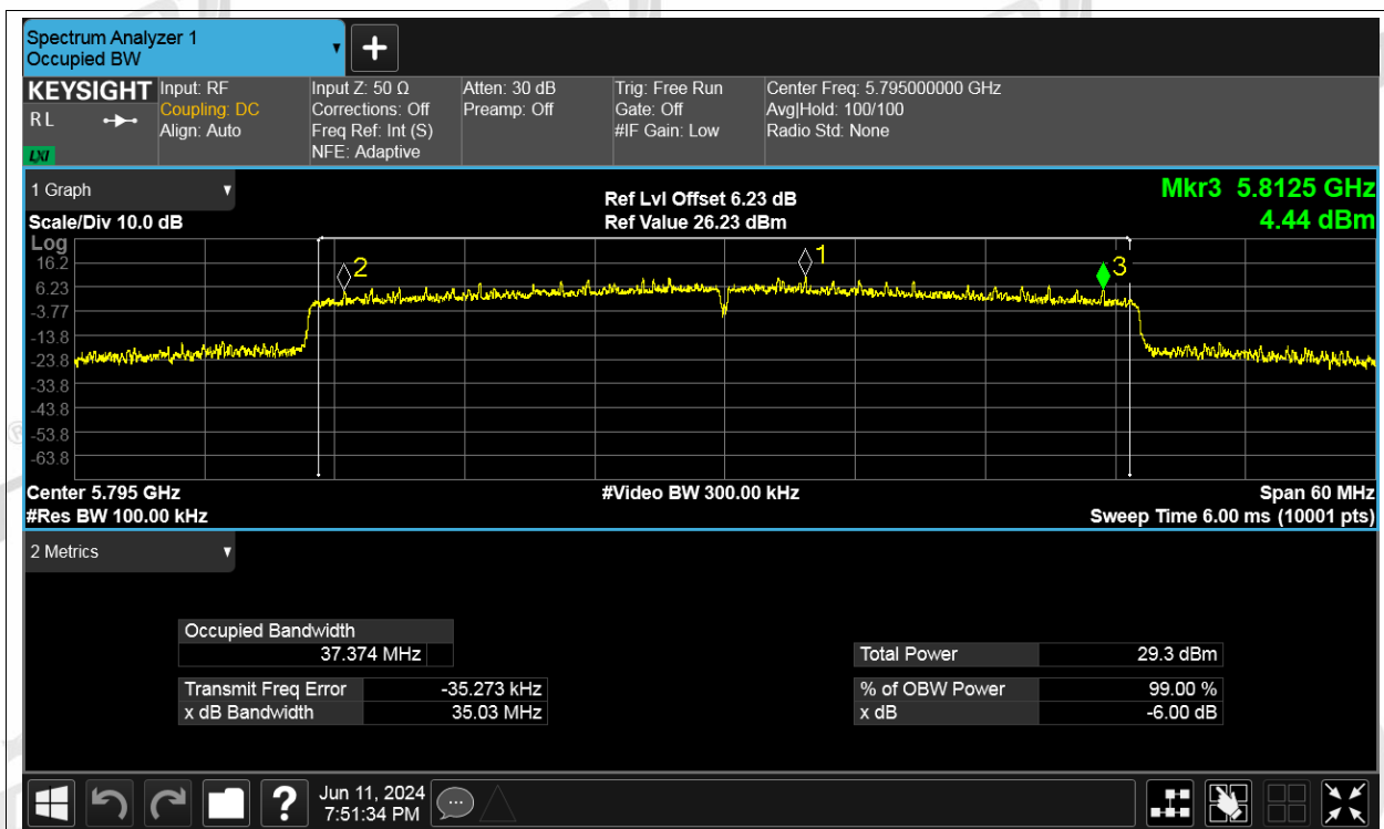
-6dB Bandwidth NVNT be40 5795MHz Ant3
