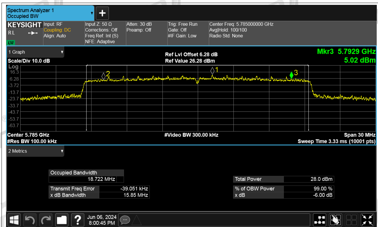
-6dB Bandwidth NVNT be20 5785MHz Ant2
