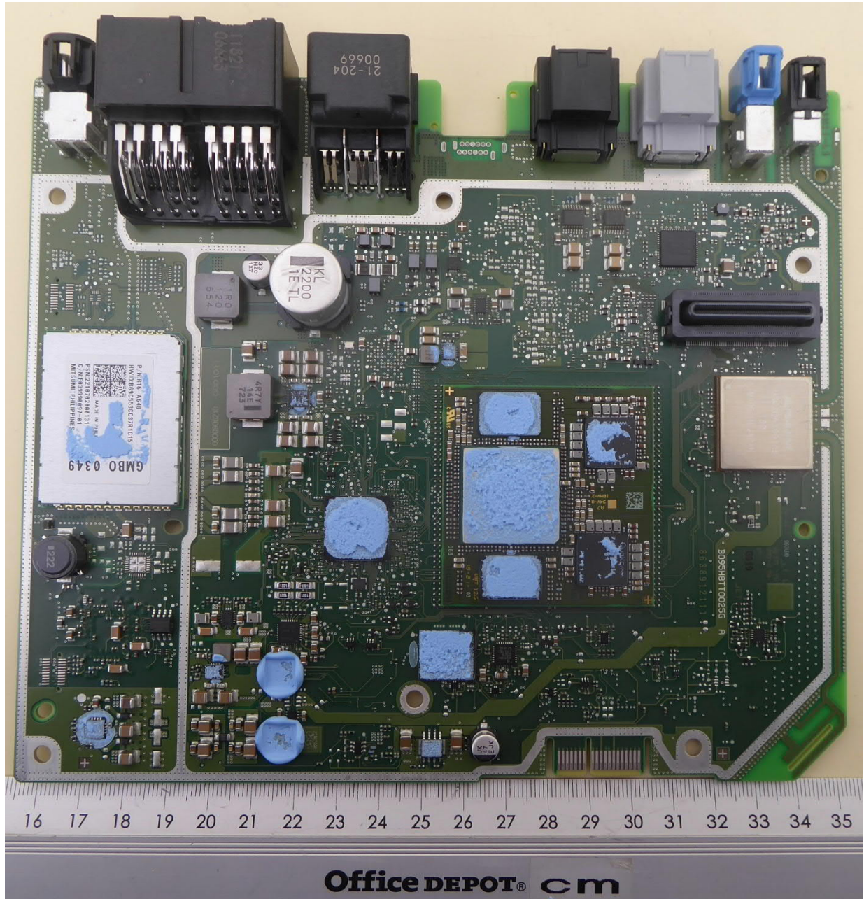
Main PCB – top view
