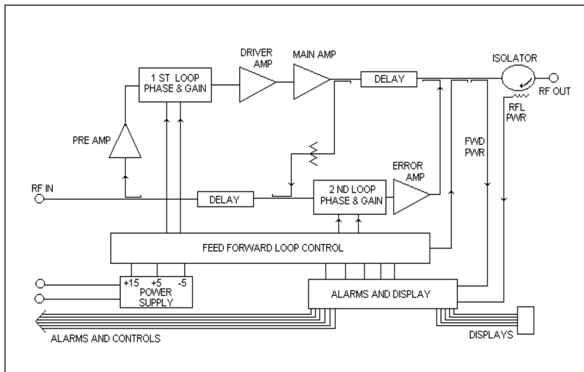
Figure 4-2. G3X-800 Series (NTL107AA) Power Amplifier Module Functional Block Diagram
