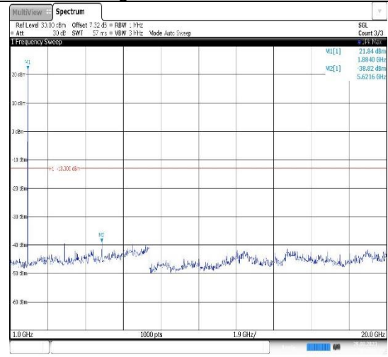
Band2-10MHz-16QAM-18900-1RB#0- Range2:1000~20000MHz
