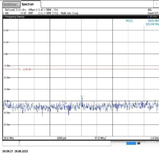
Band2-3MHz-16QAM-19185-1RB#0- Range1:30~1000MHz
