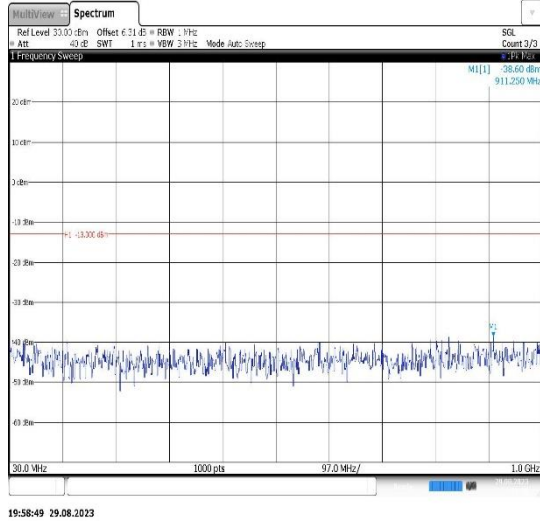
Band2-3MHz-16QAM-18900-1RB#0- Range1:30~1000MHz
