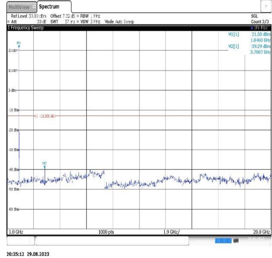
Band2-10MHz-QPSK-18900-1RB#0- Range2:1000~20000MHz
