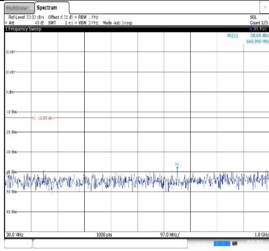
Band2-10MHz-16QAM-18650-1RB#0- Range1:30~1000MHz
