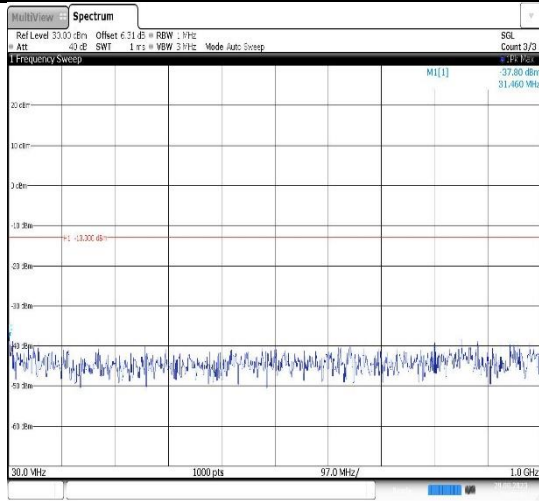
Band2-5MHz-QPSK-18625-1RB#0- Range1:30~1000MHz
