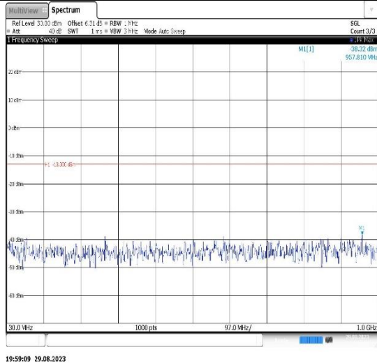
Band2-3MHz-QPSK-19185-1RB#0- Range1:30~1000MHz
