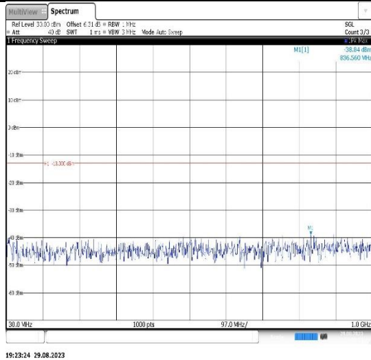
Band2-3MHz-QPSK-18615-1RB#0- Range1:30~1000MHz
