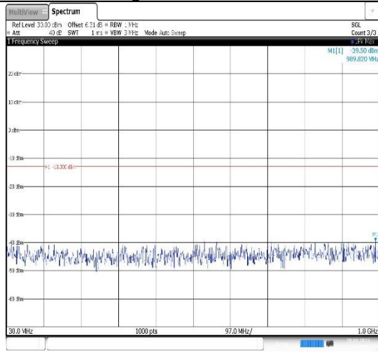
Band2-5MHz-16QAM-18900-1RB#0- Range1:30~1000MHz
