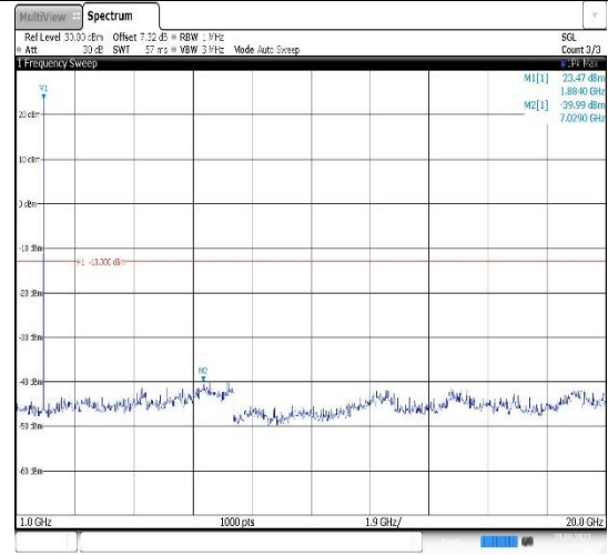
Band2-1.4MHz-16QAM-18900-1RB#0- Range2:1000~20000MHz
