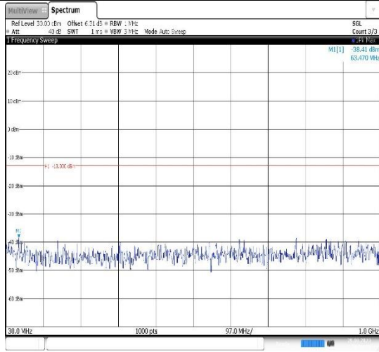
Band2-5MHz-QPSK-18900-1RB#0- Range1:30~1000MHz
