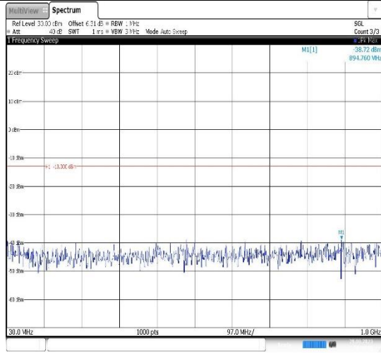
Band2-20MHz-QPSK-18900-1RB#0- Range1:30~1000MHz
