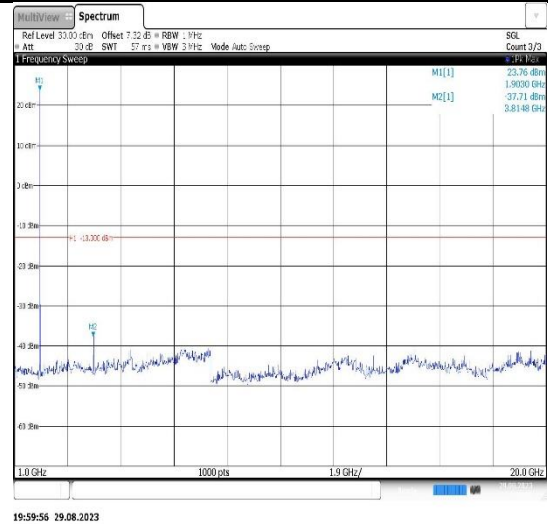
Band2-3MHz-16QAM-18615-1RB#0- Range2:1000~20000MHz
