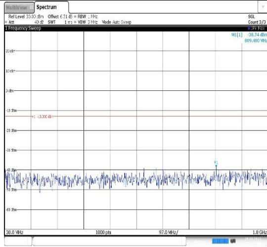
Band2-1.4MHz-16QAM-18900-1RB#0- Range1:30~1000MHz
