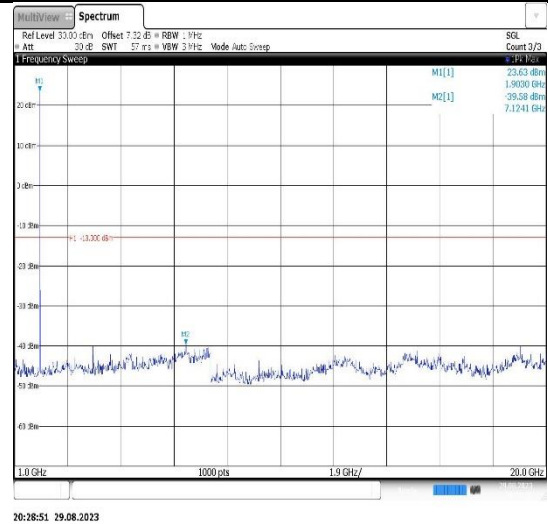
Band2-10MHz-QPSK-18650-1RB#0- Range2:1000~20000MHz
