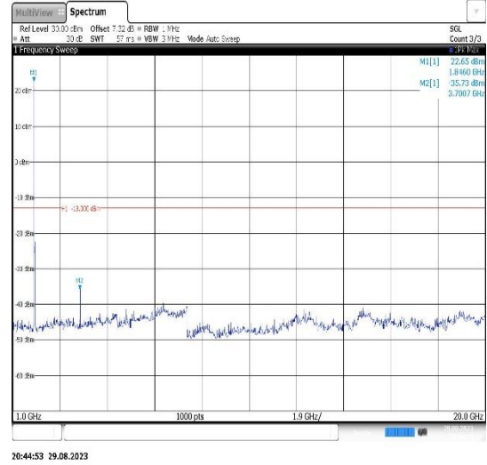
Band2-15MHz-QPSK-18900-1RB#0- Range2:1000~20000MHz
