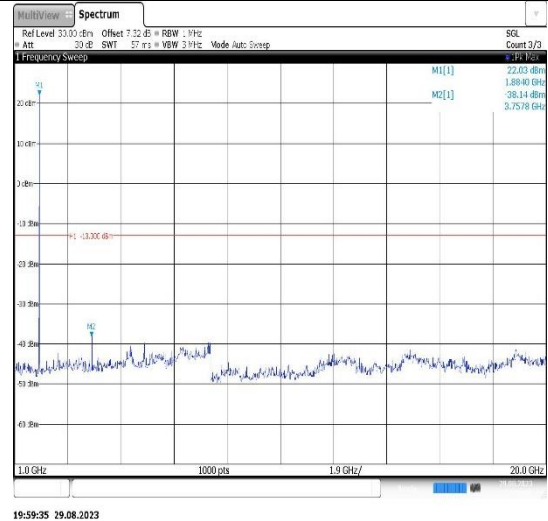
Band2-3MHz-16QAM-19185-1RB#0- Range2:1000~20000MHz
