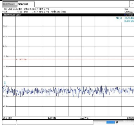
Band2-1.4MHz-16QAM-18607-1RB#0- Range1:30~1000MHz
