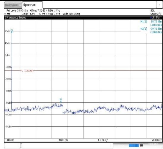
Band2-5MHz-16QAM-18900-1RB#0- Range2:1000~20000MHz
