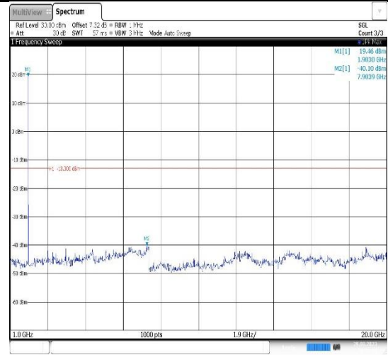
Band2-5MHz-16QAM-18625-1RB#0- Range2:1000~20000MHz
