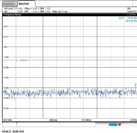
Band2-15MHz-QPSK-19125-1RB#0- Range1:30~1000MHz
