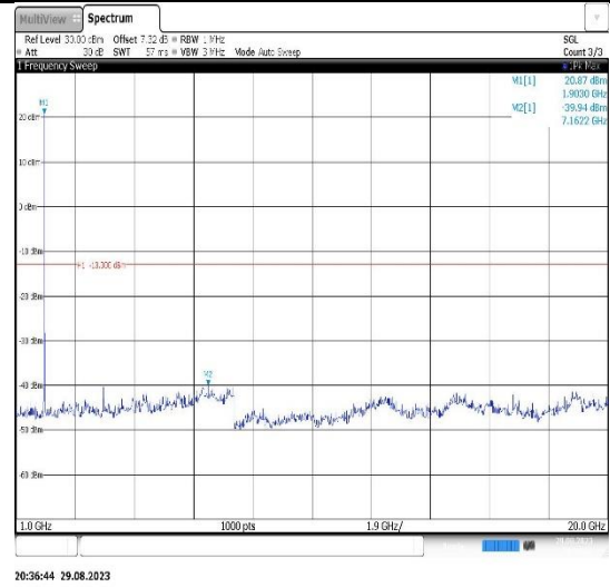
Band2-15MHz-QPSK-18675-1RB#0- Range2:1000~20000MHz
