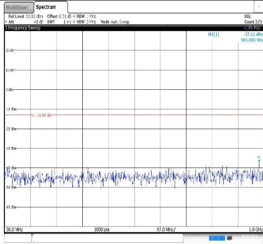
Band2-20MHz-16QAM-18900-1RB#0- Range1:30~1000MHz
