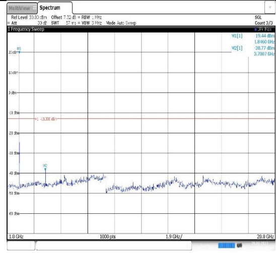
Band2-10MHz-16QAM-18650-1RB#0- Range2:1000~20000MHz
