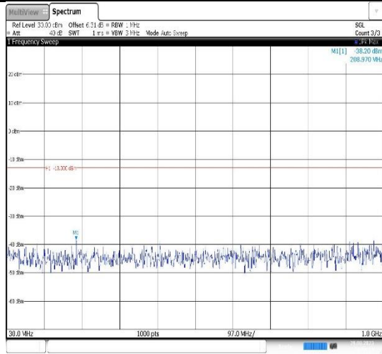
Band2-15MHz-16QAM-18675-1RB#0- Range1:30~1000MHz
