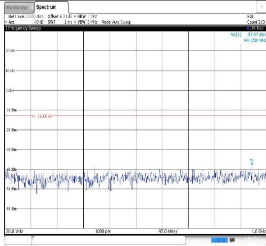
Band2-15MHz-16QAM-19125-1RB#0- Range1:30~1000MHz
