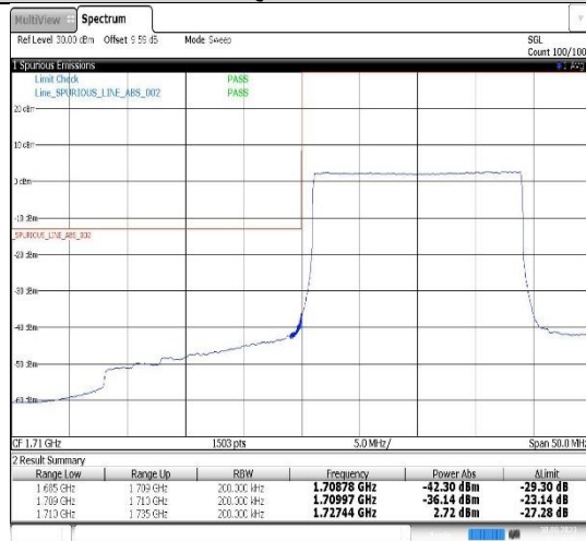
Band66-20MHz-QPSK-132072-100RB#0
