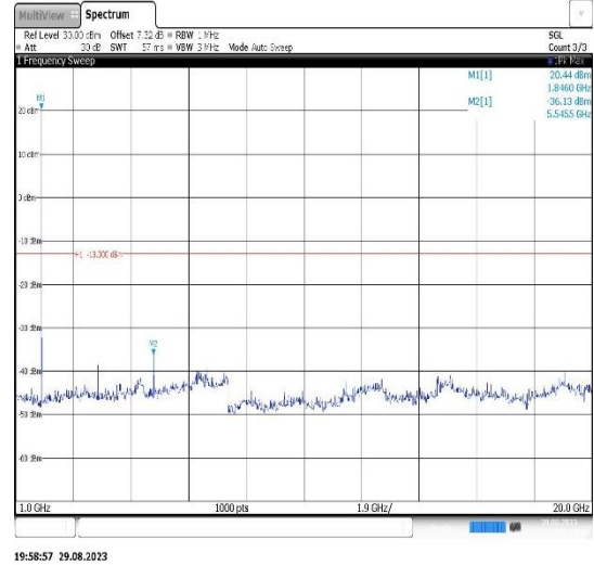
Band2-3MHz-16QAM-18900-1RB#0- Range2:1000~20000MHz
