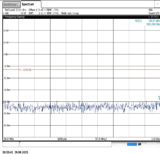
Band2-10MHz-QPSK-19150-1RB#0- Range1:30~1000MHz
