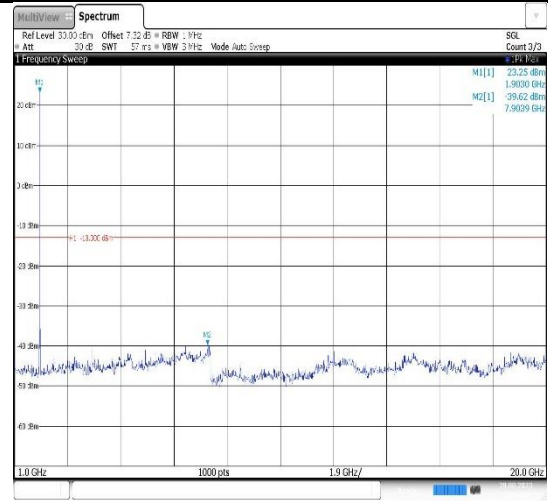
Band2-15MHz-16QAM-18675-1RB#0- Range2:1000~20000MHz
