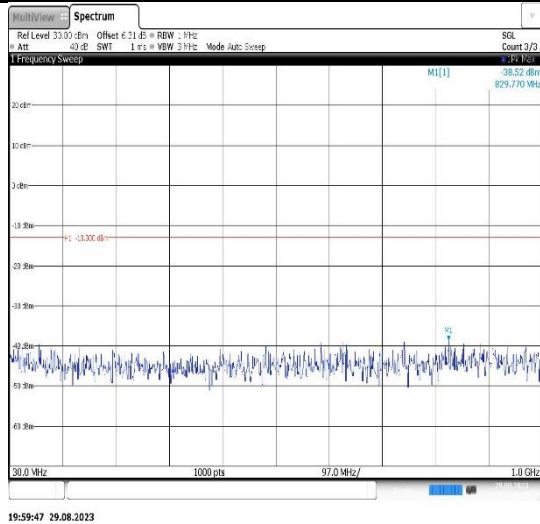
Band2-3MHz-16QAM-18615-1RB#0- Range1:30~1000MHz
