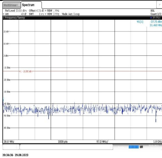
Band2-15MHz-QPSK-18675-1RB#0- Range1:30~1000MHz
