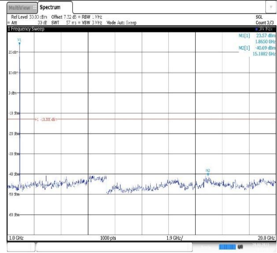
Band2-15MHz-16QAM-19125-1RB#0- Range2:1000~20000MHz
