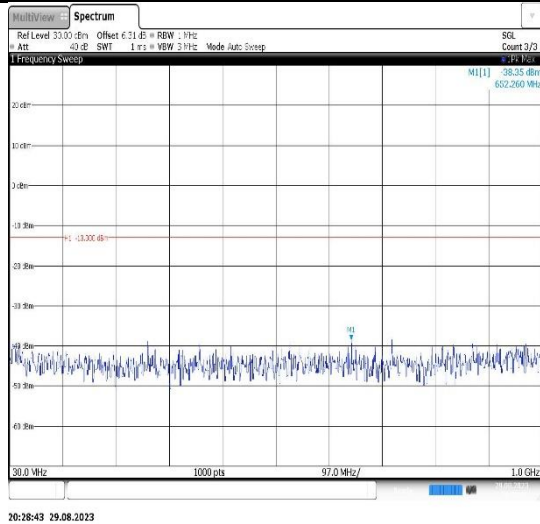
Band2-10MHz-QPSK-18650-1RB#0- Range1:30~1000MHz
