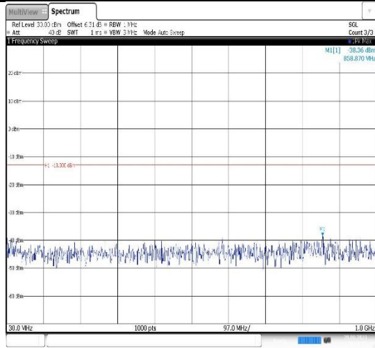
Band2-5MHz-16QAM-18625-1RB#0- Range1:30~1000MHz
