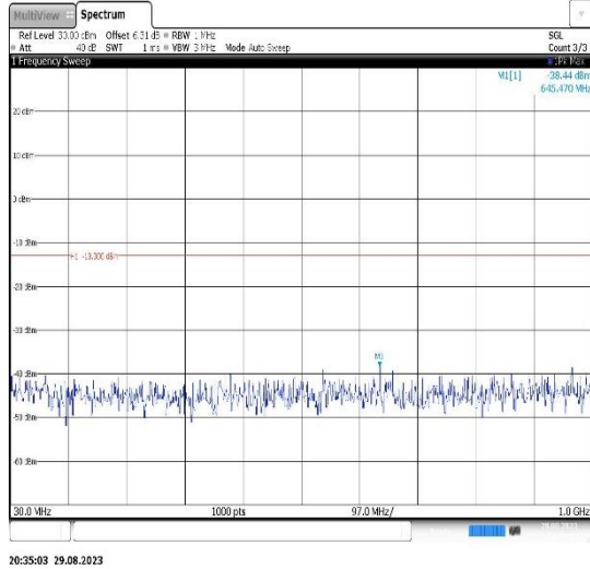
Band2-10MHz-QPSK-18900-1RB#0- Range1:30~1000MHz
