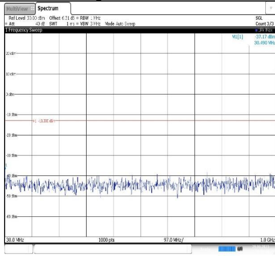
Band2-10MHz-16QAM-18900-1RB#0- Range1:30~1000MHz
