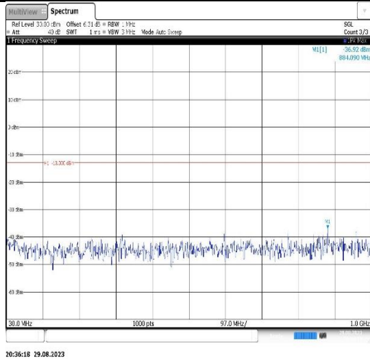
Band2-10MHz-16QAM-18650-1RB#0- Range1:30~1000MHz
