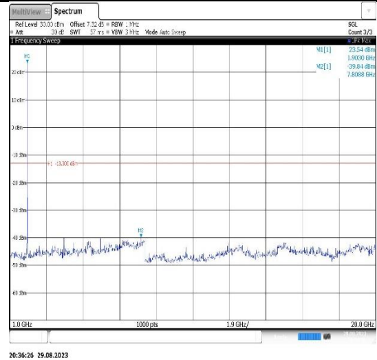
Band2-10MHz-16QAM-18650-1RB#0- Range2:1000~20000MHz
