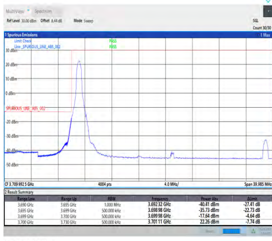
1-N78-3700-3800-PC1-30-30-L-1-DFT-PI2BPSK-Edge_1_RB_Left-1@0-Ant1-1--PASS-see graph
