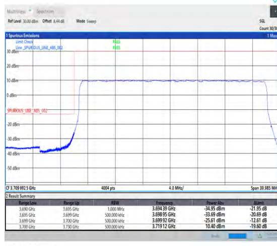
1-N78-3700-3800-PC1-30-30-L-3-DFT-PI2BPSK-Outer_Full-75@0-Ant1-1--PASS-see graph
