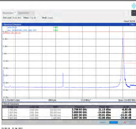
1-N78-3700-3800--30-100-H-5-CP-QPSK-Edge_1RB_ Right-1@272-Ant1-PASS-see graph
