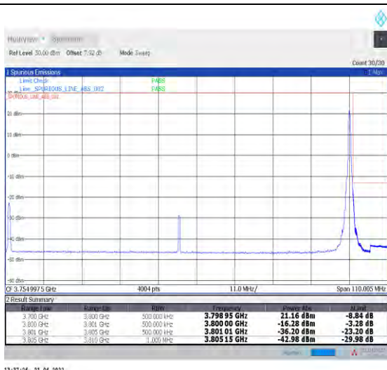
1-N78-3700-3800--30-100-H-2-DFT-PI2BPSK-Edge_1 RB_Right-1@272-Ant1-PASS-see graph
