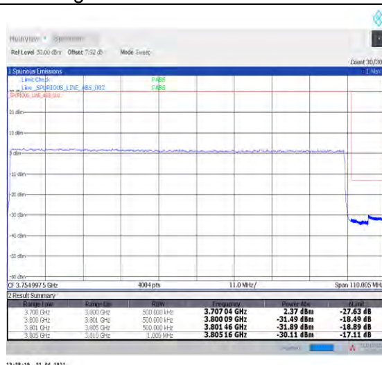
1-N78-3700-3800--30-100-H-3-DFT-PI2BPSK-Out er_Full-270@0-Ant1-PASS-see graph
