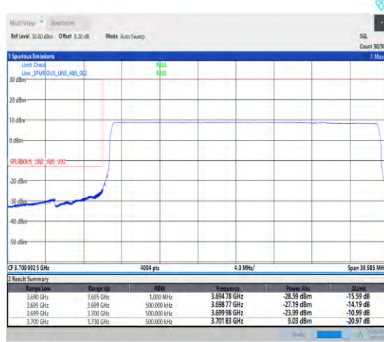
1-N78-3700-3800-PC1-30-30-L-6-CP-QPSK-Outer_Full-78@0-Ant1-1--PASS-see graph
