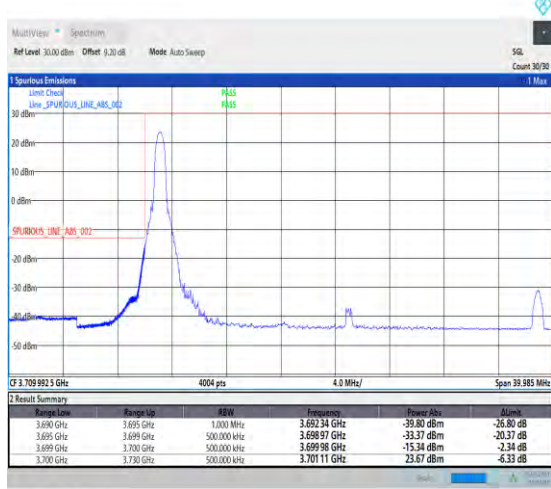
1-N78-3700-3800-PC1-30-30-L-4-CP-QPSK-Edge_1_RB_Left-1@0-Ant1-1--PASS-see graph
