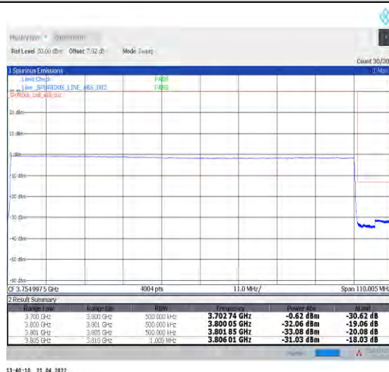
1-N78-3700-3800--30-100-H-6-CP-QPSK-Outer_F ull-273@0-Ant1-PASS-see graph
