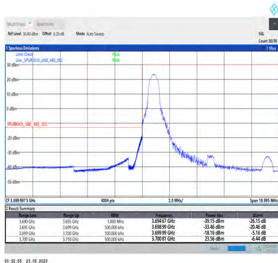
1-N78-3700-3800-PC1-30-10-L-4-CP-QPSK-Edge_1RB_Left-1@0-Ant1-1--PASS-see graph
