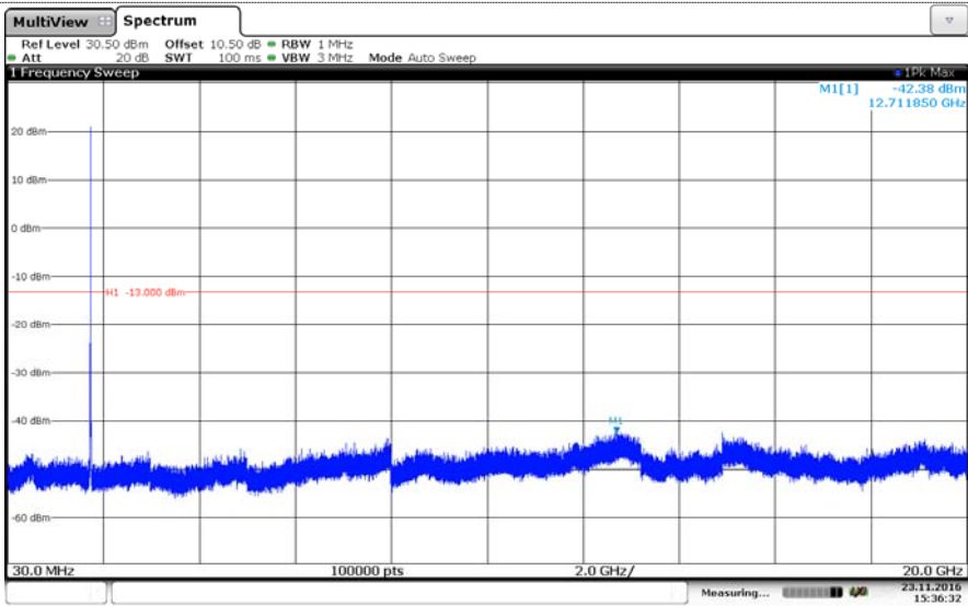
Channel High
