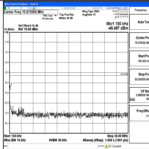
Band66_20MHz_QPSK_132572_1RB#0_0.15~30_0.15~30
