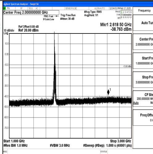
Band66_15MHz_16QAM_132322_1RB#0_1000~3000_1000~3000
