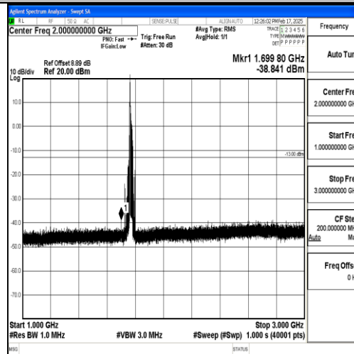
Band66_20MHz_QPSK_132572_1RB#0_1000~3000_1000~3000
