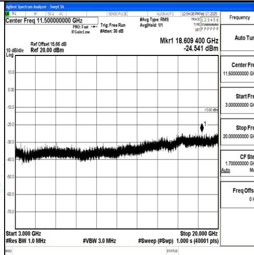
Band66_15MHz_16QAM_132322_1RB#0_3000~20000_3000~20000
