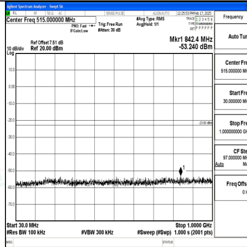
Band66_20MHz_QPSK_132572_1RB#0_30~1000_30~1000
