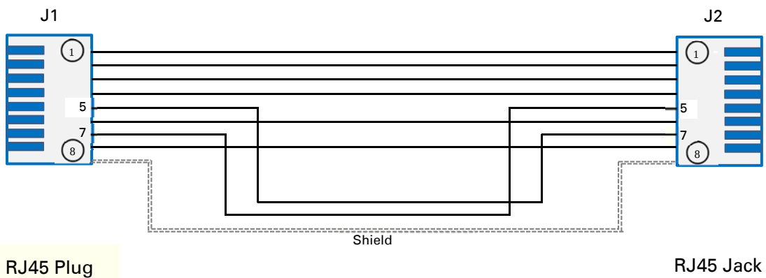
Figure 31 CMM4 power adapter cabling diagram
