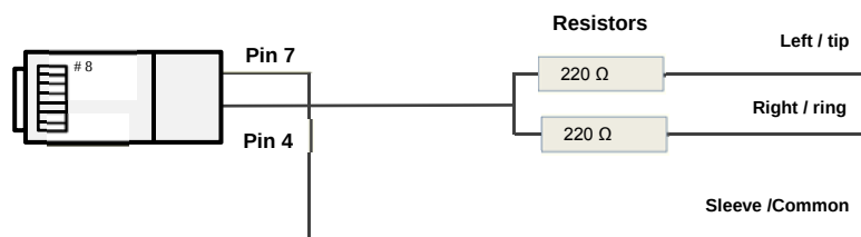
Figure 21 Alignment Tone Cable
