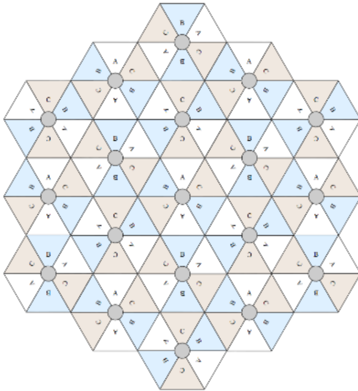
Figure 43 Example layout of 6 Access Point sectors (ABC), 60 degree sectors
