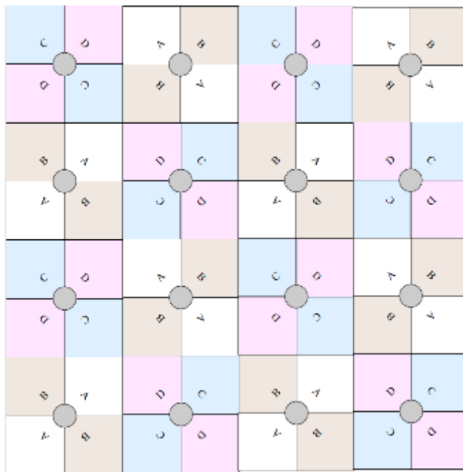
Figure 42 Example layout of 16 Access Point sectors (ABCD), 90 degree sectors
