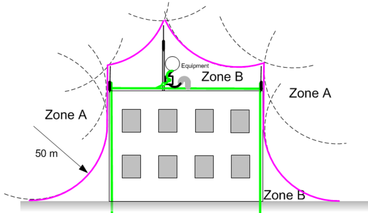
Figure 41 Rolling sphere method to determine the lightning protection zones
