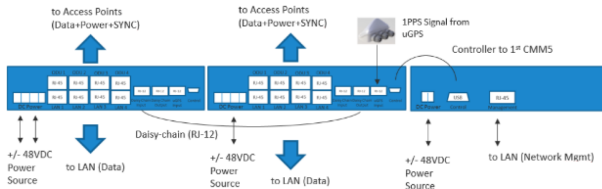
Figure 26 Cluster Management: Scenario 2
