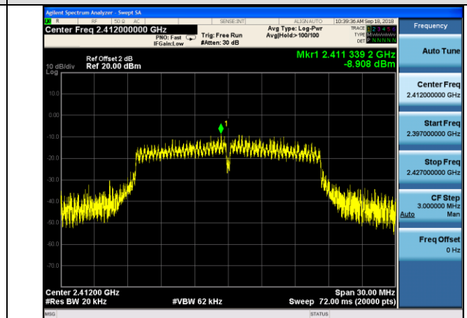
11g-LCH
