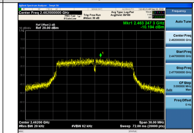
11g-HCH
