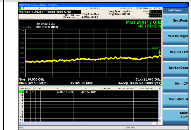
11nHT20-HCH
