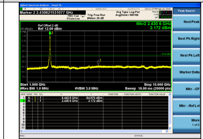
11nHT40-MCH
