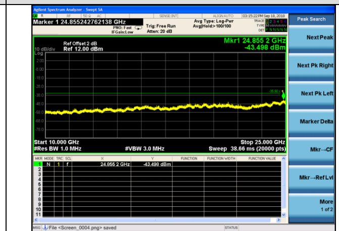
11nHT40-HCH
