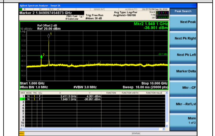
11B-LCH
