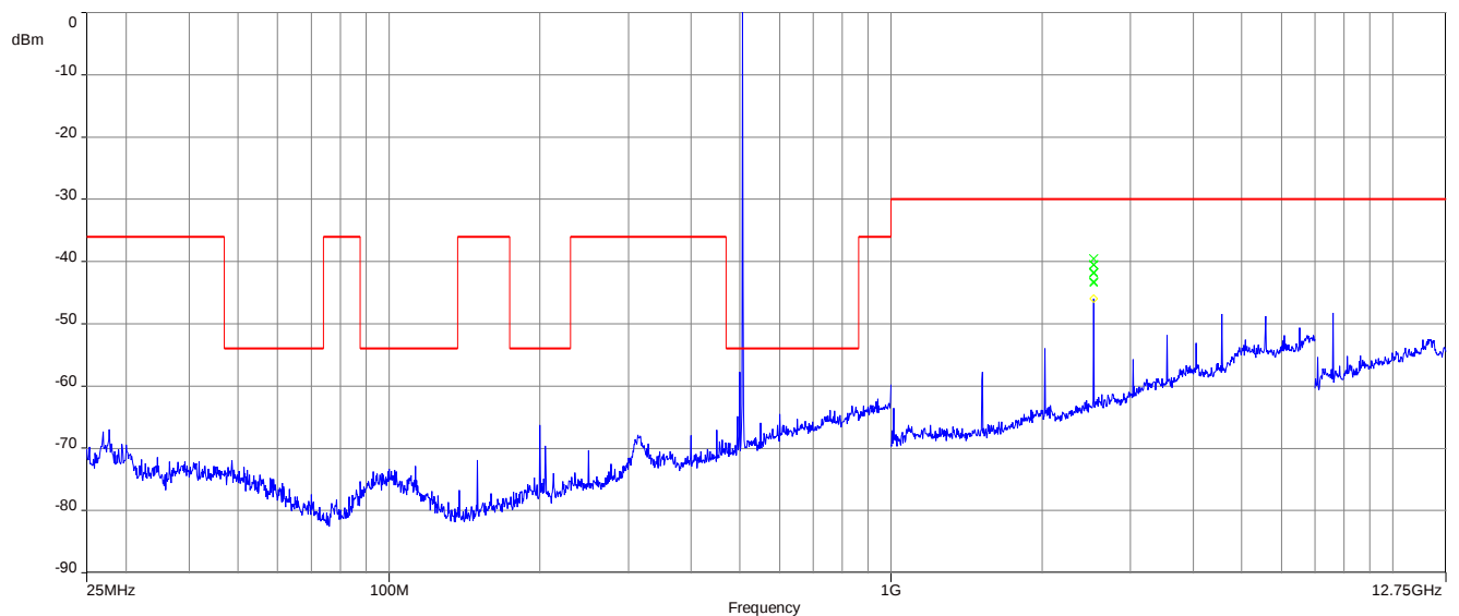
Plot 3: 506.500 MHz, spurious emissions, 25 MHz – 12.75 GHz
