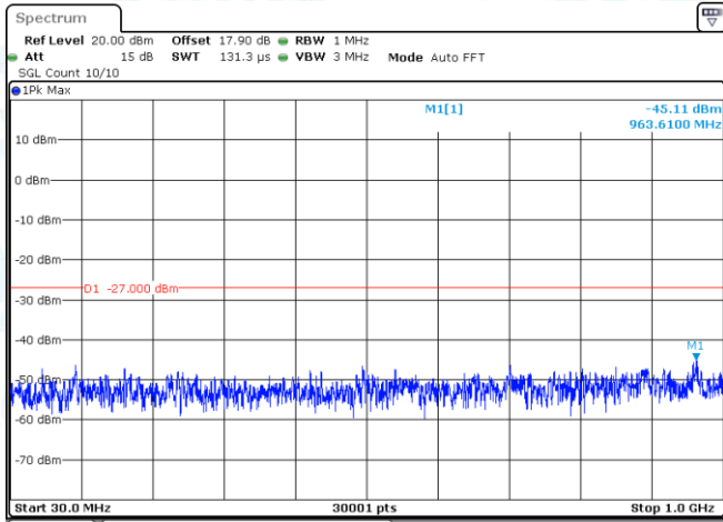
11AC20-CDD-Ant1-5720-30~1000-PASS
