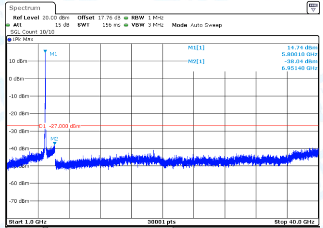
11AC40-CDD-Ant2-5795-1000~40000-PASS
