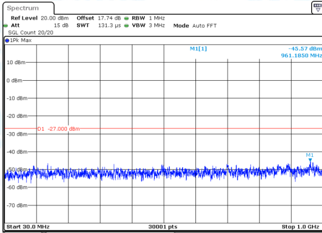
11AC20-CDD-Ant1-5825-30~1000-PASS
