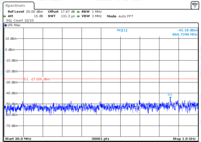
11AC40-CDD-Ant2-5550-30~1000-PASS
