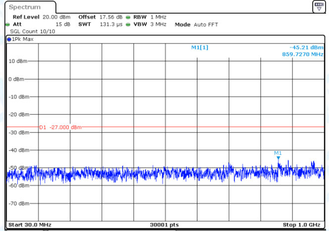
11AC20-CDD-Ant2-5260-30~1000-PASS
