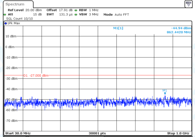
11AC80-CDD-Ant2-5690-30~1000-PASS
