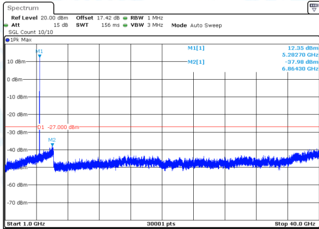
11AC20-CDD-Ant1-5280-1000~40000-PASS
