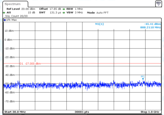
11AC20-CDD-Ant2-5825-30~1000-PASS
