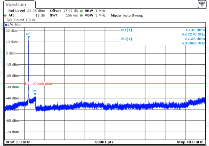
11AC40-CDD-Ant2-5670-1000~40000-PASS
