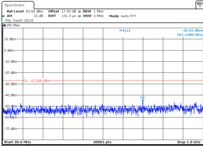
11AC80-CDD-Ant1-5290-30~1000-PASS
