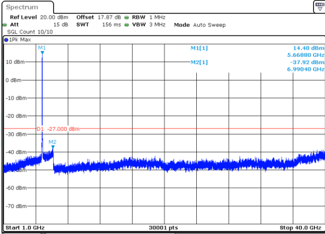
11AC40-CDD-Ant1-5670-1000~40000-PASS
