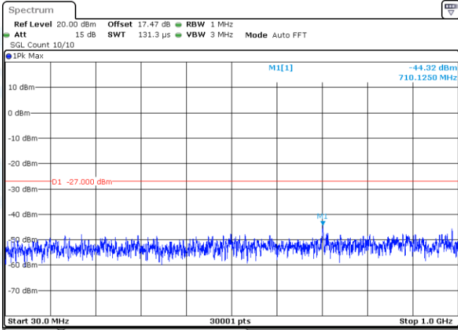
11AC20-CDD-Ant1-5260-30~1000-PASS
