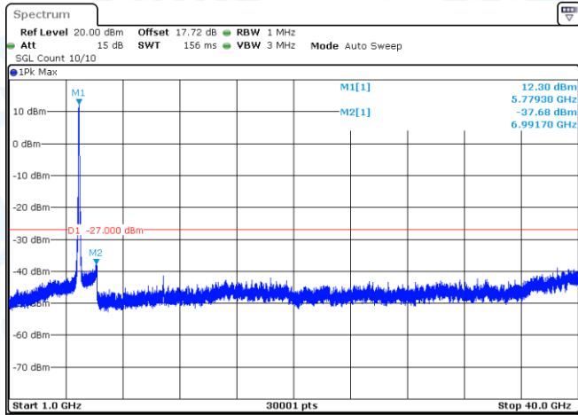
11AC80-CDD-Ant1-5775-1000~40000-PASS
