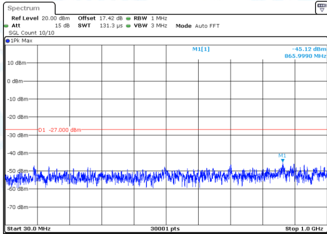
11AC40-CDD-Ant1-5270-30~1000-PASS
