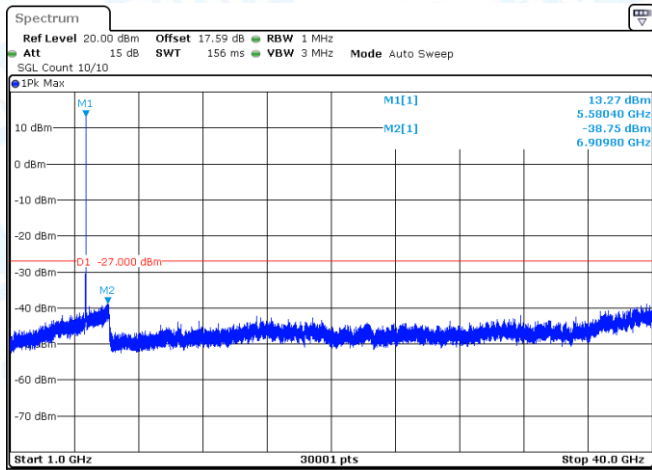
11AC20-CDD-Ant1-5580-1000~40000-PASS
