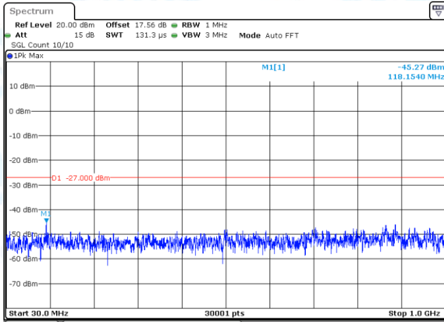
11AC20-CDD-Ant1-5500-30~1000-PASS
