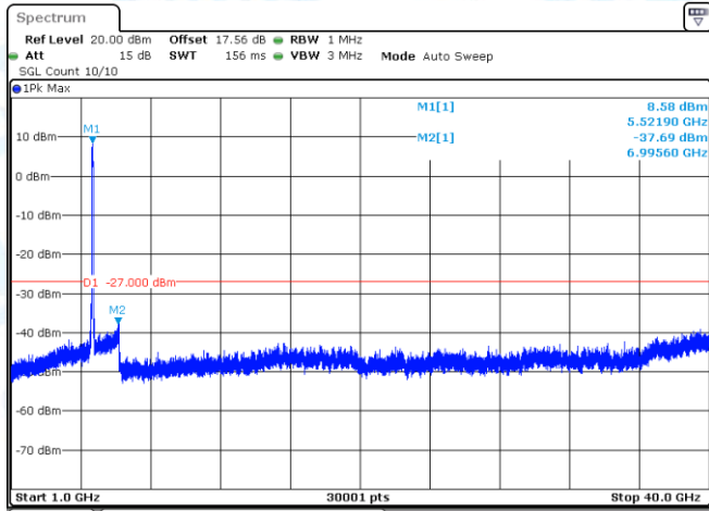
11AC80-CDD-Ant1-5530-1000~40000-PASS
