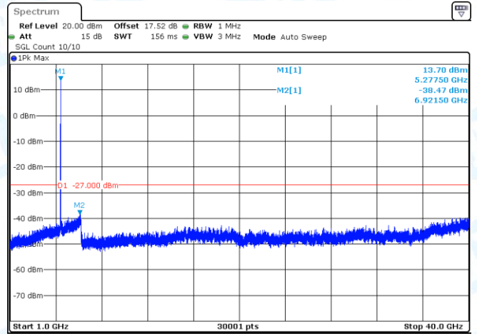
11AC20-CDD-Ant2-5280-1000~40000-PASS
