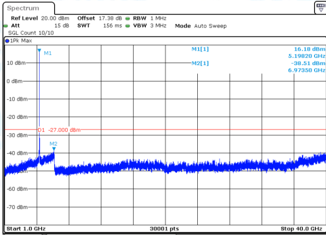
11AC20-CDD-Ant1-5200-1000~40000-PASS
