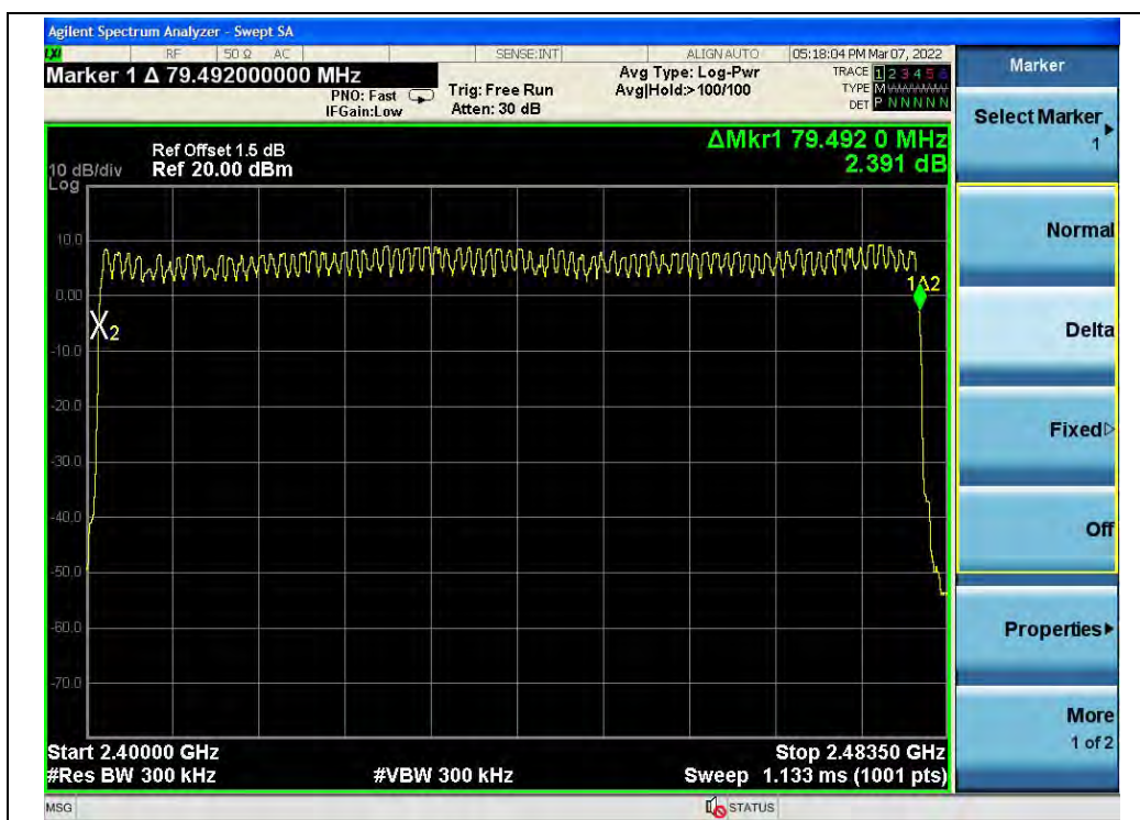
(\pi/4\text{-DQPSK})
