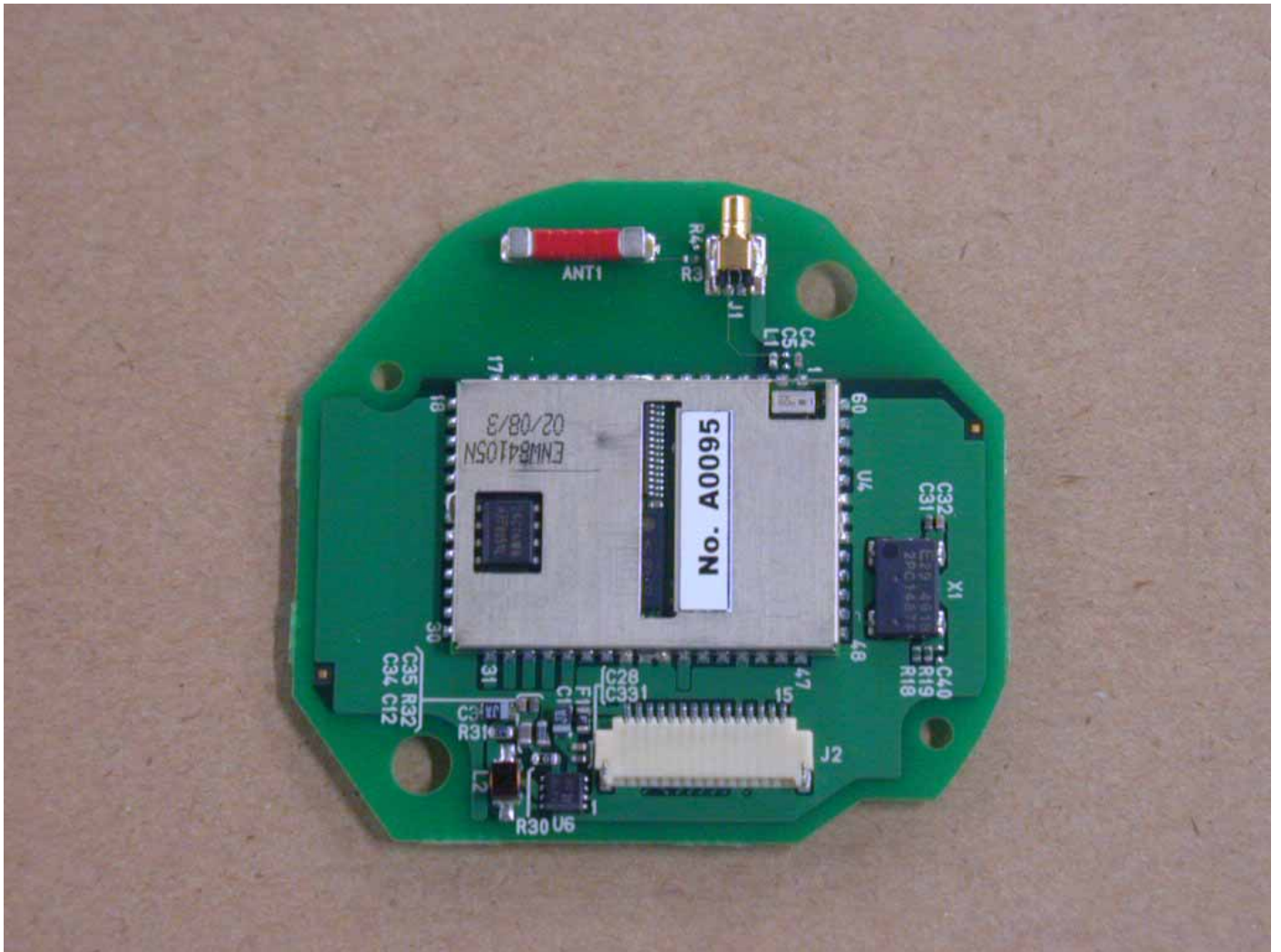
- TX Circuit Board (A side) -
