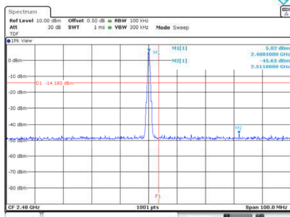
Conducted band-edge / High ch.
