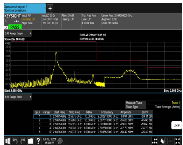
Band41-5MHz-QPSK-40640-25RB#0
