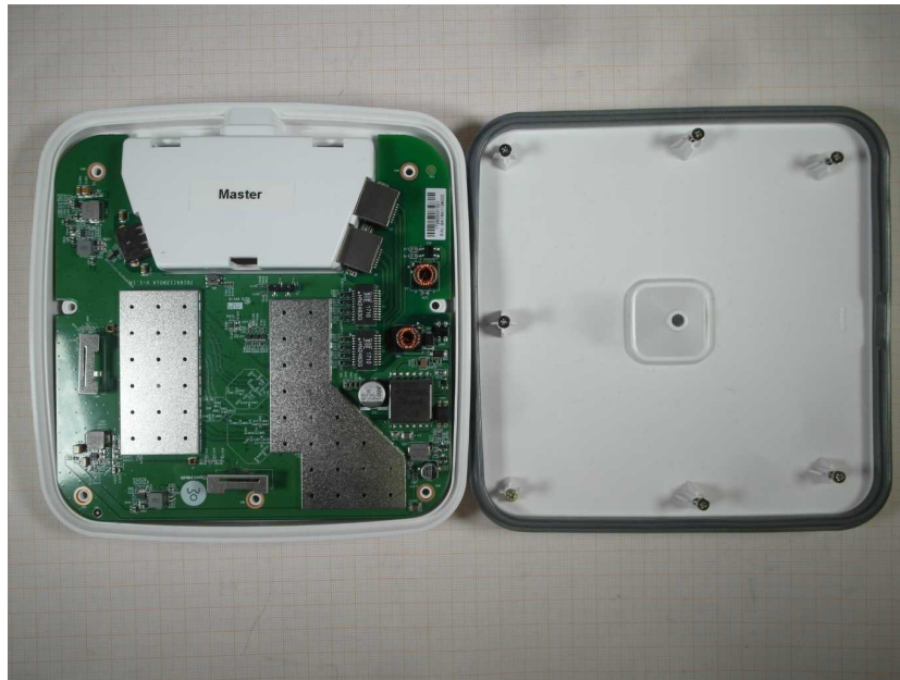
Photo 1 EUT top side (internal view)
