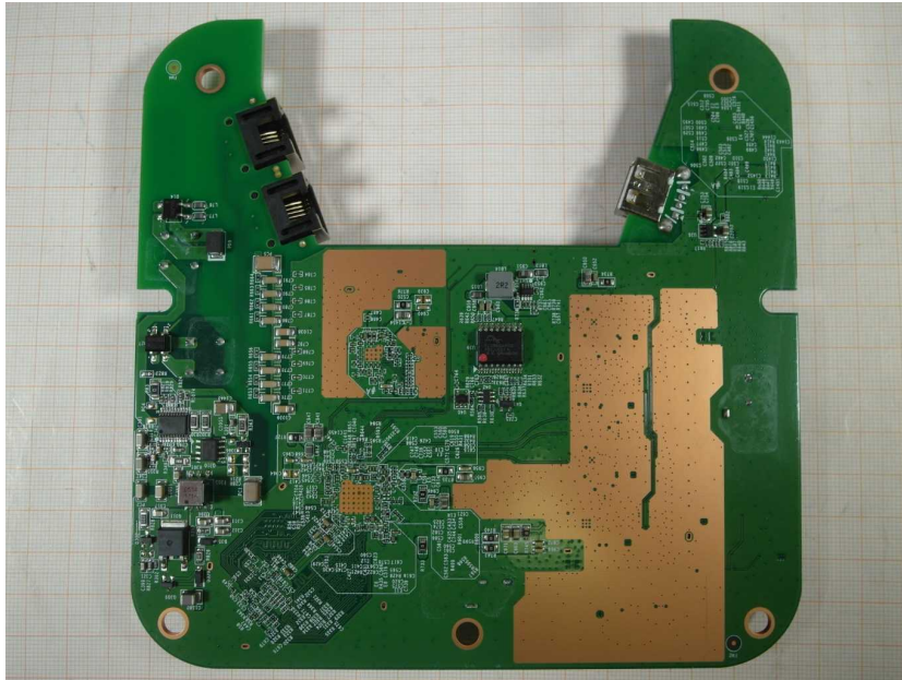
Photo 3 PCB rear view
