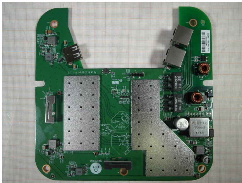
Photo 2 PCB top side
