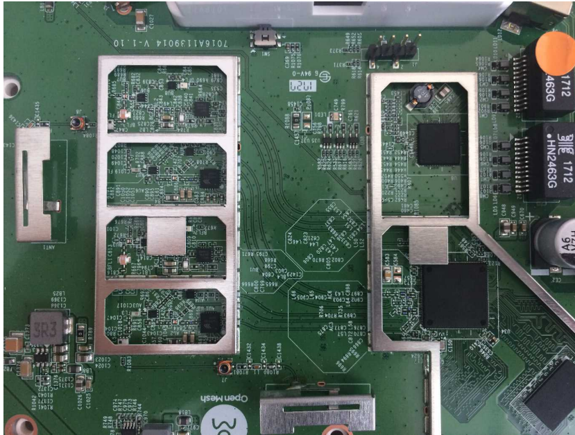
Photo 5 PCB top side (shielding removed)
