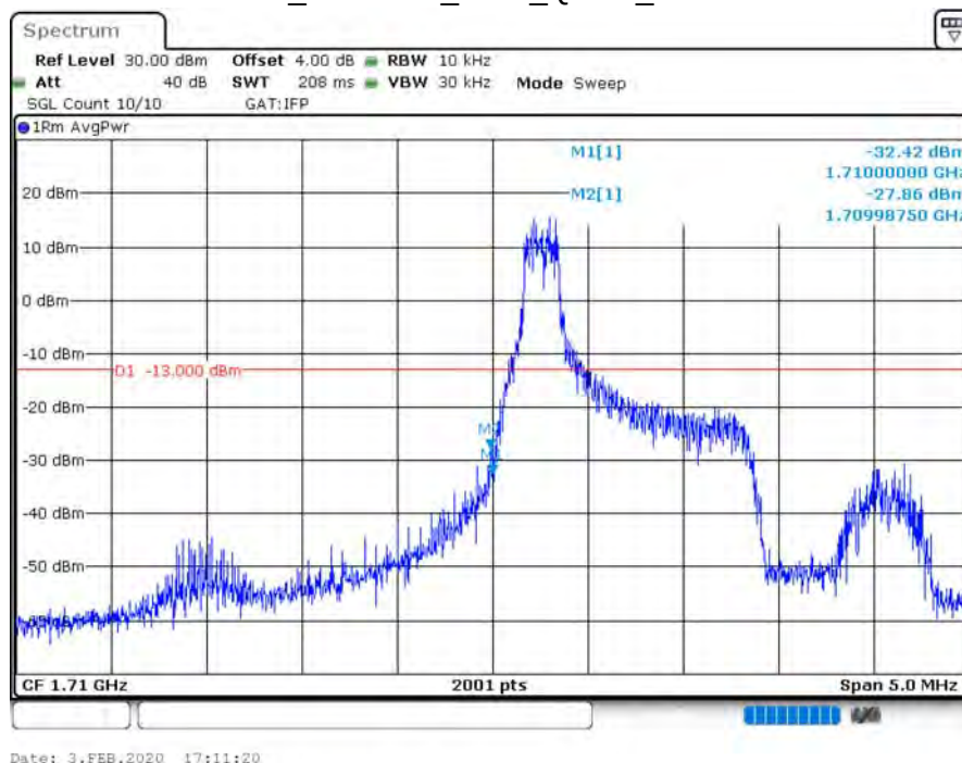
B4_CH19957_1.4M_QPSK_1RB0
