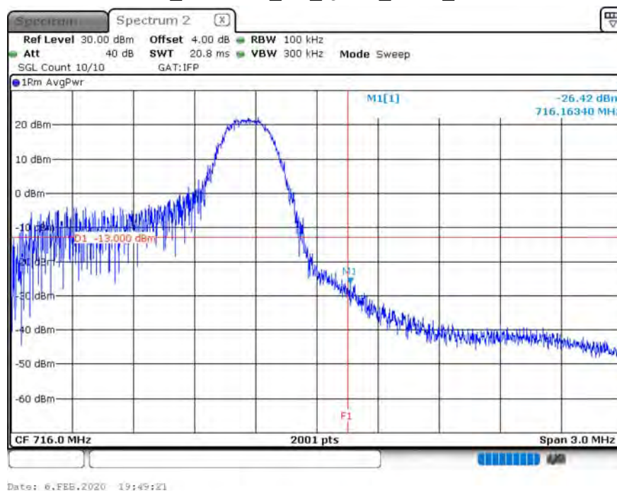
B12_CH23155_5M_QPSK_1RB5_150k
