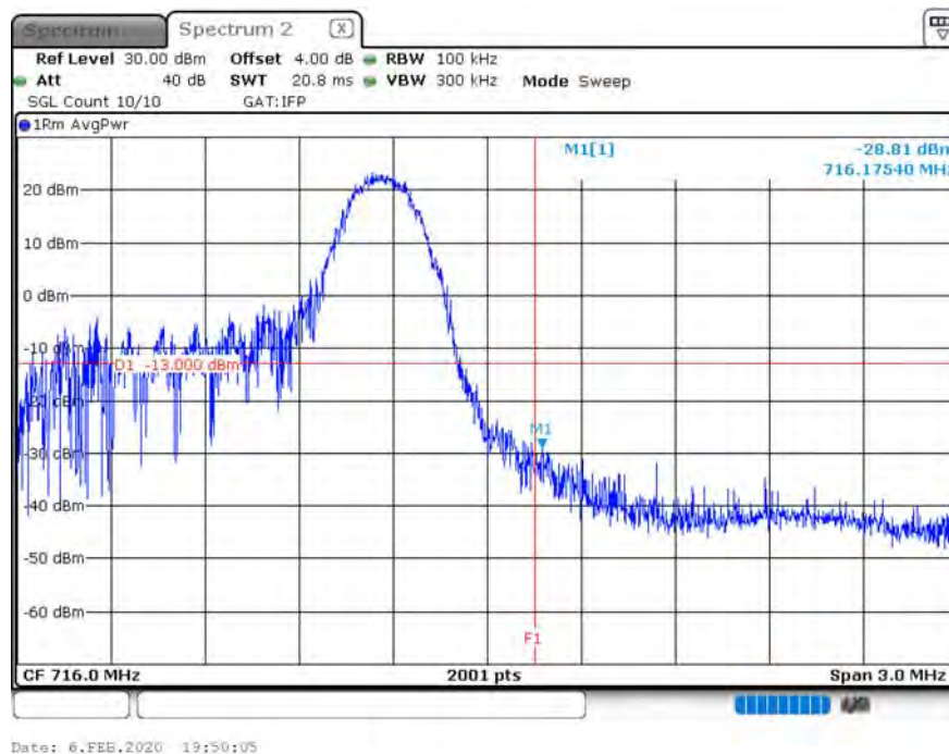
B12_CH23155_5M_16-QAM_1RB5_150k
