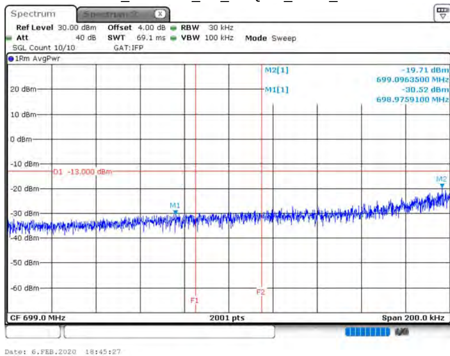
B12_CH23035_5M_16-QAM_1RB0_150k
