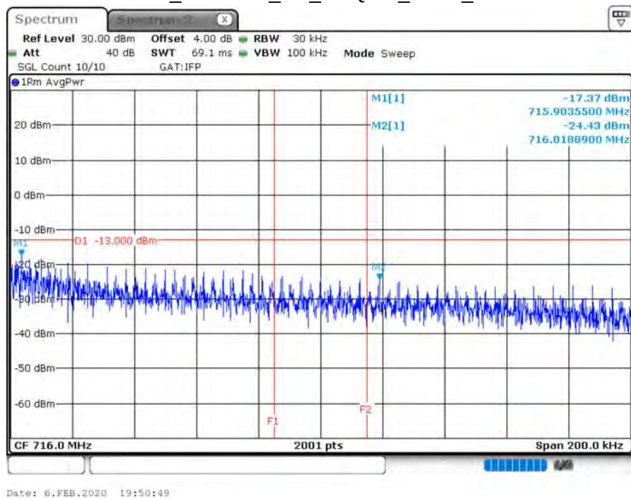
B12_CH23155_5M_16-QAM_1RB5_150k
