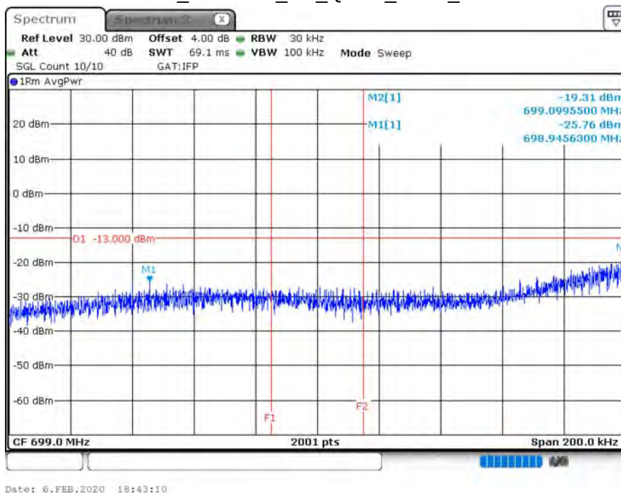
B12_CH23035_5M_QPSK_1RB0_15k
