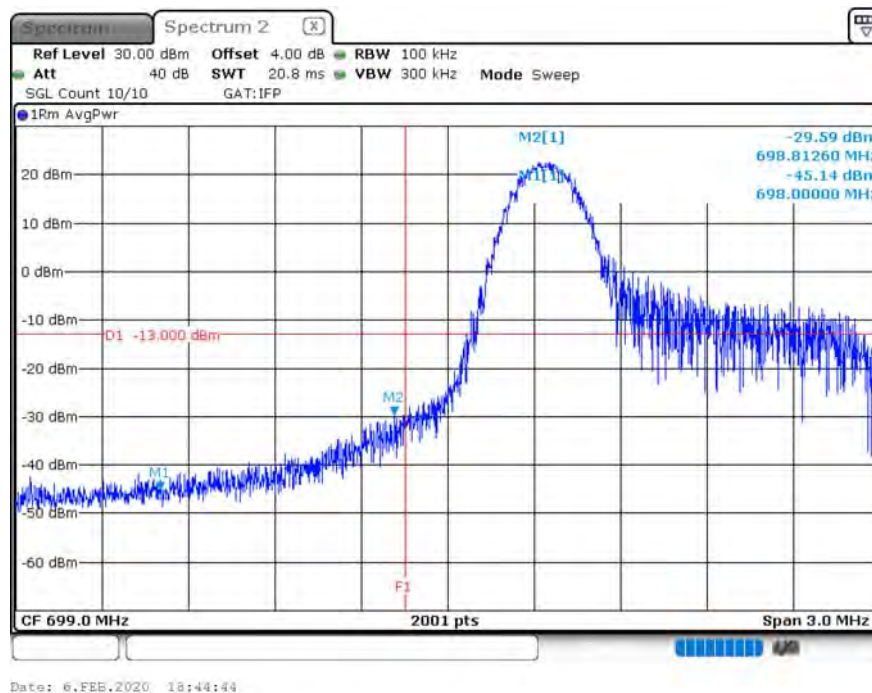
B12_CH23035_5M_16-QAM_1RB0_150k
