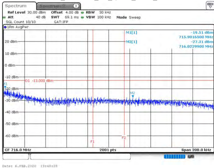
B12_CH23155_5M_QPSK_1RB5_150k
