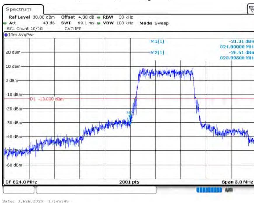
B5_CH20407_1.4M_QPSK_6RB0
