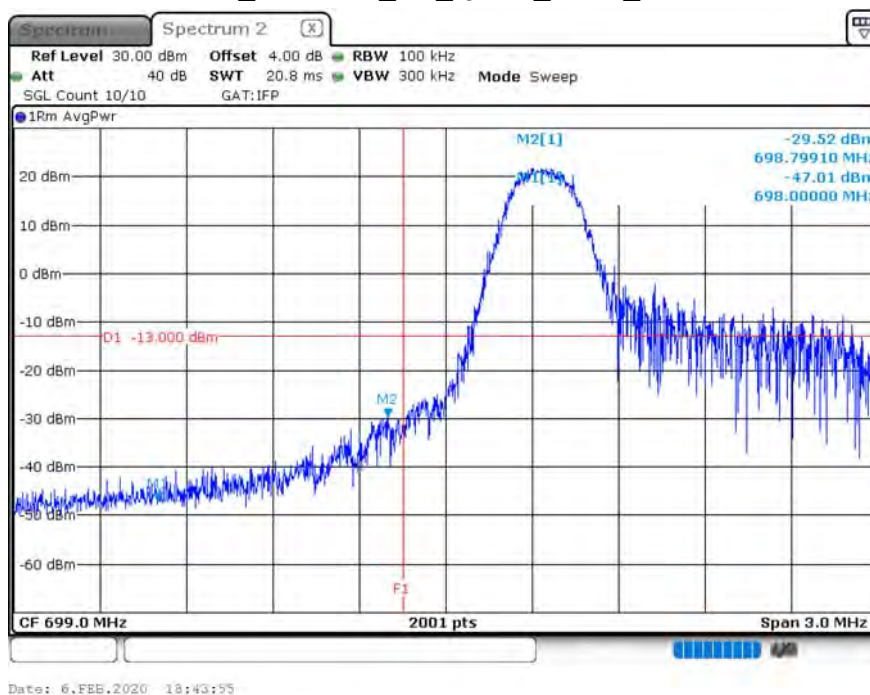
B12_CH23035_5M_QPSK_1RB0_150k
