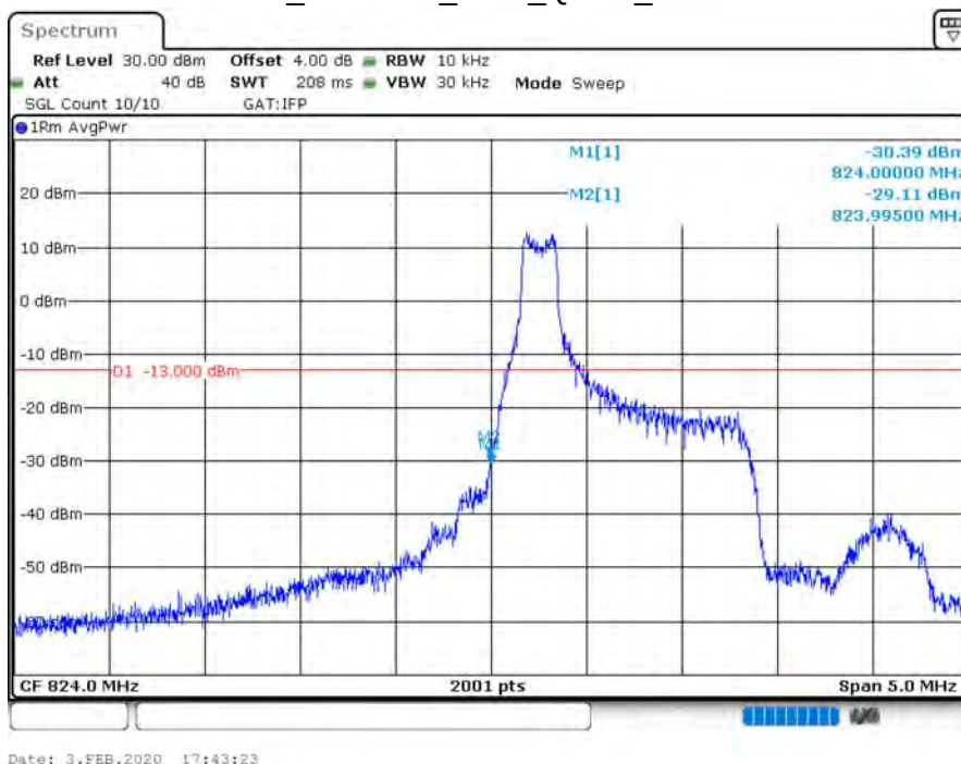
B5_CH20407_1.4M_QPSK_1RB0
