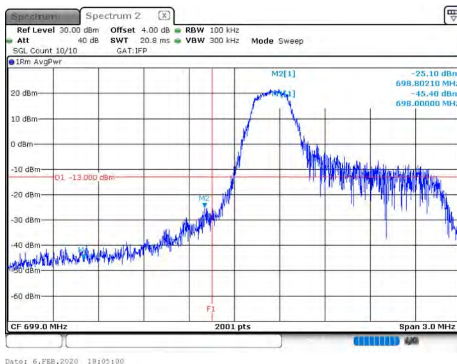
B12_CH23017_1.4M_QPSK_1RB0_150k
