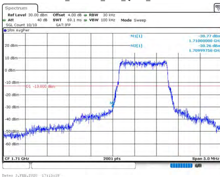
B4_CH19957_1.4M_QPSK_6RB0
