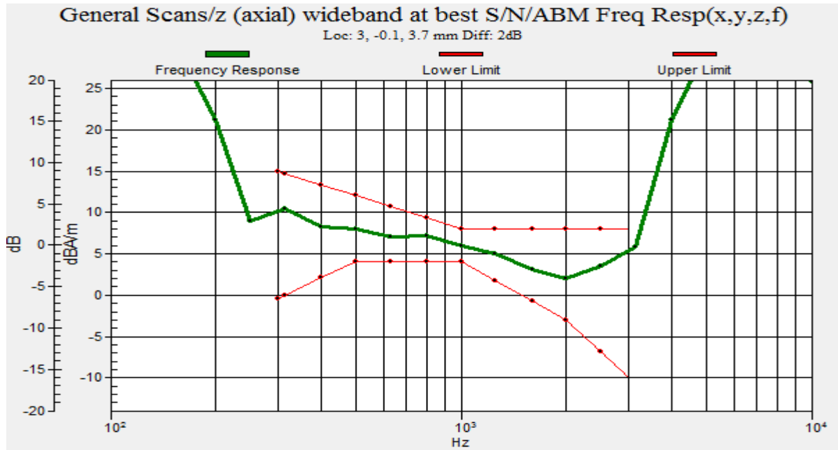
Graph 1 : CDMA (CH 1013) Frequency Response
