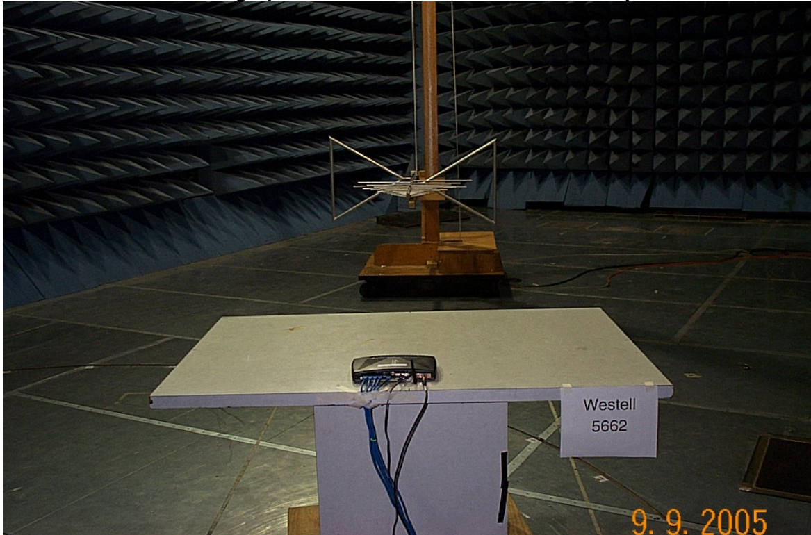
Photographs of Radiated Emissions Test Setup
