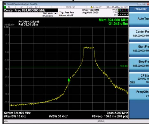
Band26-5MHz-QPSK-26815-25RB#0
