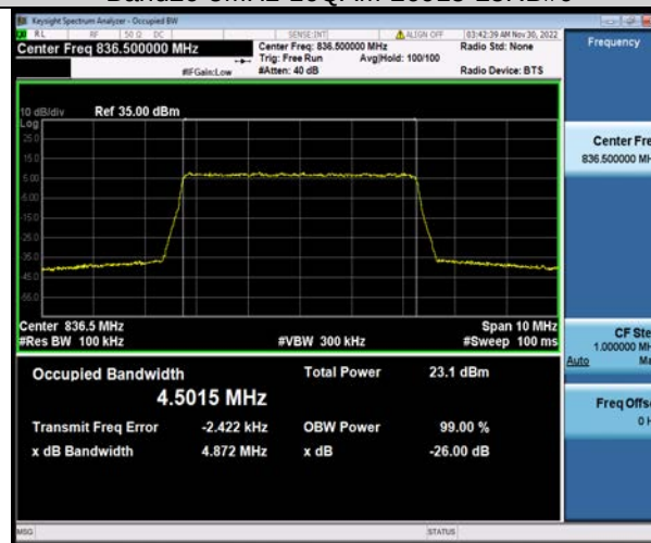
Band26-5MHz-16QAM-27015-25RB#0
