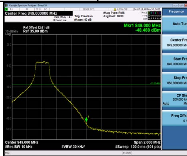
Band26-10MHz-64QAM-26990-50RB#0
