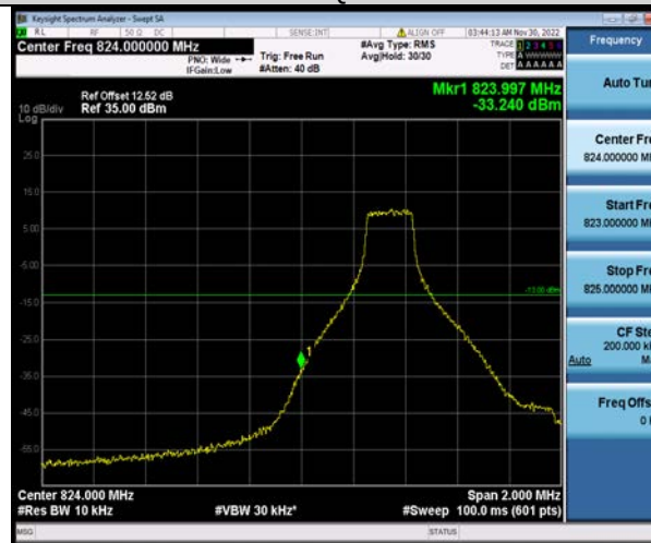
Band26-5MHz-16QAM-26815-25RB#0
