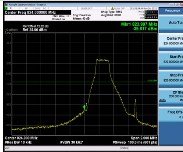
Band26-1.4MHz-64QAM-26797-6RB#0
