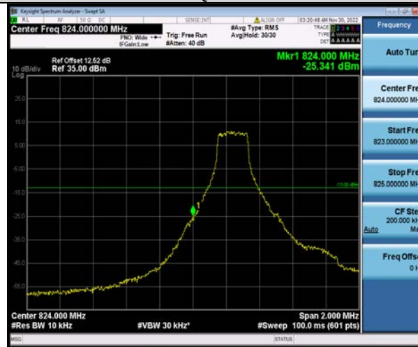
Band26-3MHz-QPSK-26805-15RB#0
