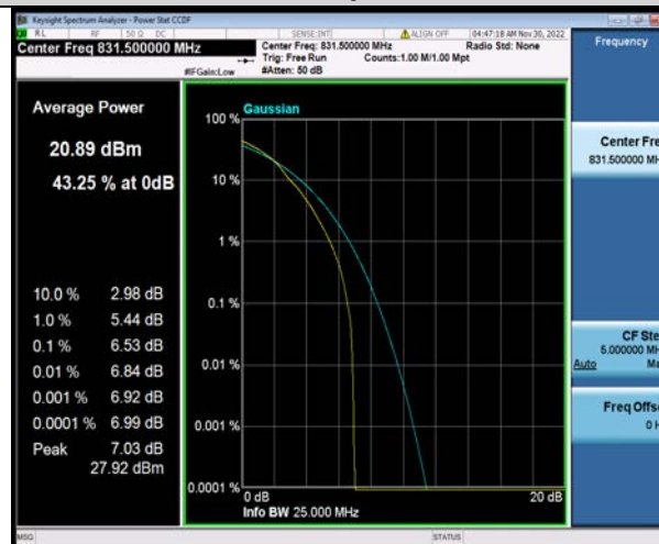
Band26-15MHz-64QAM-26865-75RB#0
