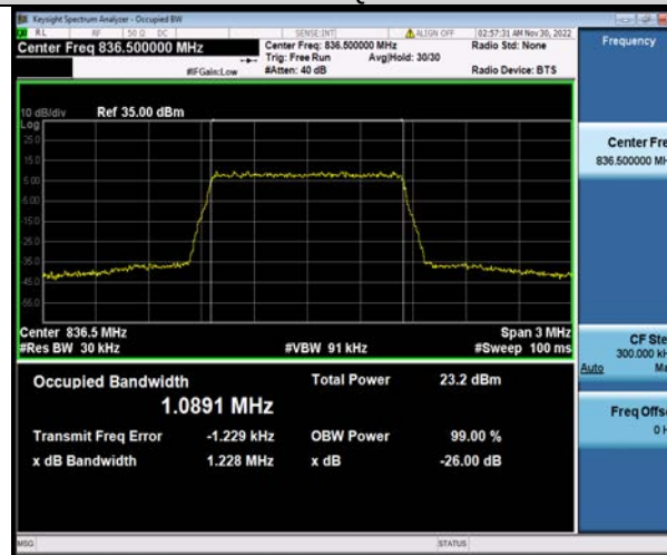
Band26-1.4MHz-16QAM-27033-6RB#0
