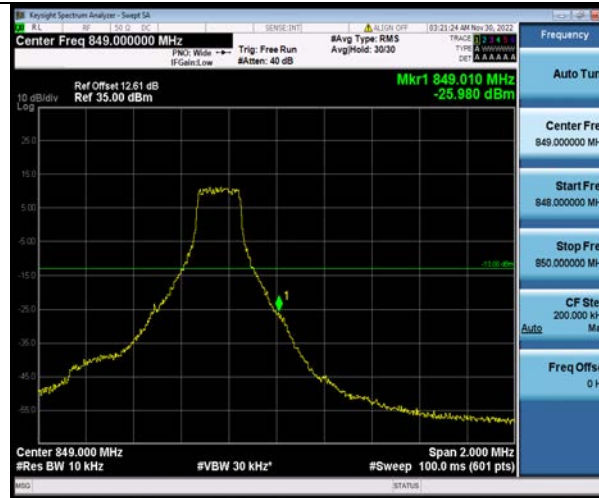
Band26-3MHz-QPSK-27025-15RB#0
