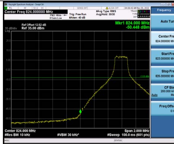
Band26-10MHz-64QAM-26840-50RB#0
