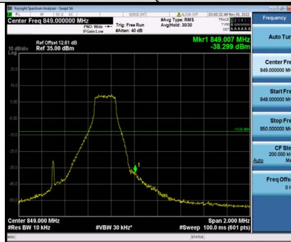
Band26-1.4MHz-64QAM-27033-6RB#0
