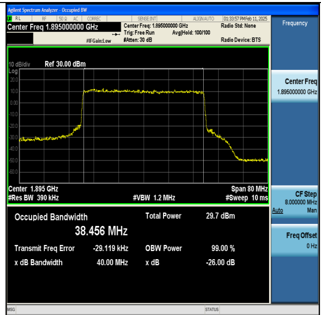
NTNV-n25-PC3-15-40-H-CP-16QAM-Outer_Full-Ant1-PASS
