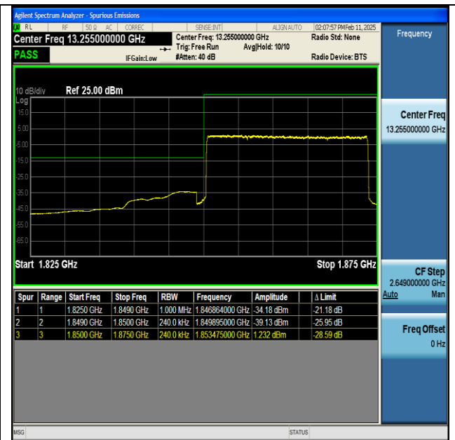
NTNV-n25-PC3-15-25-L-DFT-BPSK-Outer_Full-PASS
