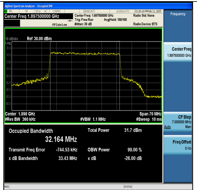
NTNV-n25-PC3-15-35-H-DFT-QPSK-Outter_Full-Ant1- PASS
