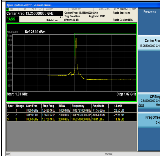
NTNV-n25-PC3-15-20-L-CP-QPSK-Edge_1RB_Left-PASS
