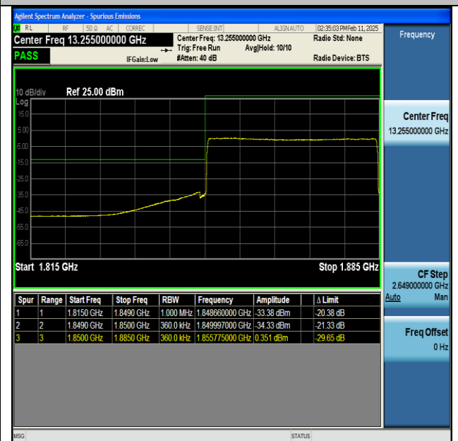
NTNV-n25-PC3-15-35-L-CP-QPSK-Outer_Full-PASS
