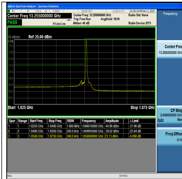
NTNV-n25-PC3-15-25-L-DFT-BPSK-Edge_1RB_Left-PASS
