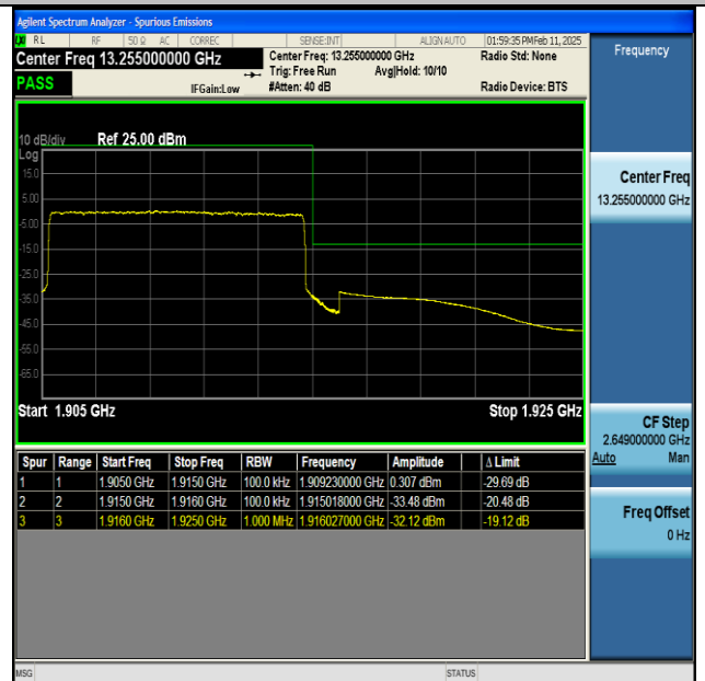
NTNV-n25-PC3-15-10-H-CP-QPSK-Outer_Full-PASS
