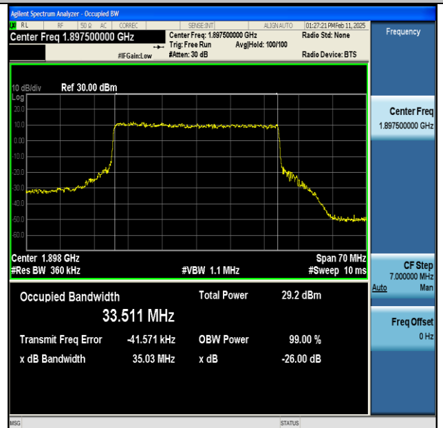
NTNV-n25-PC3-15-35-H-CP-64QAM-Outer_Full-Ant1-PASS
