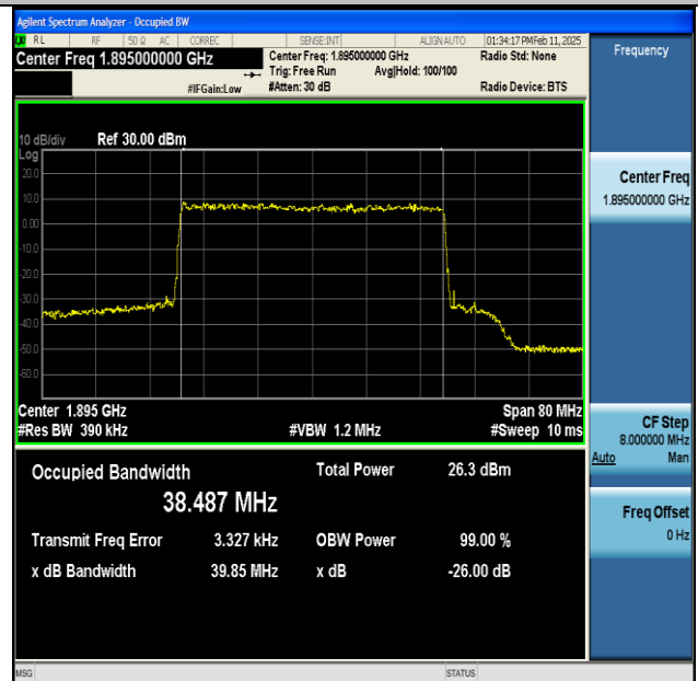
NTNV-n25-PC3-15-40-H-CP-256QAM-Outer_Full-Ant1-PASS
