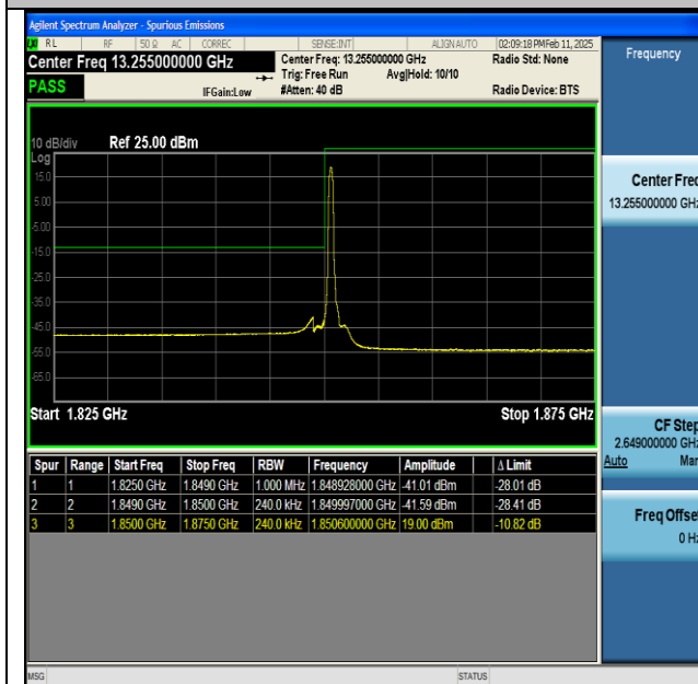
NTNV-n25-PC3-15-25-L-CP-QPSK-Edge_1RB_Left-PASS
