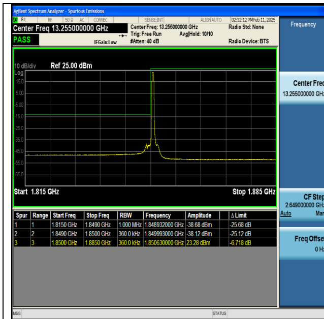
NTNV-n25-PC3-15-35-L-DFT-BPSK-Edge_1RB_Left-PASS
