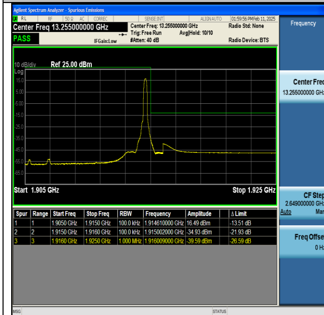
NTNV-n25-PC3-15-10-H-CP-QPSK-Edge_1RB_Right-PASS
