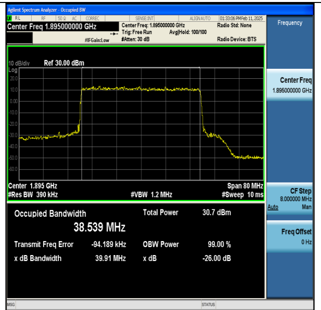
NTNV-n25-PC3-15-40-H-DFT-16QAM-Outer_Full-Ant1- PASS
