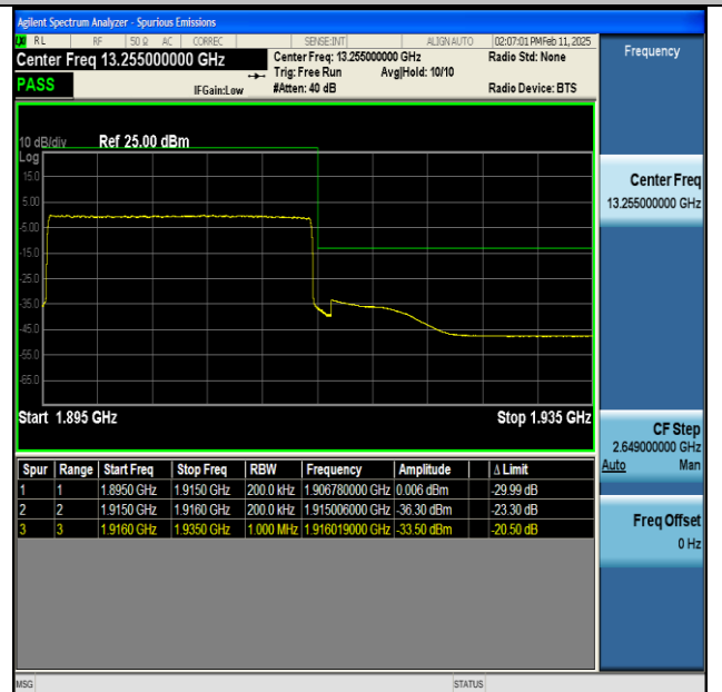
NTNV-n25-PC3-15-20-H-CP-QPSK-Outer_Full-PASS
