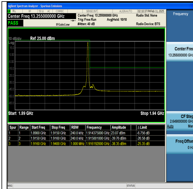
NTNV-n25-PC3-15-25-H-DFT-BPSK-Edge_1RB_Right-PASS
