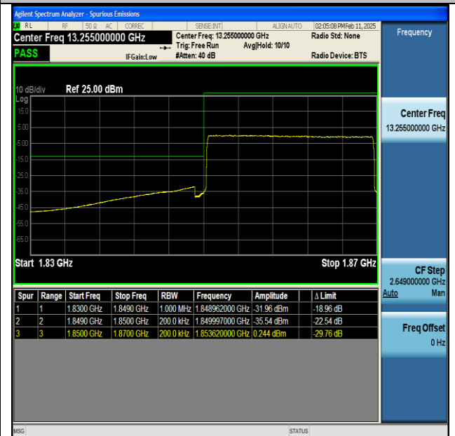
NTNV-n25-PC3-15-20-L-CP-QPSK-Outer_Full-PASS
