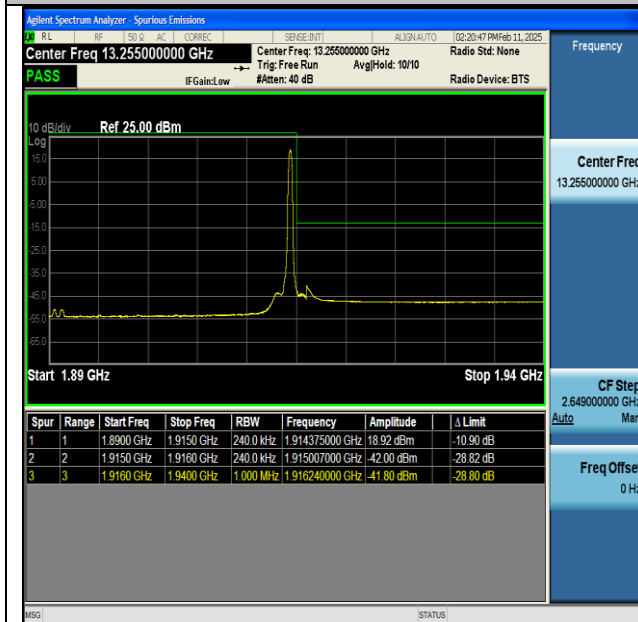
NTNV-n25-PC3-15-25-H-CP-QPSK-Edge_1RB_Right-PASS
