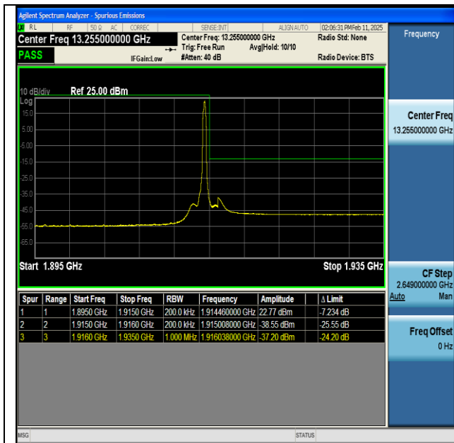
NTNV-n25-PC3-15-20-H-DFT-BPSK-Edge_1RB_Right-PASS
