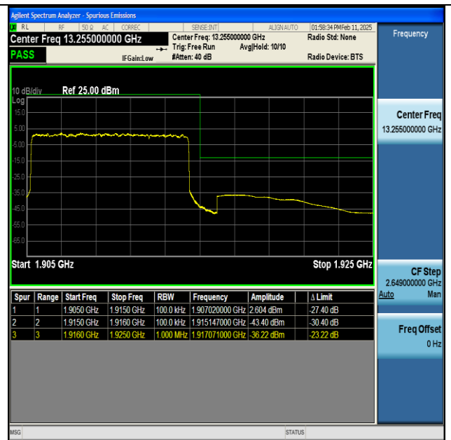
NTNV-n25-PC3-15-10-H-DFT-BPSK-Outer_Full-PASS
