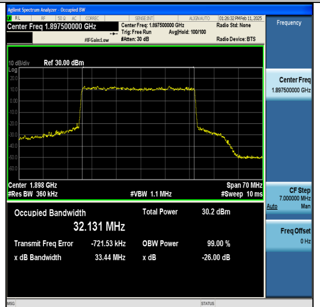
NTNV-n25-PC3-15-35-H-DFT-64QAM-Outter_Full-Ant1- PASS
