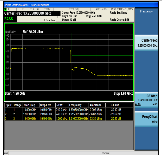
NTNV-n25-PC3-15-25-H-CP-QPSK-Outer_Full-PASS
