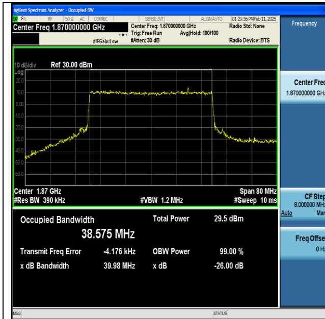
NTNV-n25-PC3-15-40-L-CP-64QAM-Outer_Full-Ant1- PASS
