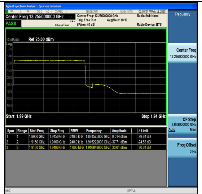
NTNV-n25-PC3-15-25-H-DFT-BPSK-Outer_Full-PASS
