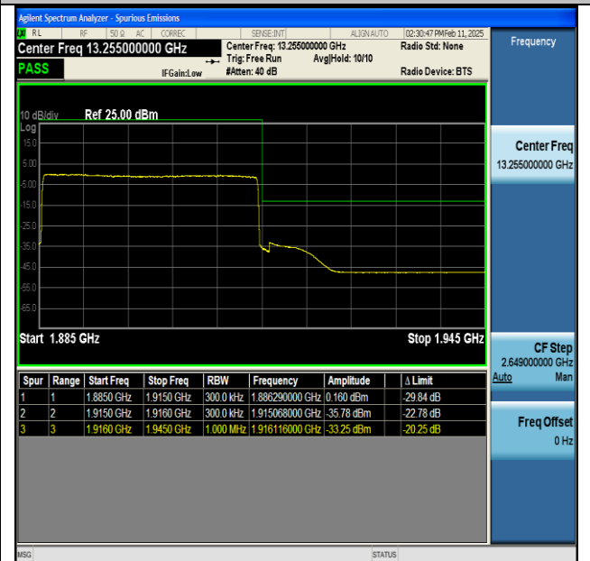
NTNV-n25-PC3-15-30-H-CP-QPSK-Outer_Full-PASS
