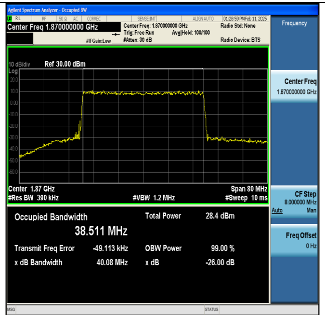
NTNV-n25-PC3-15-40-L-DFT-256QAM-Outer_Full-Ant1- PASS
