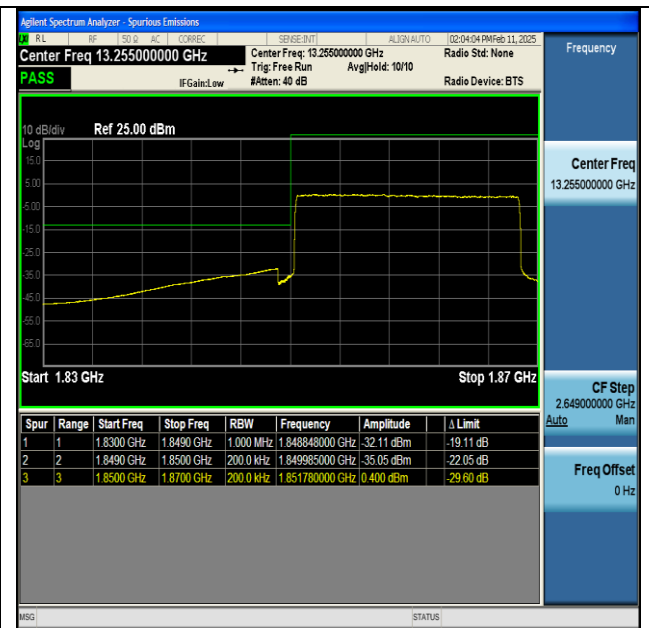
NTNV-n25-PC3-15-20-L-DFT-BPSK-Outer_Full-PASS
