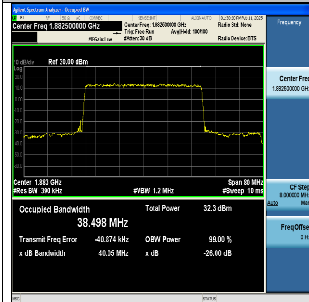
NTNV-n25-PC3-15-40-M-DFT-BPSK-Outer_Full-Ant1- PASS
