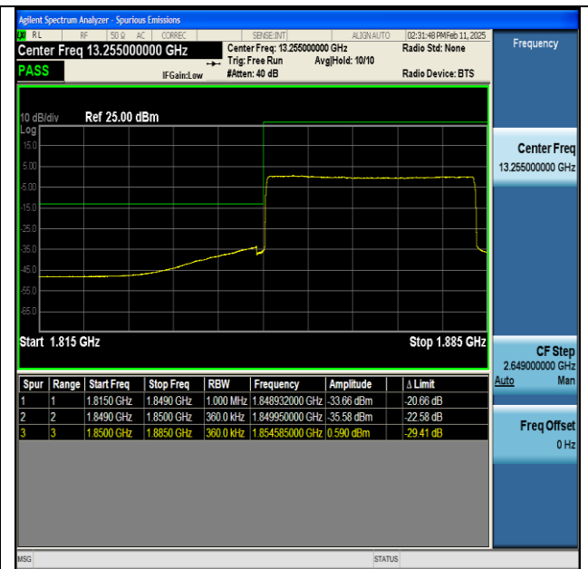
NTNV-n25-PC3-15-35-L-DFT-BPSK-Outer_Full-PASS
