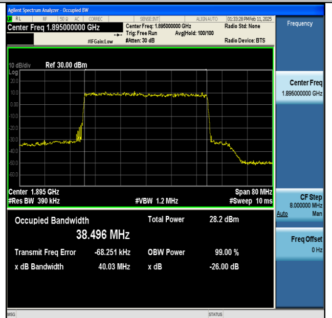
NTNV-n25-PC3-15-40-H-DFT-256QAM-Outer_Full-Ant1- PASS
