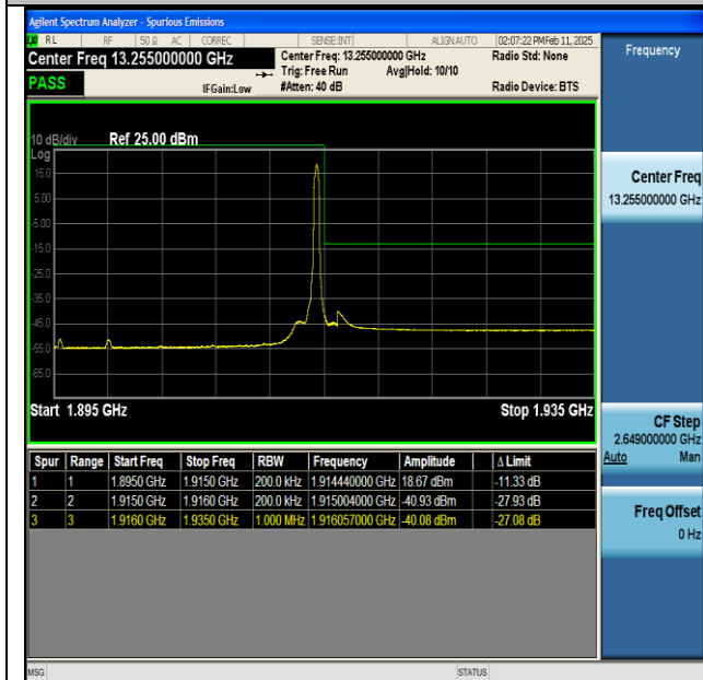
NTNV-n25-PC3-15-20-H-CP-QPSK-Edge_1RB_Right-PASS
