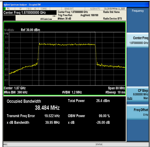
NTNV-n25-PC3-15-40-L-CP-256QAM-Outer_Full-Ant1- PASS
