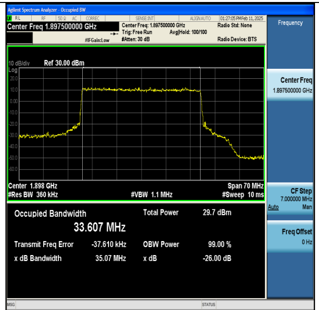
NTNV-n25-PC3-15-35-H-CP-QPSK-Outer_Full-Ant1-PASS
