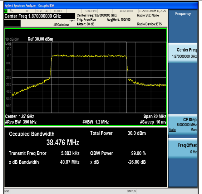
NTNV-n25-PC3-15-40-L-CP-16QAM-Outer_Full-Ant1- PASS
