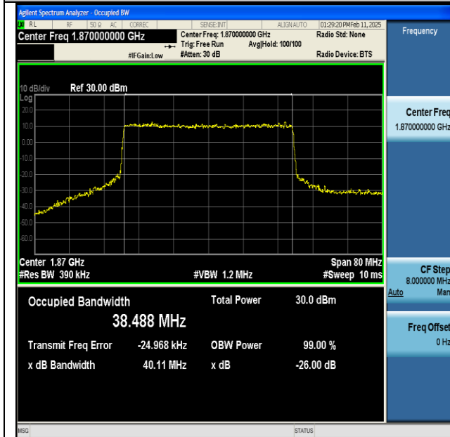
NTNV-n25-PC3-15-40-L-DFT-64QAM-Outer_Full-Ant1- PASS
