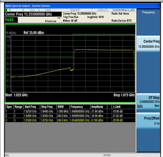
NTNV-n25-PC3-15-25-L-CP-QPSK-Outer_Full-PASS
