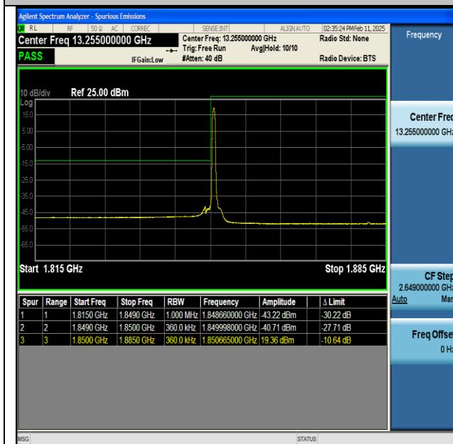
NTNV-n25-PC3-15-35-L-CP-QPSK-Edge_1RB_Left-PASS
