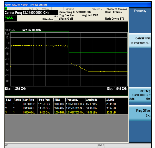
NTNV-n25-PC3-15-30-H-DFT-BPSK-Outer_Full-PASS
