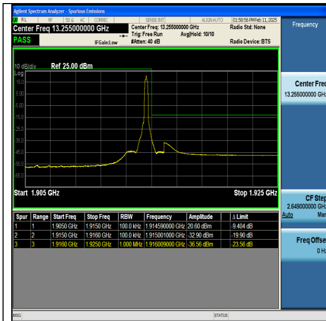
NTNV-n25-PC3-15-10-H-DFT-BPSK-Edge_1RB_Right-PASS
