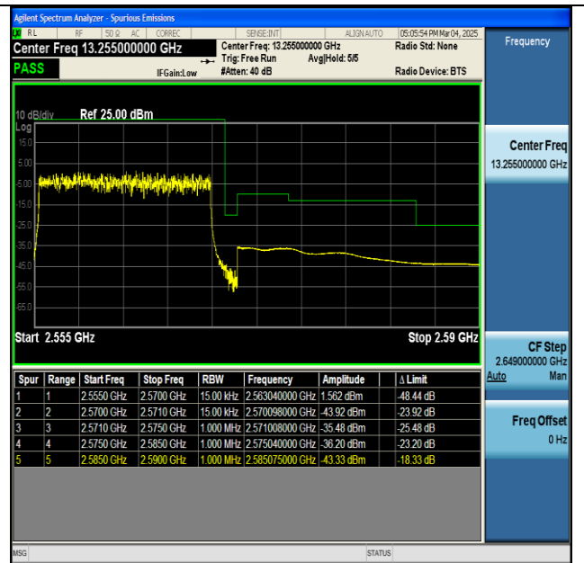
NTNV-n7-PC3-15-15-H-DFT-BPSK-Outer_Full-PASS
