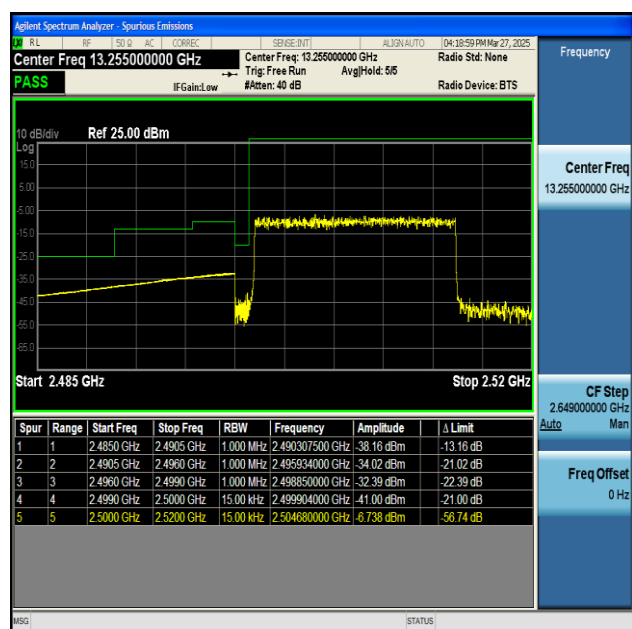
NTNV-n7-PC3-15-15-L-CP-QPSK-Outer_Full-PASS
