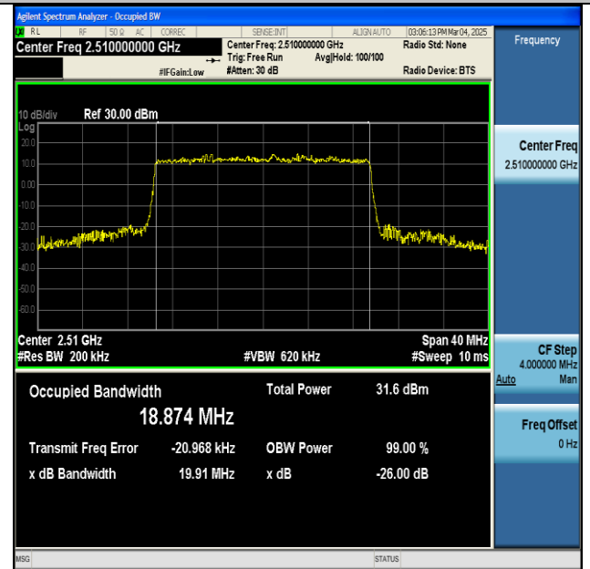
NTNV-n7-PC3-15-20-L-CP-16QAM-Outer_Full-Ant1-PASS
