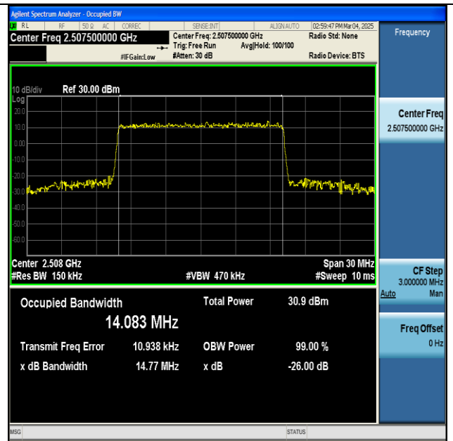
NTNV-n7-PC3-15-15-L-CP-64QAM-Outer_Full-Ant1-PASS
