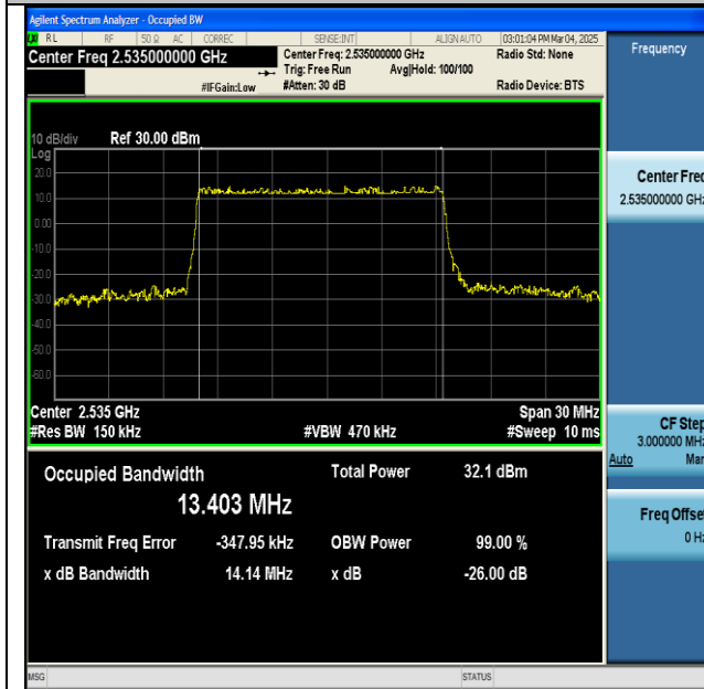
NTNV-n7-PC3-15-15-M-DFT-64QAM-Outet_Full-Ant1-PASS
