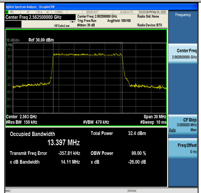
NTNV-n7-PC3-15-15-H-DFT-64QAM-Outet_Full-Ant1-PASS
