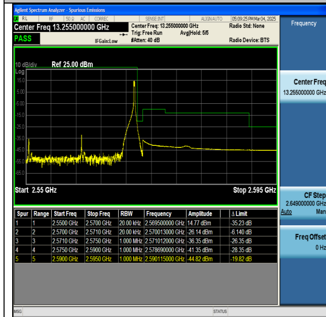
NTNV-n7-PC3-15-20-H-CP-QPSK-Edge_1RB_Right-PASS
