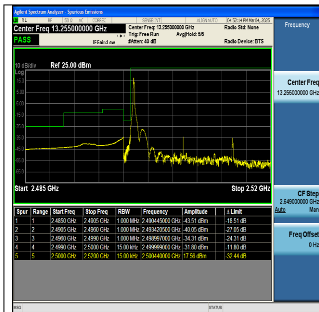
NTNV-n7-PC3-15-15-L-DFT-BPSK-Edge_1RB_Left-PASS
