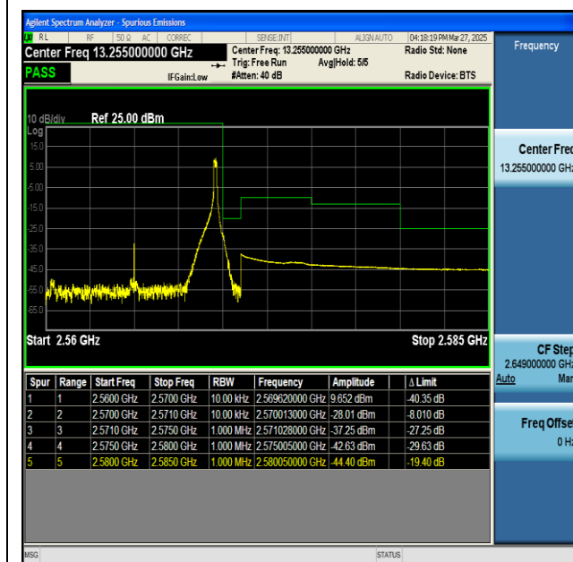
NTNV-n7-PC3-15-10-H-CP-QPSK-Edge_1RB_Right-PASS
