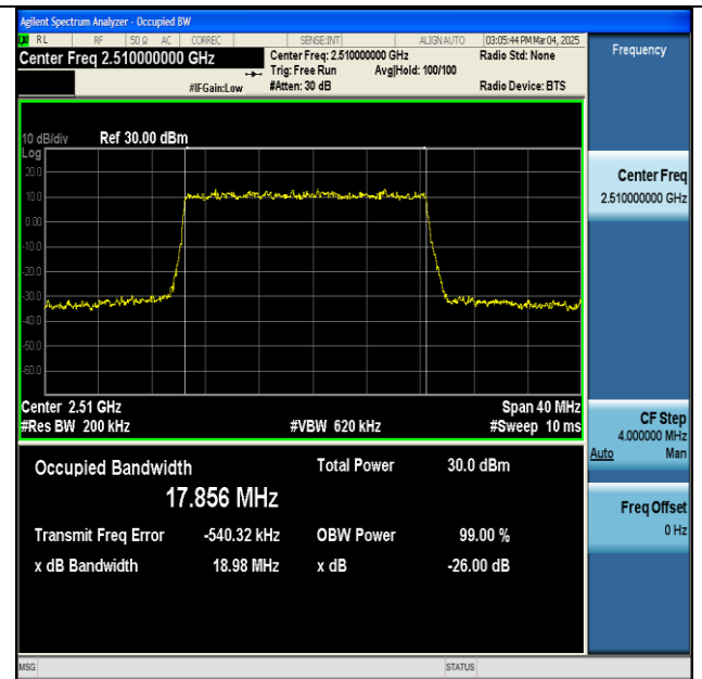
NTNV-n7-PC3-15-20-L-DFT-256QAM-Outer_Full-Ant1-PASS
