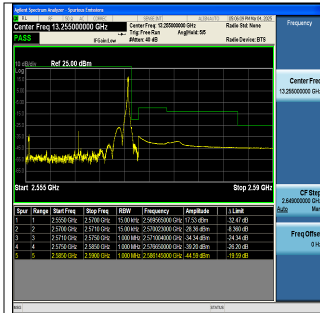
NTNV-n7-PC3-15-15-H-DFT-BPSK-Edge_1RB_Right-PASS
