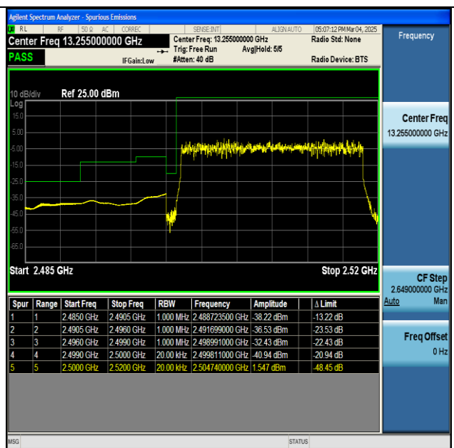
NTNV-n7-PC3-15-20-L-DFT-BPSK-Outer_Full-PASS
