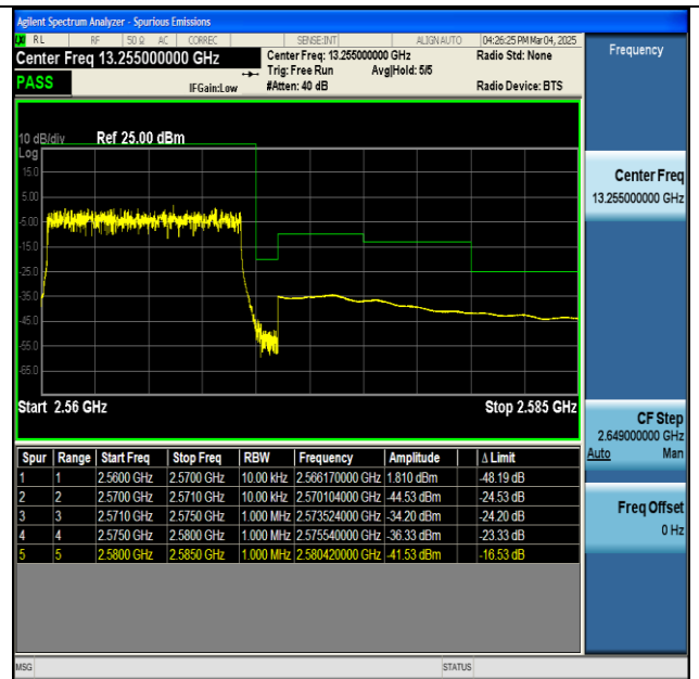
NTNV-n7-PC3-15-10-H-DFT-BPSK-Outer_Full-PASS
