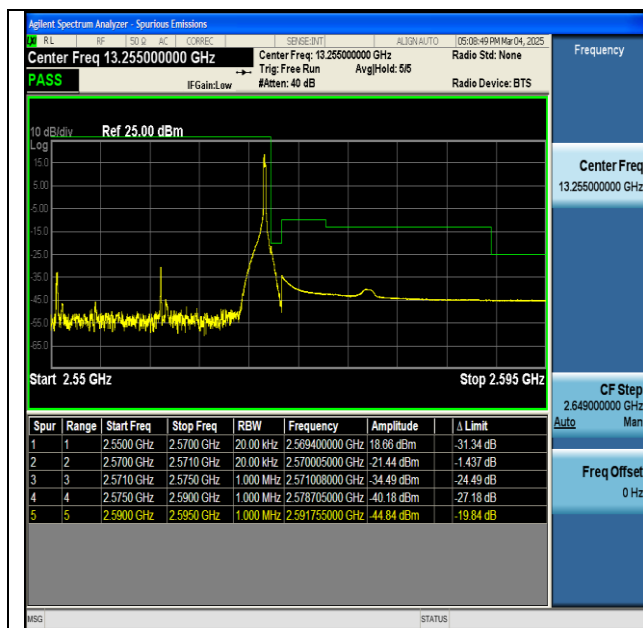
NTNV-n7-PC3-15-20-H-DFT-BPSK-Edge_1RB_Right-PASS
