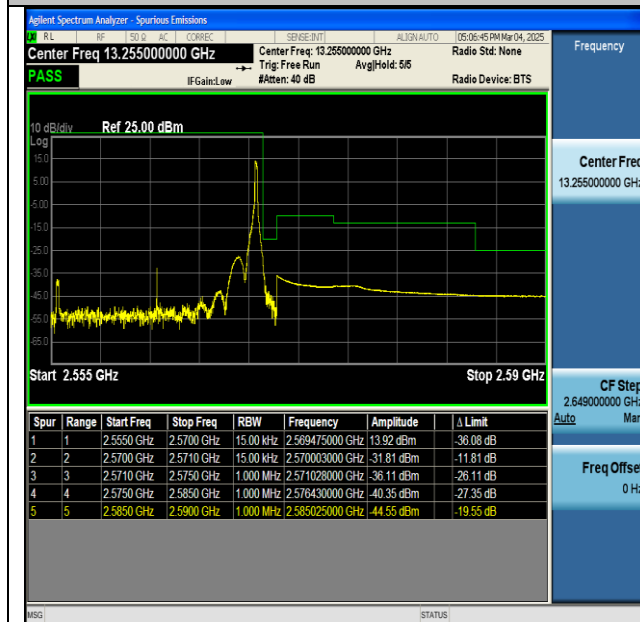
NTNV-n7-PC3-15-15-H-CP-QPSK-Edge_1RB_Right-PASS
