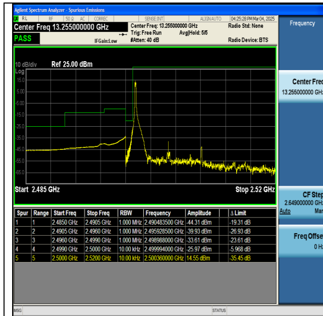
NTNV-n7-PC3-15-10-L-DFT-BPSK-Edge_1RB_Left-PASS
