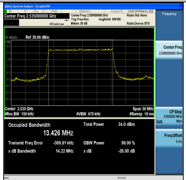
NTNV-n7-PC3-15-15-L-CP-64QAM-Outer_Full-Ant1-PASS
