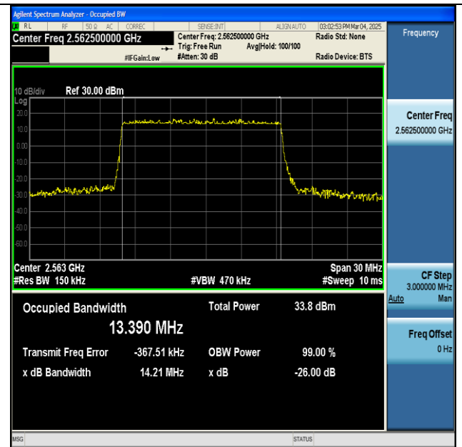
NTNV-n7-PC3-15-15-H-DFT-QPSK-Outet_Full-Ant1-PASS
