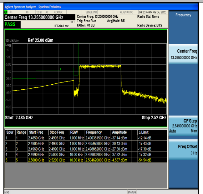
NTNV-n7-PC3-15-10-L-CP-QPSK-Outer_Full-PASS
