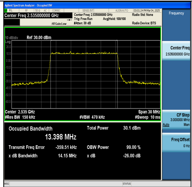
NTNV-n7-PC3-15-15-M-DFT-256QAM-Outet_Full-Ant1-PASS
