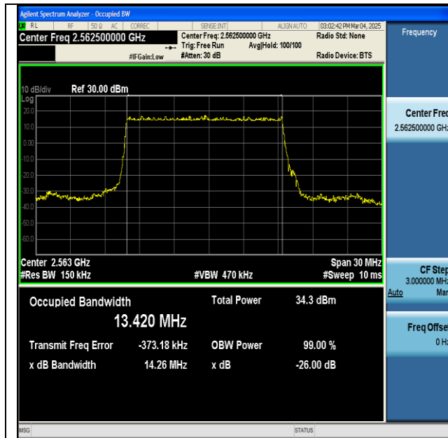
NTNV-n7-PC3-15-15-H-DFT-BPSK-Outet_Full-Ant1-PASS
