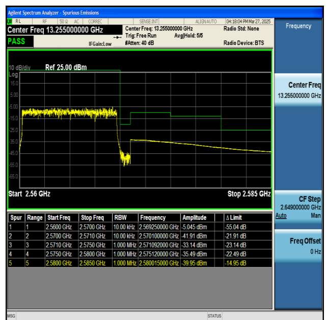
NTNV-n7-PC3-15-10-H-CP-QPSK-Outer_Full-PASS
