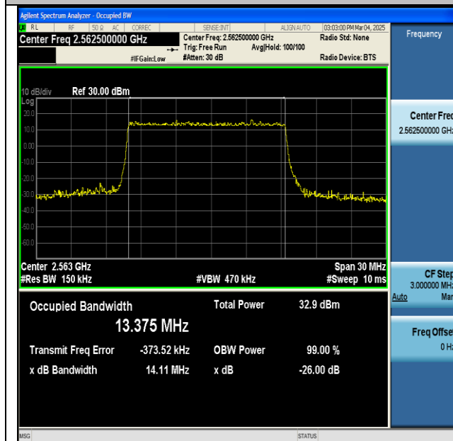
NTNV-n7-PC3-15-15-H-DFT-16QAM-Outet_Full-Ant1-PASS
