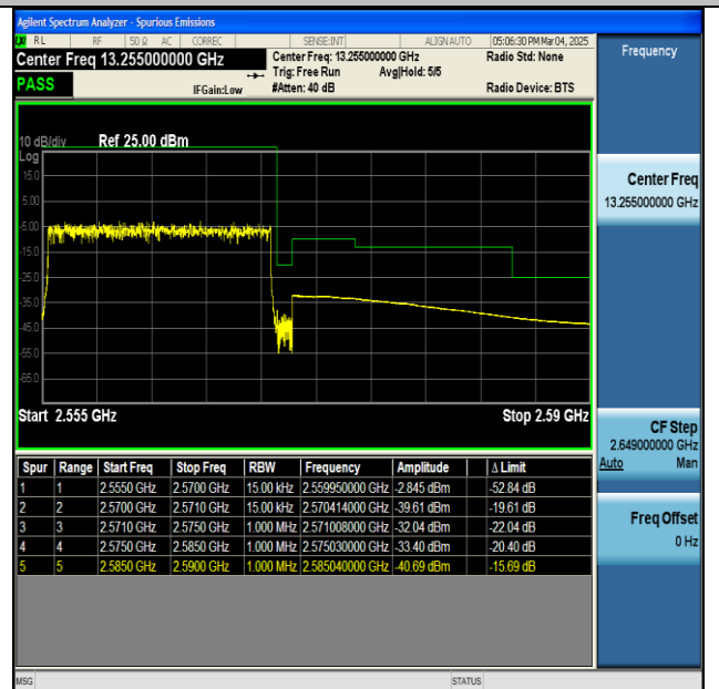
NTNV-n7-PC3-15-15-H-CP-QPSK-Outer_Full-PASS
