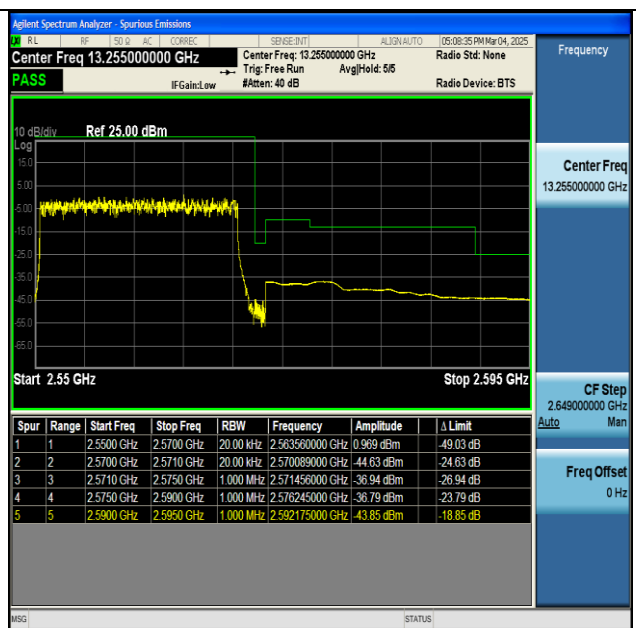
NTNV-n7-PC3-15-20-H-DFT-BPSK-Outer_Full-PASS
