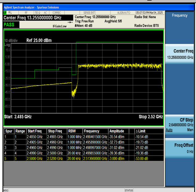
NTNV-n7-PC3-15-20-L-CP-QPSK-Outer_Full-PASS
