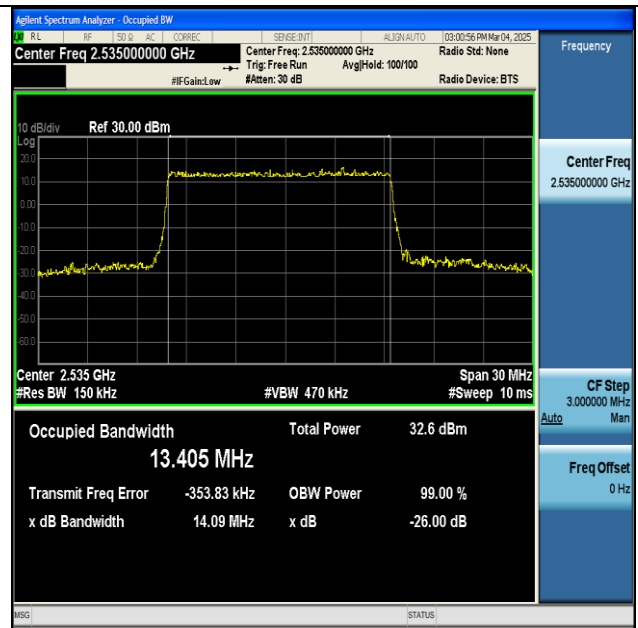
NTNV-n7-PC3-15-15-M-DFT-16QAM-Outet_Full-Ant1-PASS
