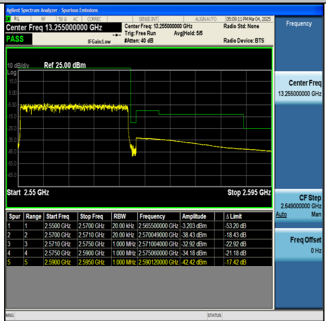
NTNV-n7-PC3-15-20-H-CP-QPSK-Outer_Full-PASS
