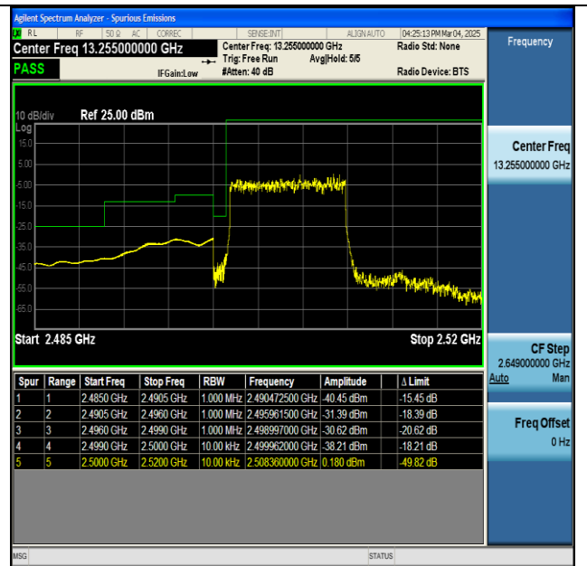
NTNV-n7-PC3-15-10-L-DFT-BPSK-Outer_Full-PASS
