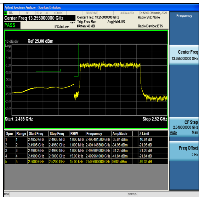
NTNV-n7-PC3-15-15-L-DFT-BPSK-Outer_Full-PASS
