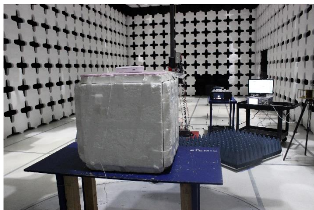
Spurious Emission Above 1GHz-Front View
