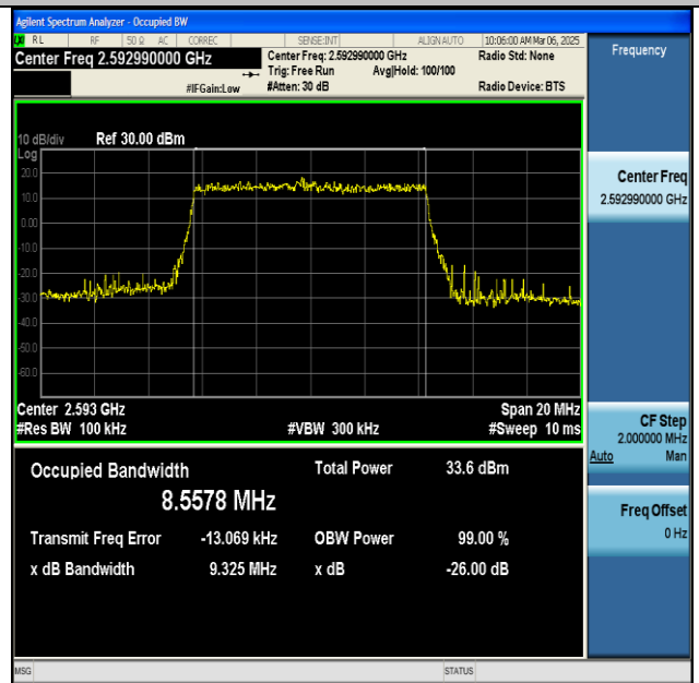
NTNV-n41-PC2-30-10-M-DFT-16QAM-Outer_Full-Ant1- PASS
