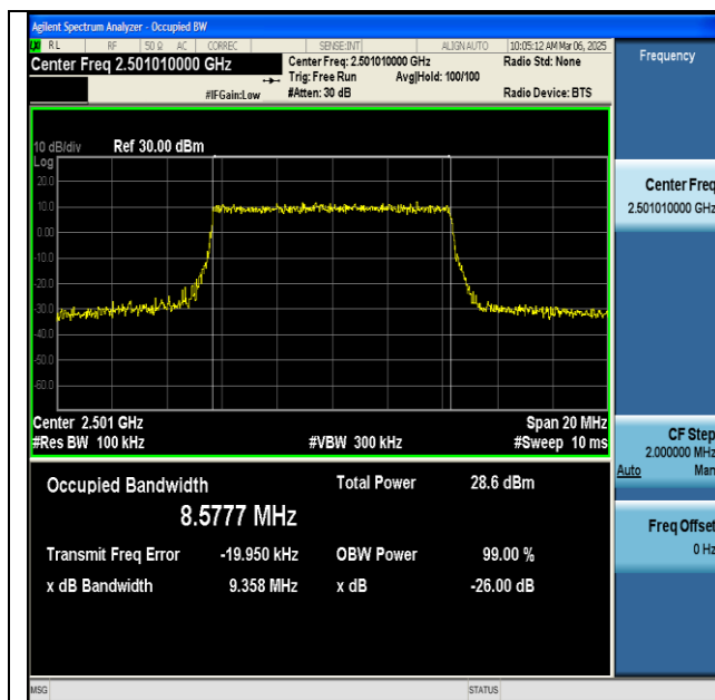
NTNV-n41-PC2-30-10-L-CP-256QAM-Outer_Full-Ant1- PASS
