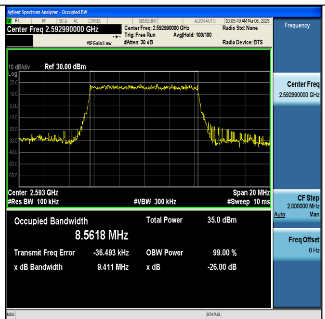
NTNV-n41-PC2-30-10-M-DFT-BPSK-Outer_Full-Ant1- PASS
