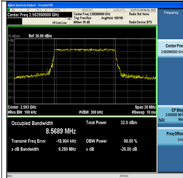
NTNV-n41-PC2-30-10-M-DFT-64QAM-Outer_Full-Ant1- PASS
