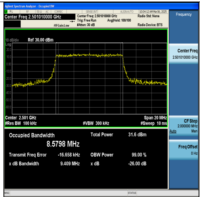
NTNV-n41-PC2-30-10-L-CP-QPSK-Outer_Full-Ant1-PASS
