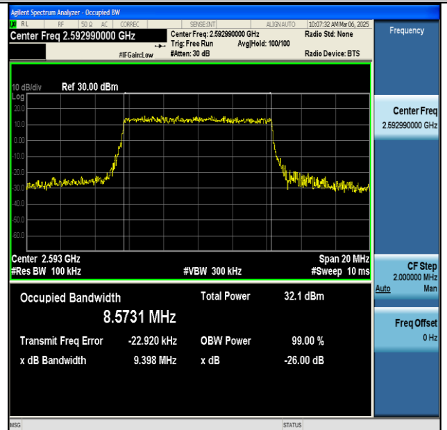
NTNV-n41-PC2-30-10-M-CP-16QAM-Outer_Full-Ant1- PASS
