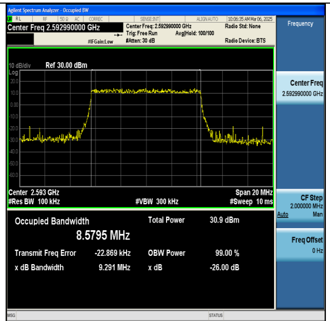
NTNV-n41-PC2-30-10-M-DFT-256QAM-Outer_Full-Ant1- PASS
