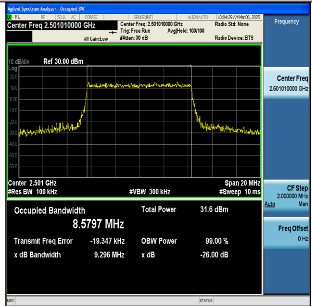
NTNV-n41-PC2-30-10-L-CP-64QAM-Outer_Full-Ant1-PASS
