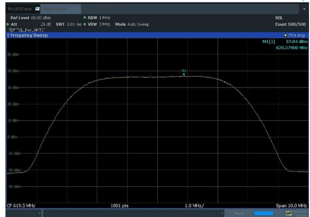
Plot 8-32. Power Spectral Density Plot (LTE_B71_1C_5M_16QAM - Low Channel, Port 1)
