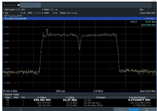
Plot 8-18. Occupied Bandwidth Plot (LTE_B71_2C_5M+5M_16QAM – Mid Channel, Port 0)
