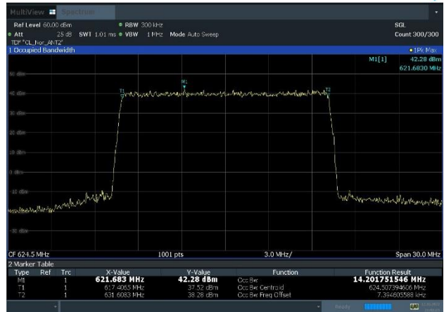
Plot 8-4. Occupied Bandwidth Plot (NR_n71_1C_15M_256QAM - Low Channel, Port 2)
