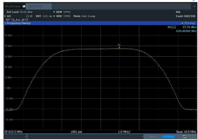
Plot 8-34. Power Spectral Density Plot (LTE_B71_1C_5M_16QAM - Low Channel, Port 3)
