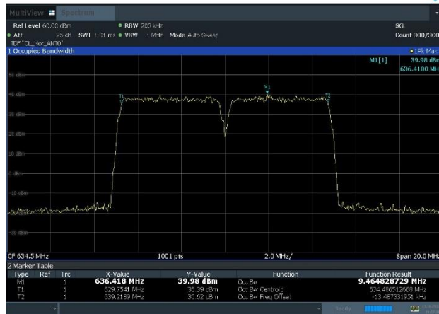
Plot 8-19. Occupied Bandwidth Plot (NR_n71_2C_5M+5M_QPSK – Mid Channel, Port 0)
