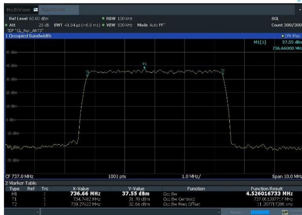
Plot 8-11. Occupied Bandwidth Plot (NR_n85_1C_5M_QPSK – Mid Channel, Port 3)
