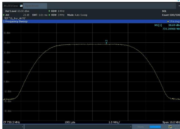
Plot 8-63. Power Spectral Density Plot (NR_n85_1C_5M_256QAM - Low Channel, Port 0)
