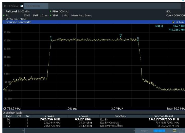
Plot 8-15. Occupied Bandwidth Plot (NR_n85_1C_15M_QPSK – High Channel, Port 3)
