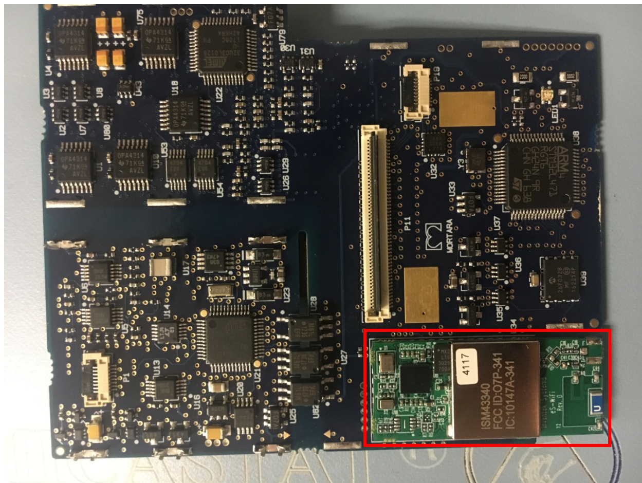
Top of Host Device PCB, with Module Board Outlined
