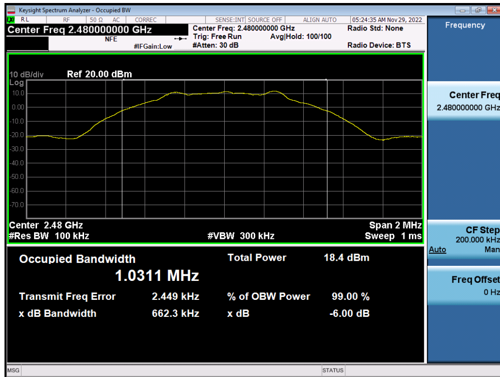
Plot 7-15. 6dB Bandwidth Plot (Bluetooth (LE), 1Mbps – Ch. 39) – ANT 2
