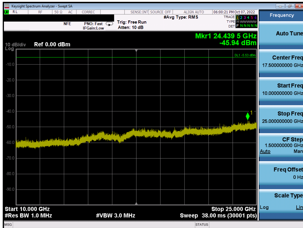
Plot 7-70. Conducted Spurious Plot (Bluetooth (LE), 1Mbps - Ch. 19) - ANT 1
