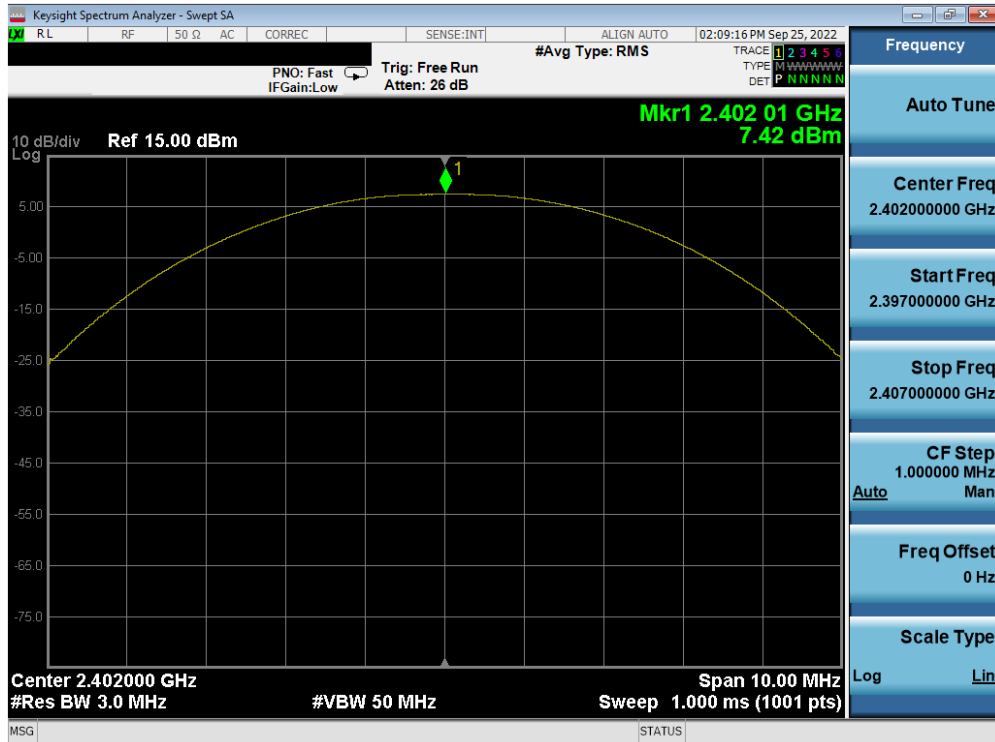
Plot 7-19. Peak Power Plot (Bluetooth (LE), 125kbps – Ch. 0) – ANT 1
