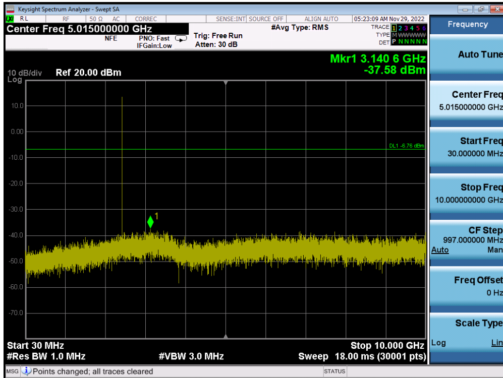
Plot 7-75. Conducted Spurious Plot (Bluetooth (LE), 1Mbps – Ch. 19) – ANT 2
