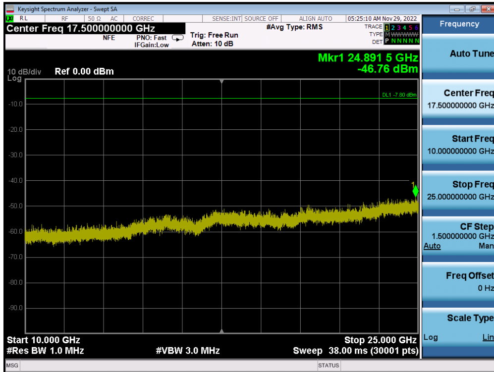
Plot 7-78. Conducted Spurious Plot (Bluetooth (LE), 1Mbps – Ch. 39) – ANT 2
