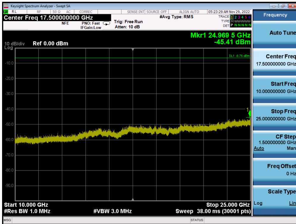
Plot 7-76. Conducted Spurious Plot (Bluetooth (LE), 1Mbps – Ch. 19) – ANT 2
