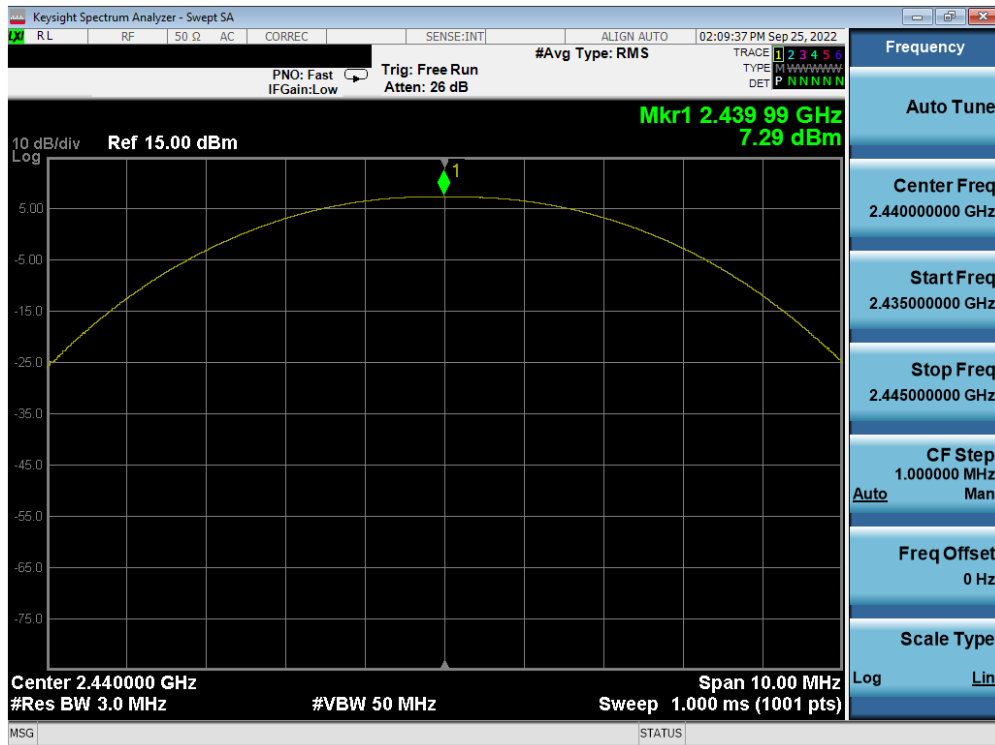
Plot 7-20. Peak Power Plot (Bluetooth (LE), 125kbps – Ch. 19) – ANT 1
