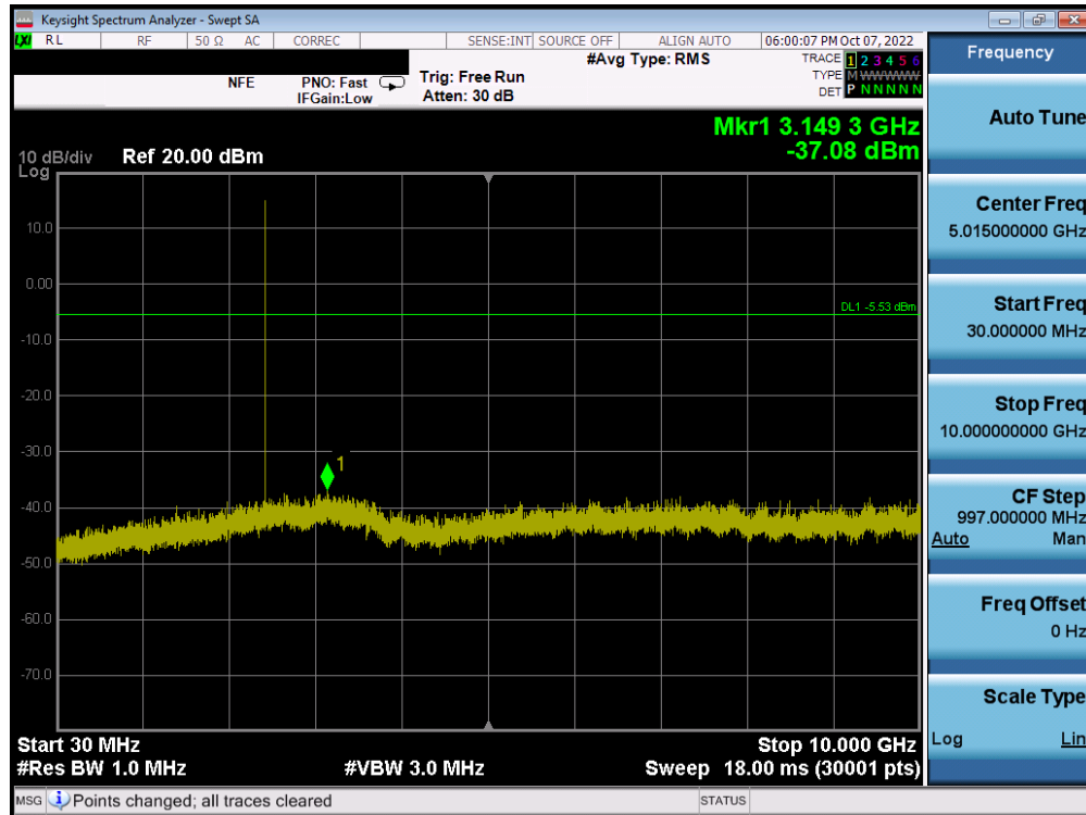
Plot 7-69. Conducted Spurious Plot (Bluetooth (LE), 1Mbps - Ch. 19) - ANT 1
