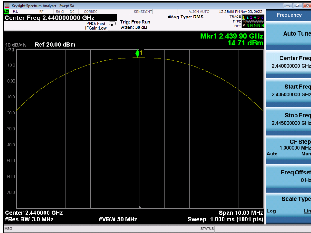
Plot 7-32. Peak Power Plot (Bluetooth (LE), 1Mbps – Ch. 19) – ANT 2
