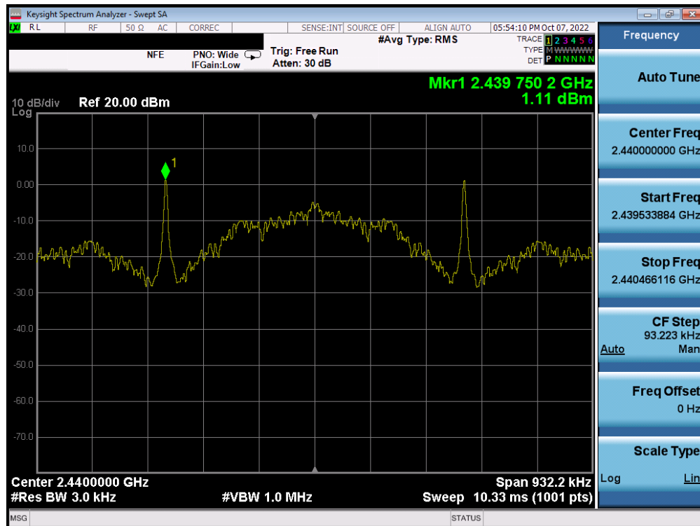
Plot 7-38. Power Spectral Density Plot (Bluetooth (LE), 125kbps – Ch. 19) – ANT 1
