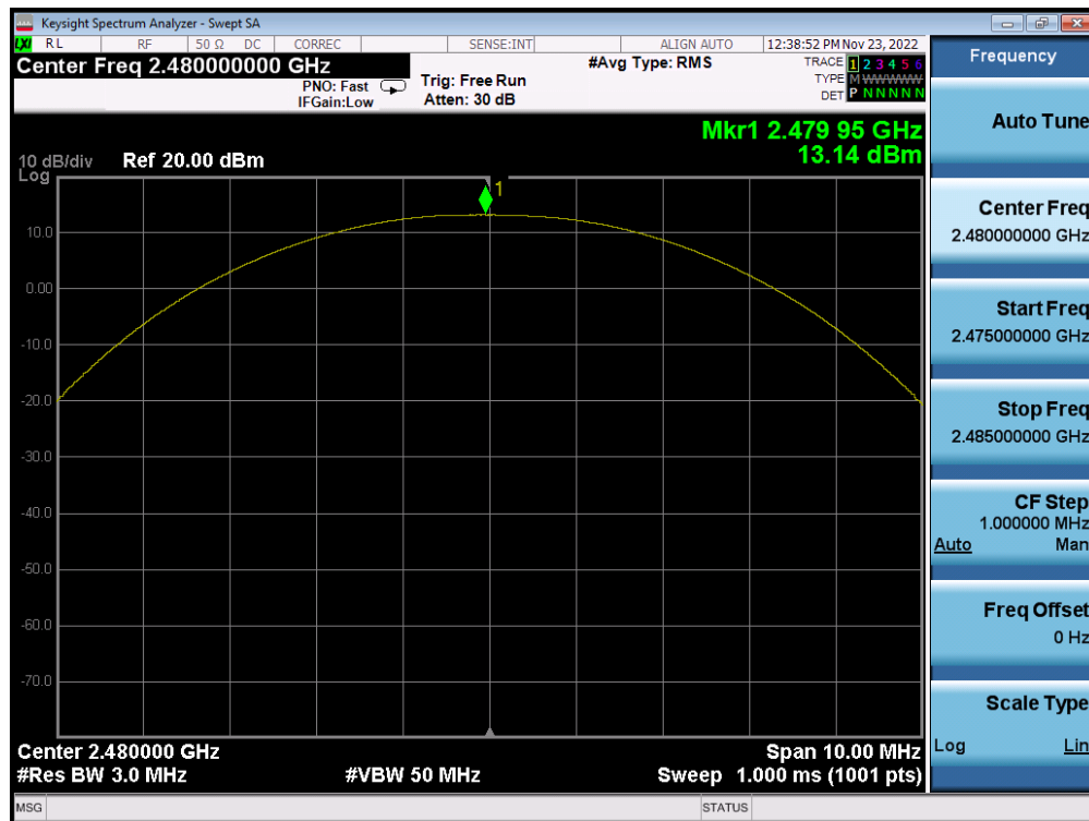
Plot 7-33. Peak Power Plot (Bluetooth (LE), 1Mbps – Ch. 39) – ANT 2
