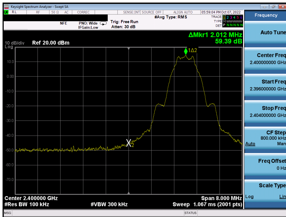
Plot 7-59. Band Edge Plot (Bluetooth (LE), 1Mbps – Ch. 0) – ANT 1
