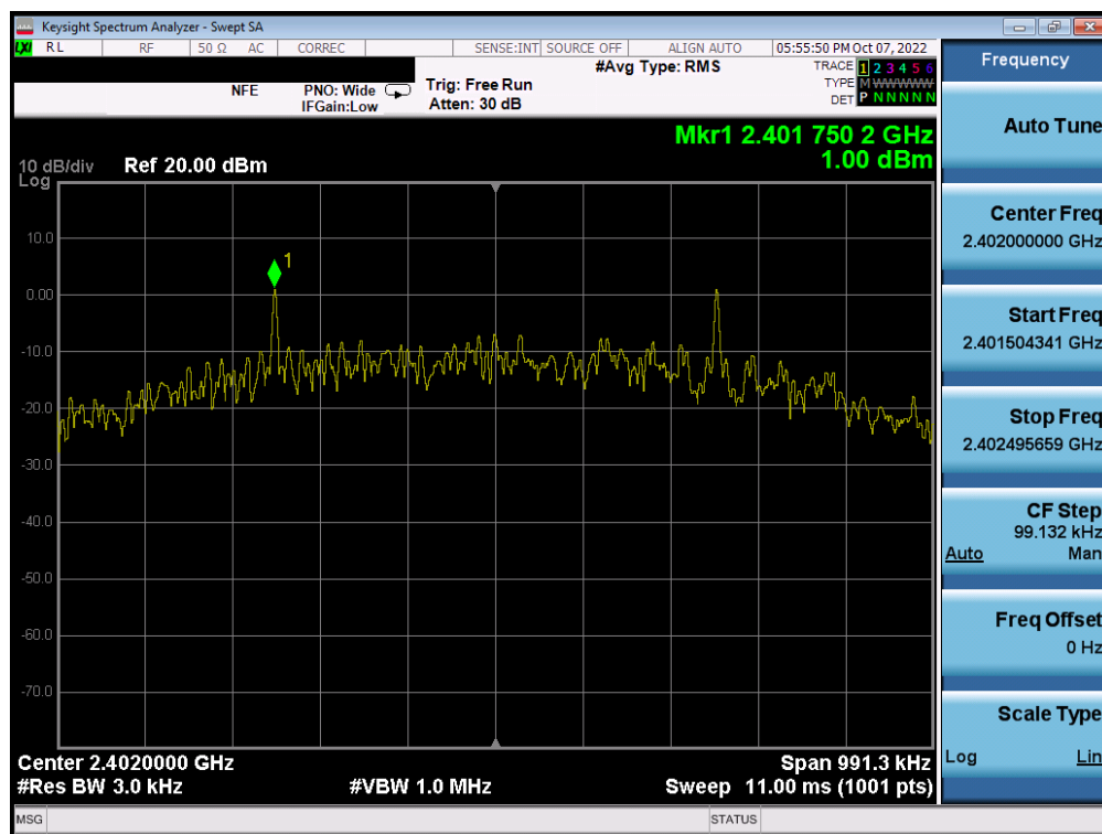
Plot 7-40. Power Spectral Density Plot (Bluetooth (LE), 500kbps – Ch. 0) – ANT 1
