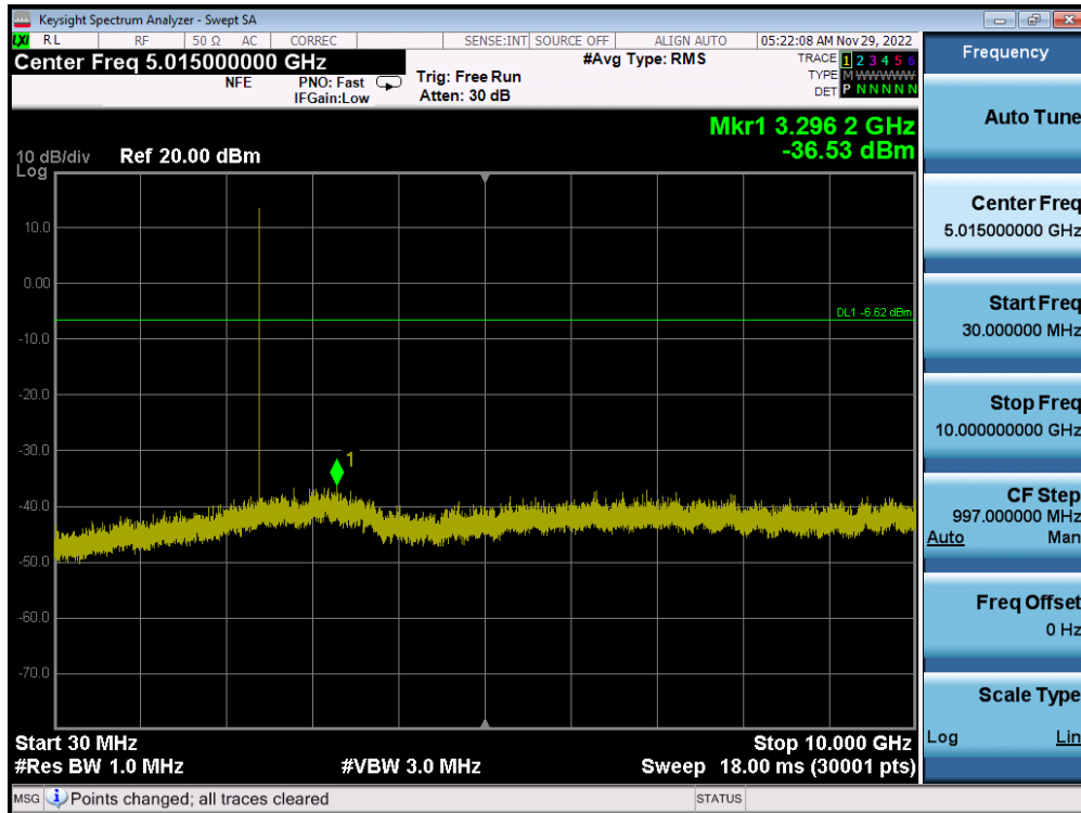
Plot 7-73. Conducted Spurious Plot (Bluetooth (LE), 1Mbps - Ch. 0) - ANT 2
