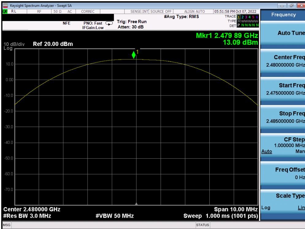
Plot 7-30. Peak Power Plot (Bluetooth (LE), 2Mbps – Ch. 39) – ANT 1
