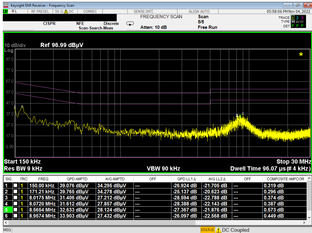
Plot 7-84. Line Conducted Plot with Bluetooth LE (N)
