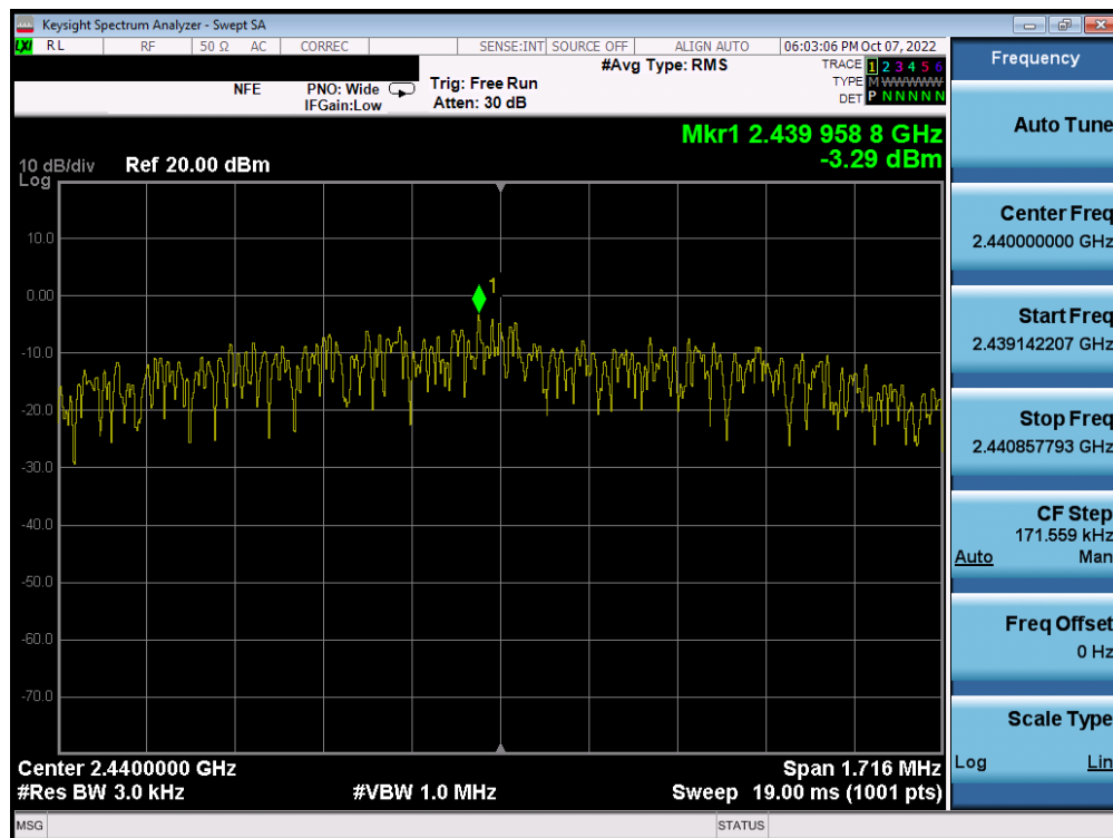
Plot 7-47. Power Spectral Density Plot (Bluetooth (LE), 2Mbps – Ch. 19) – ANT 1
