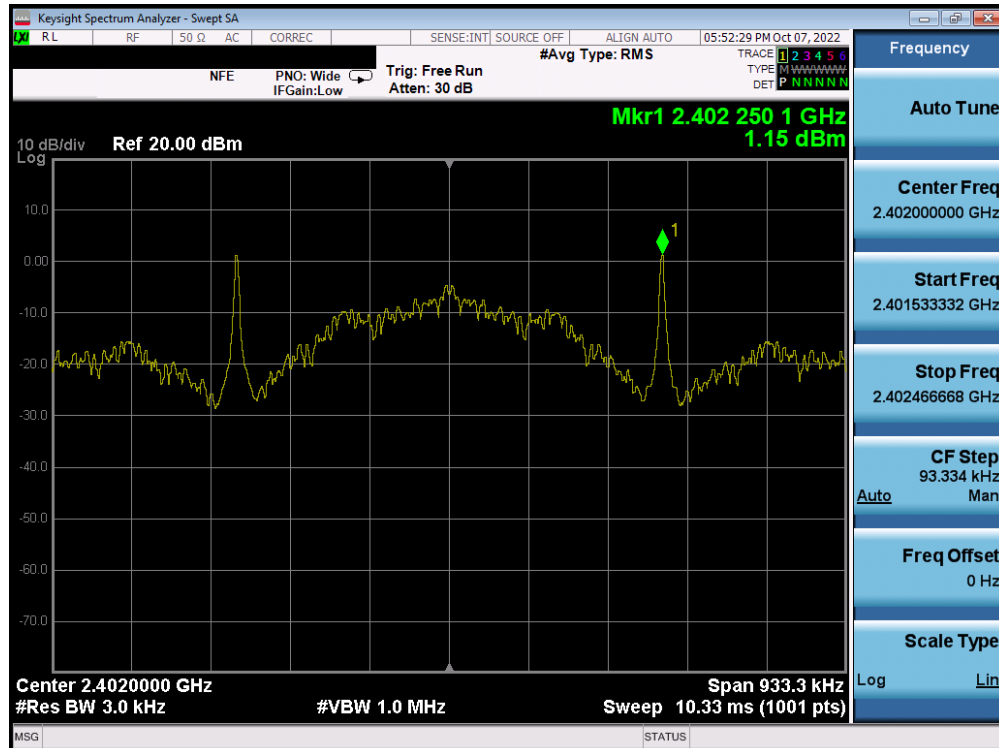
Plot 7-37. Power Spectral Density Plot (Bluetooth (LE), 125kbps – Ch. 0) – ANT 1
