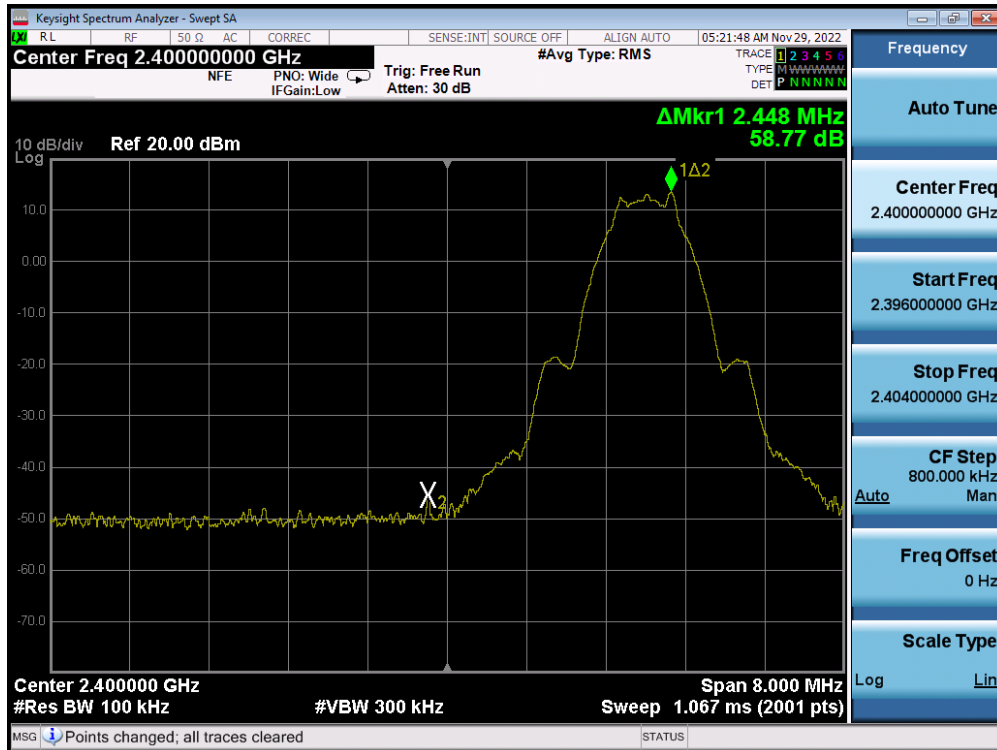
Plot 7-63. Band Edge Plot (Bluetooth (LE), 1Mbps - Ch. 0) - ANT 2
