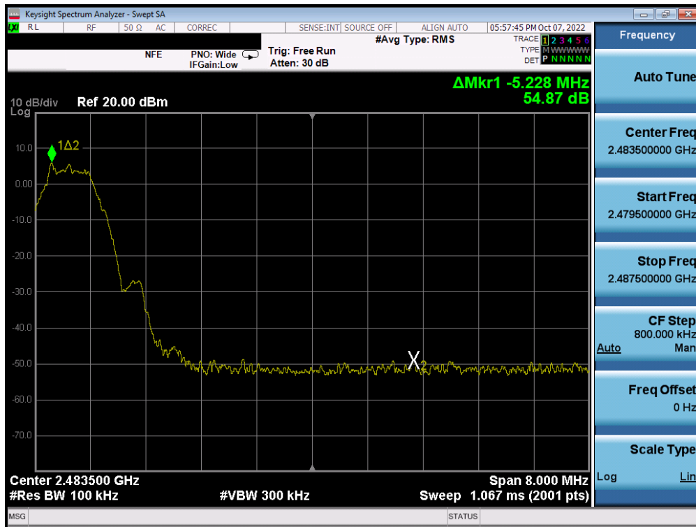
Plot 7-58. Band Edge Plot (Bluetooth (LE), 500kbps – Ch. 39) – ANT 1
