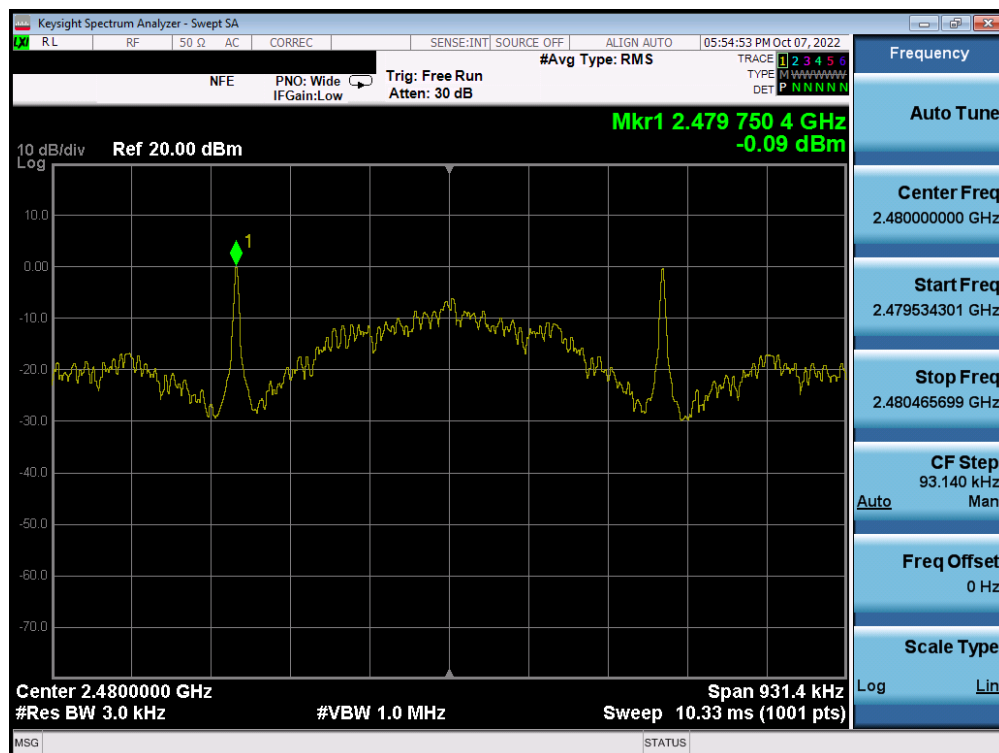
Plot 7-39. Power Spectral Density Plot (Bluetooth (LE), 125kbps – Ch. 39) – ANT 1
