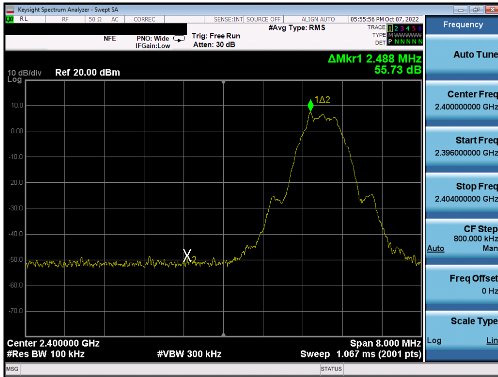
Plot 7-57. Band Edge Plot (Bluetooth (LE), 500kbps – Ch. 0) – ANT 1
