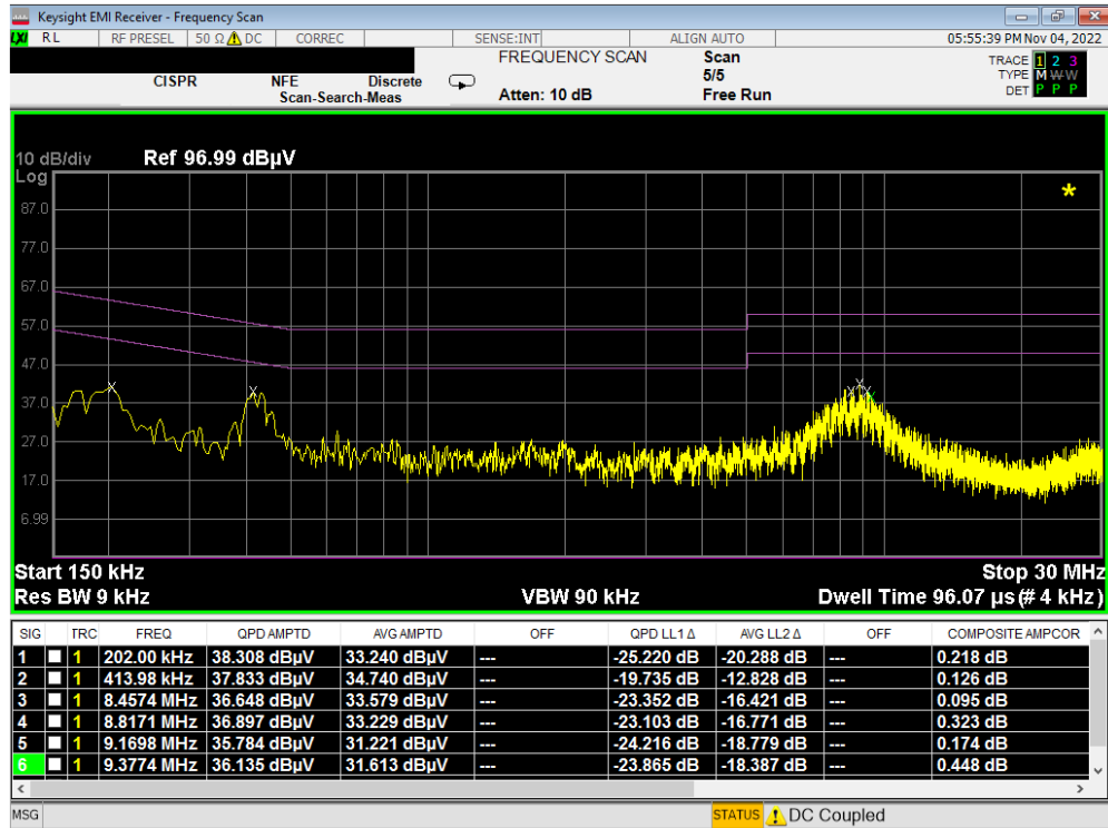
Plot 7-83. Line Conducted Plot with Bluetooth LE (L1)
