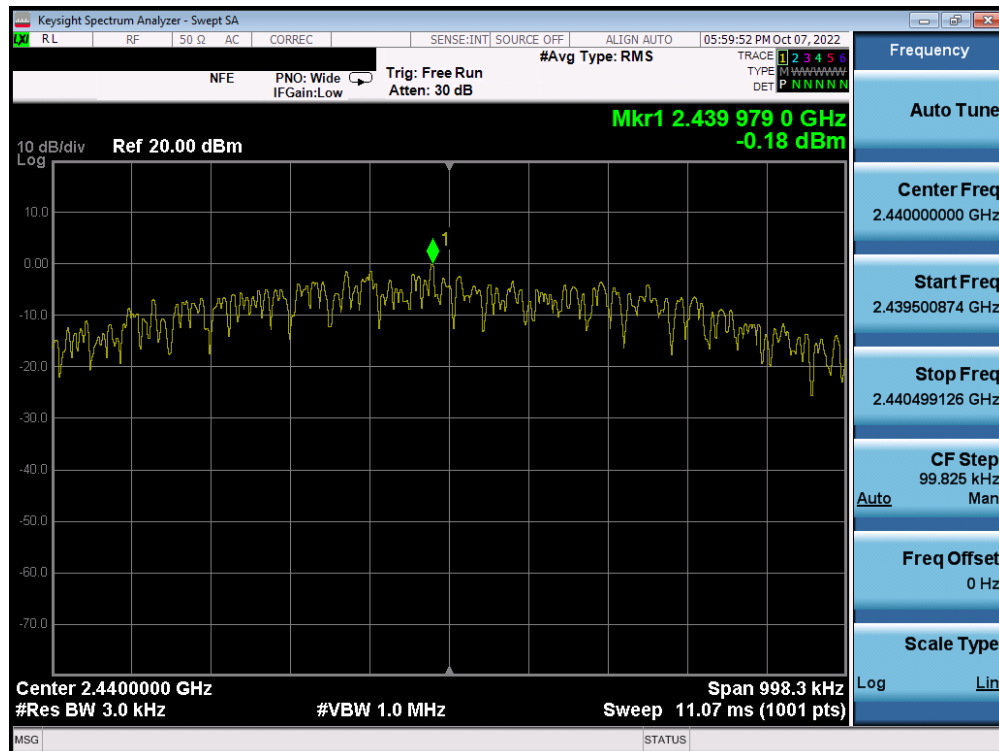
Plot 7-44. Power Spectral Density Plot (Bluetooth (LE), 1Mbps – Ch. 19) – ANT 1
