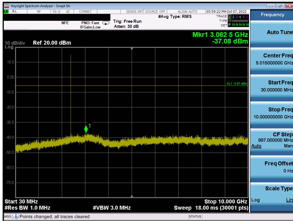
Plot 7-67. Conducted Spurious Plot (Bluetooth (LE), 1Mbps – Ch. 0) – ANT 1
