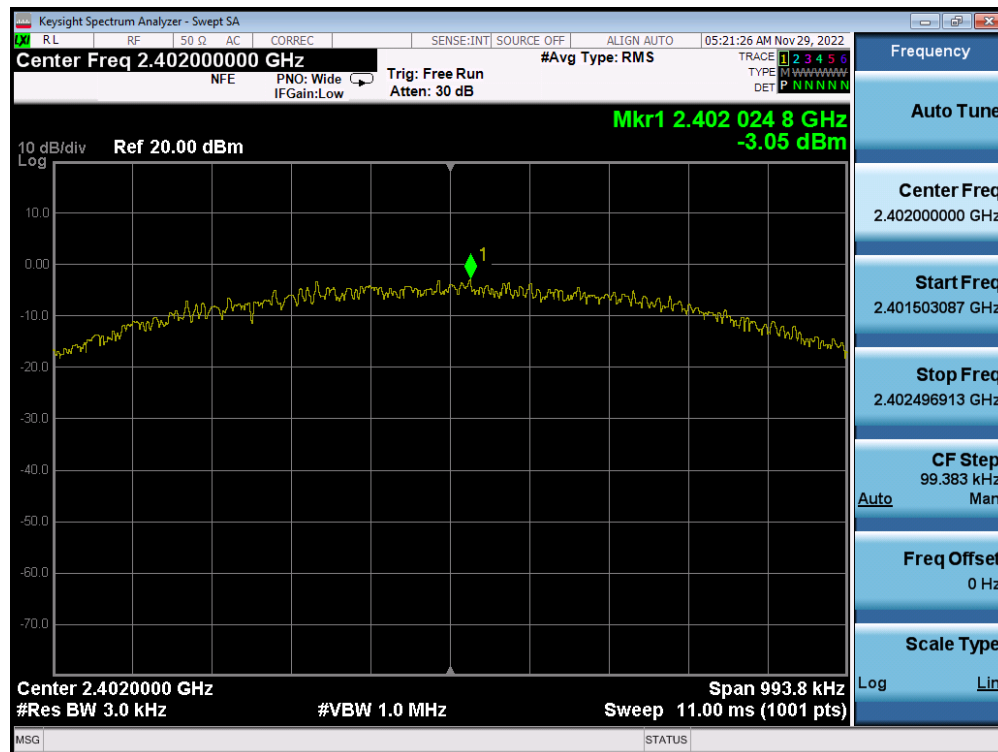
Plot 7-49. Power Spectral Density Plot (Bluetooth (LE), 1Mbps – Ch. 0) – ANT 2
