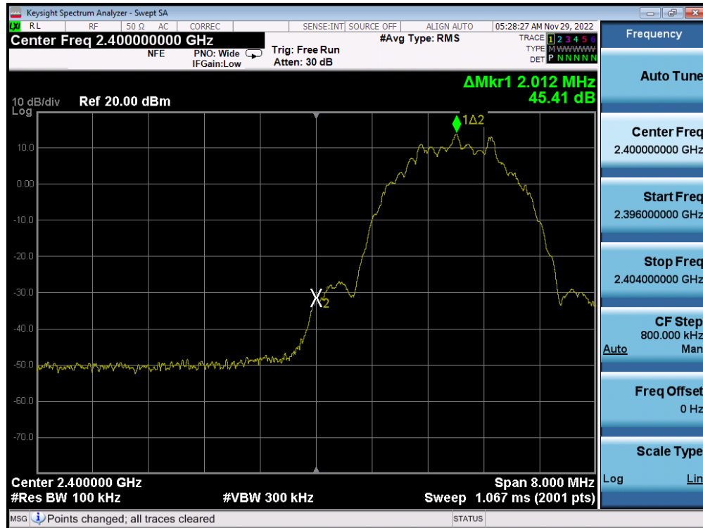
Plot 7-65. Band Edge Plot (Bluetooth (LE), 2Mbps – Ch. 0) – ANT 2
