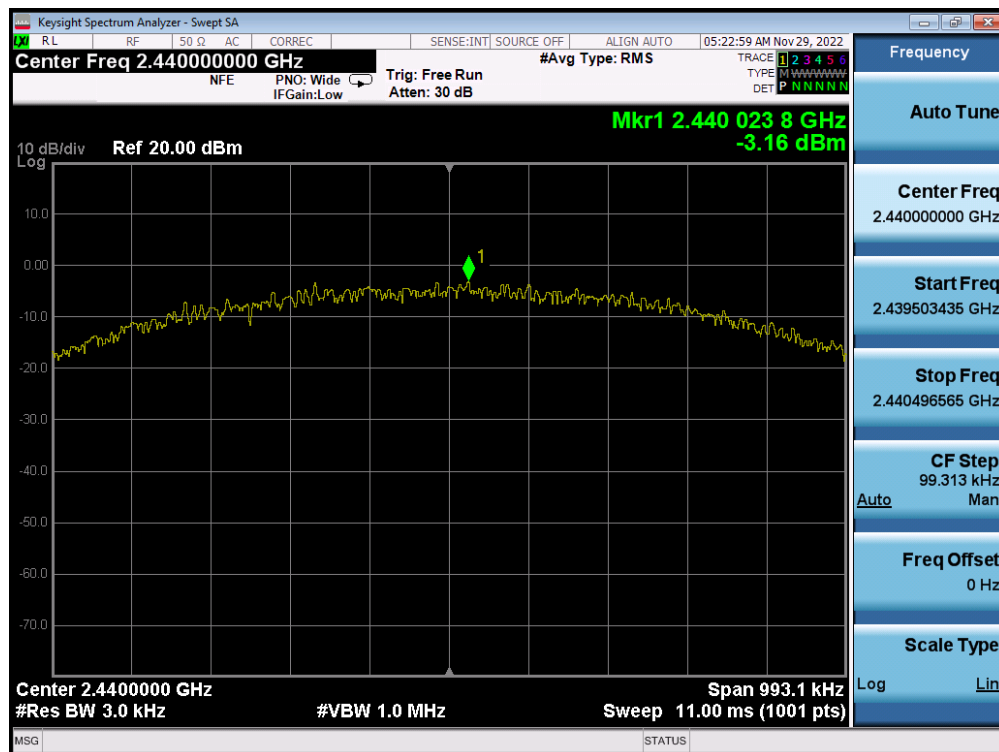
Plot 7-50. Power Spectral Density Plot (Bluetooth (LE), 1Mbps – Ch. 19) – ANT 2
