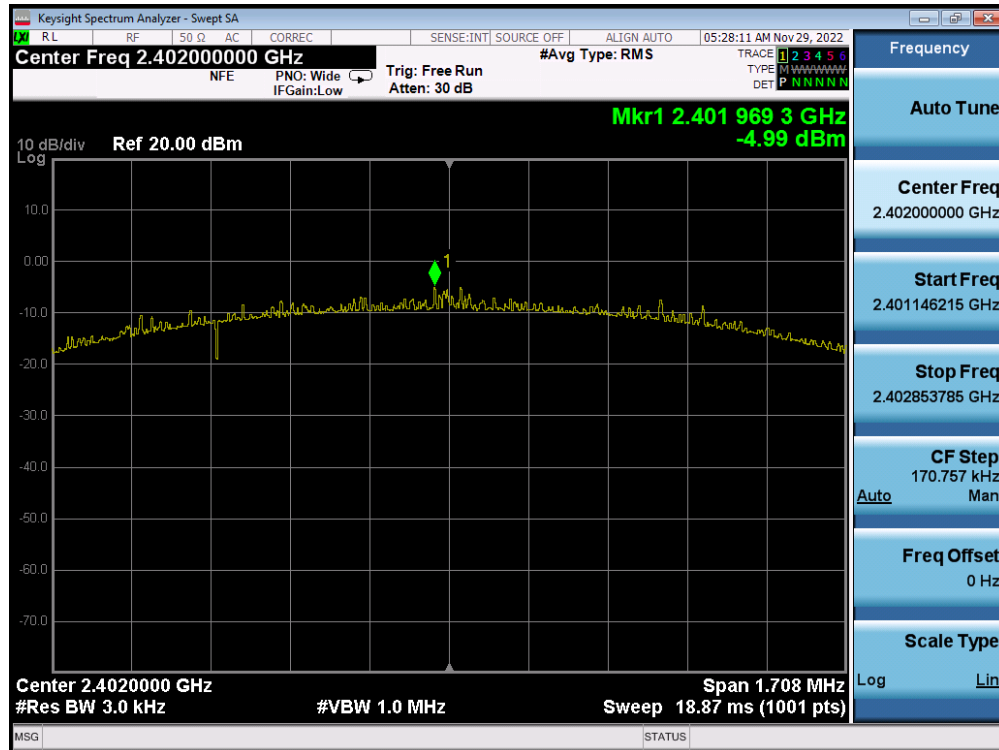
Plot 7-52. Power Spectral Density Plot (Bluetooth (LE), 2Mbps – Ch. 0) – ANT 2
