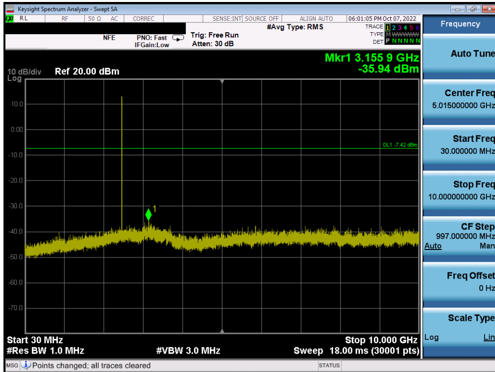
Plot 7-71. Conducted Spurious Plot (Bluetooth (LE), 1Mbps - Ch. 39) - ANT 1
