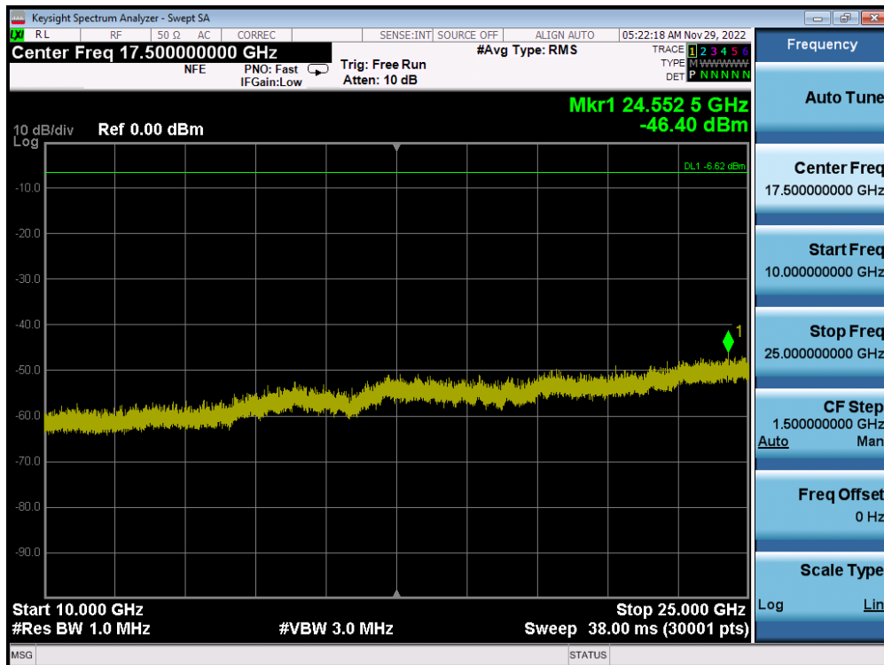
Plot 7-74. Conducted Spurious Plot (Bluetooth (LE), 1Mbps - Ch. 0) - ANT 2
