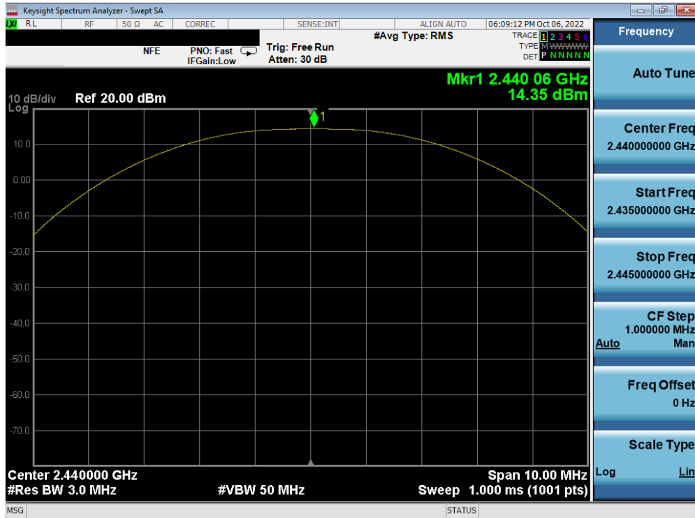
Plot 7-29. Peak Power Plot (Bluetooth (LE), 2Mbps – Ch. 19) – ANT 1
