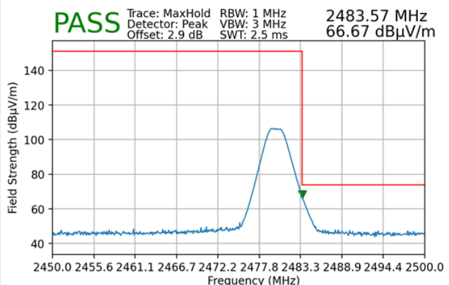
Plot 7-82. Radiated Restricted Upper Band Edge Measurement (Peak) – Ant2
