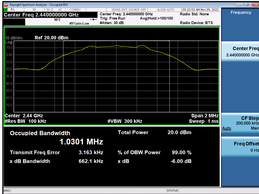
Plot 7-14. 6dB Bandwidth Plot (Bluetooth (LE), 1Mbps – Ch. 19) – ANT 2
