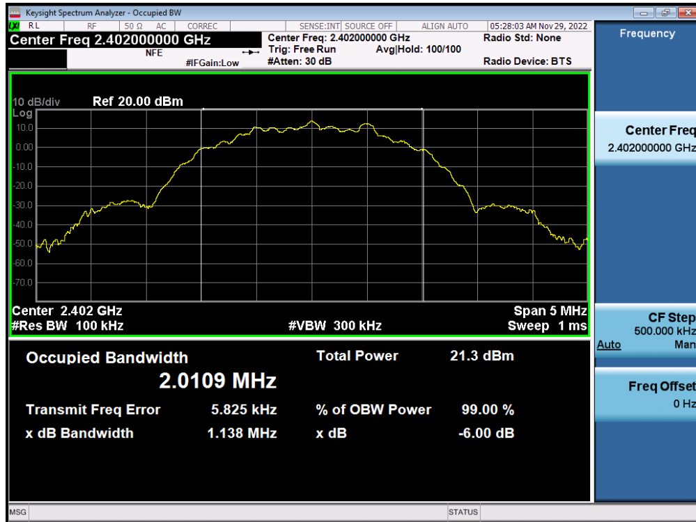
Plot 7-16. 6dB Bandwidth Plot (Bluetooth (LE), 2Mbps – Ch. 0) – ANT 2
