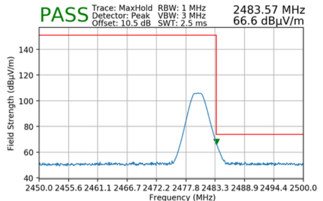
Plot 7-80. Radiated Restricted Upper Band Edge Measurement (Peak) – Ant1
