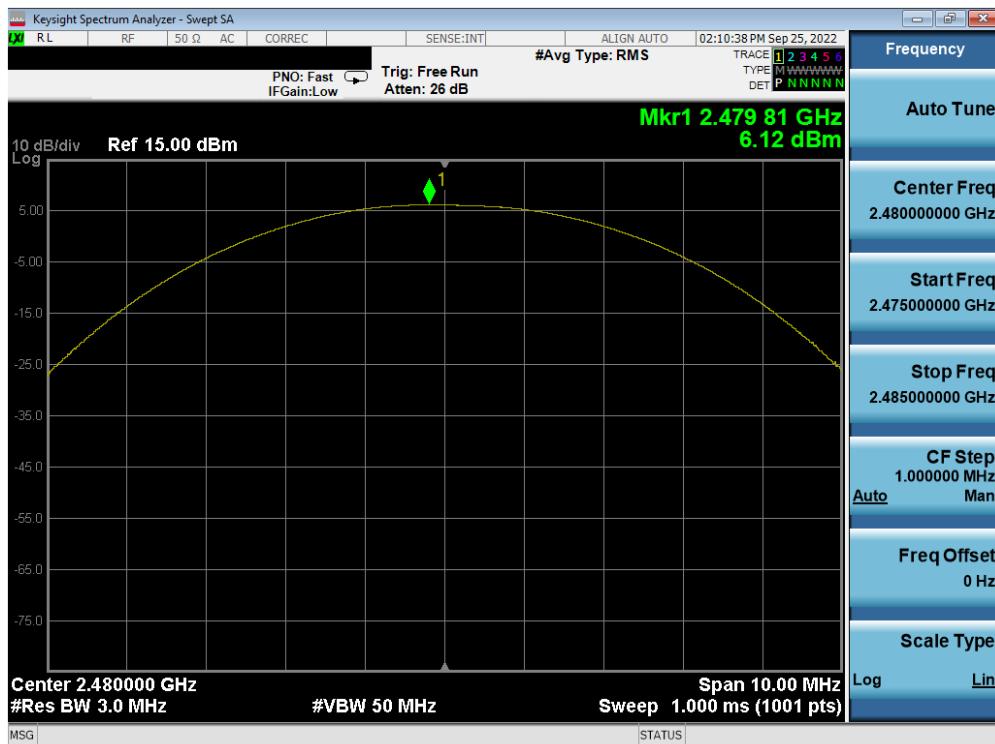
Plot 7-24. Peak Power Plot (Bluetooth (LE), 500kbps – Ch. 39) – ANT 1
