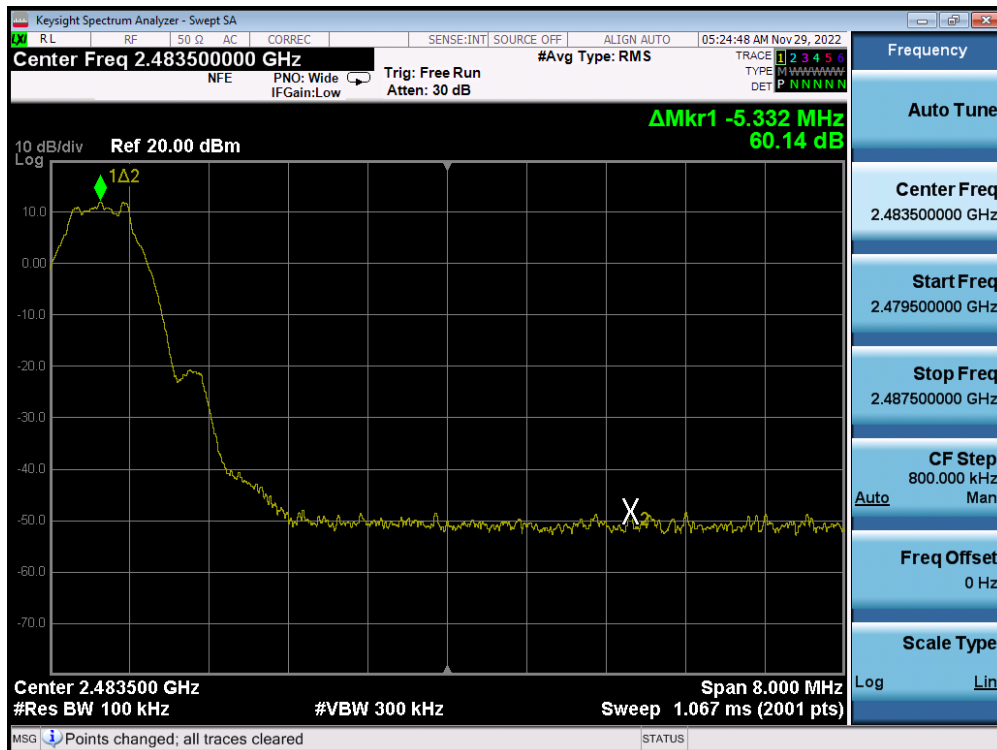
Plot 7-64. Band Edge Plot (Bluetooth (LE), 1Mbps - Ch. 39) - ANT 2
