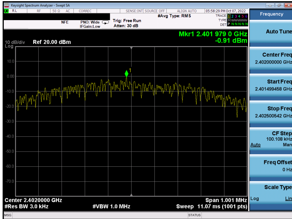
Plot 7-43. Power Spectral Density Plot (Bluetooth (LE), 1Mbps – Ch. 0) – ANT 1
