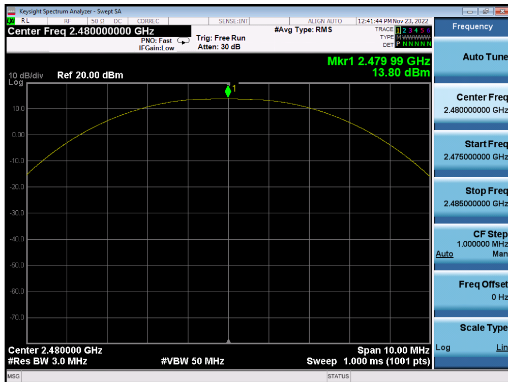
Plot 7-36. Peak Power Plot (Bluetooth (LE), 2Mbps – Ch. 39) – ANT 2
