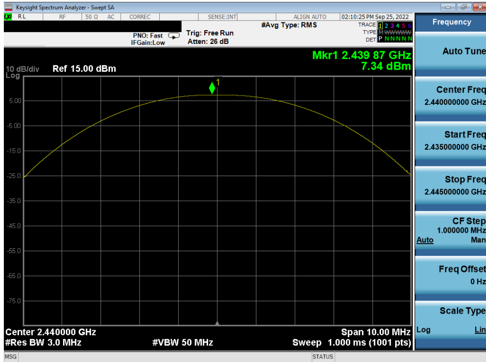
Plot 7-23. Peak Power Plot (Bluetooth (LE), 500kbps – Ch. 19) – ANT 1
