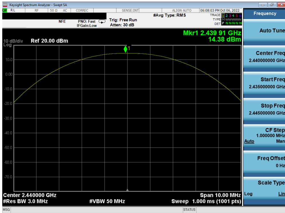
Plot 7-26. Peak Power Plot (Bluetooth (LE), 1Mbps – Ch. 19) – ANT 1
