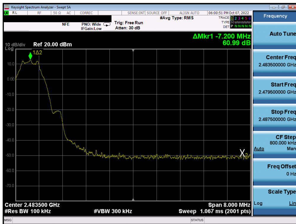
Plot 7-60. Band Edge Plot (Bluetooth (LE), 1Mbps – Ch. 39) – ANT 1
