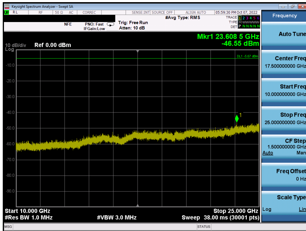
Plot 7-68. Conducted Spurious Plot (Bluetooth (LE), 1Mbps – Ch. 0) – ANT 1
