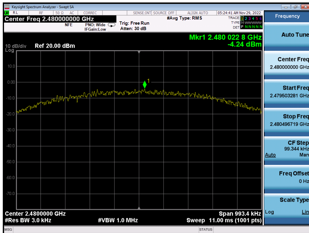
Plot 7-51. Power Spectral Density Plot (Bluetooth (LE), 1Mbps – Ch. 39) – ANT 2
