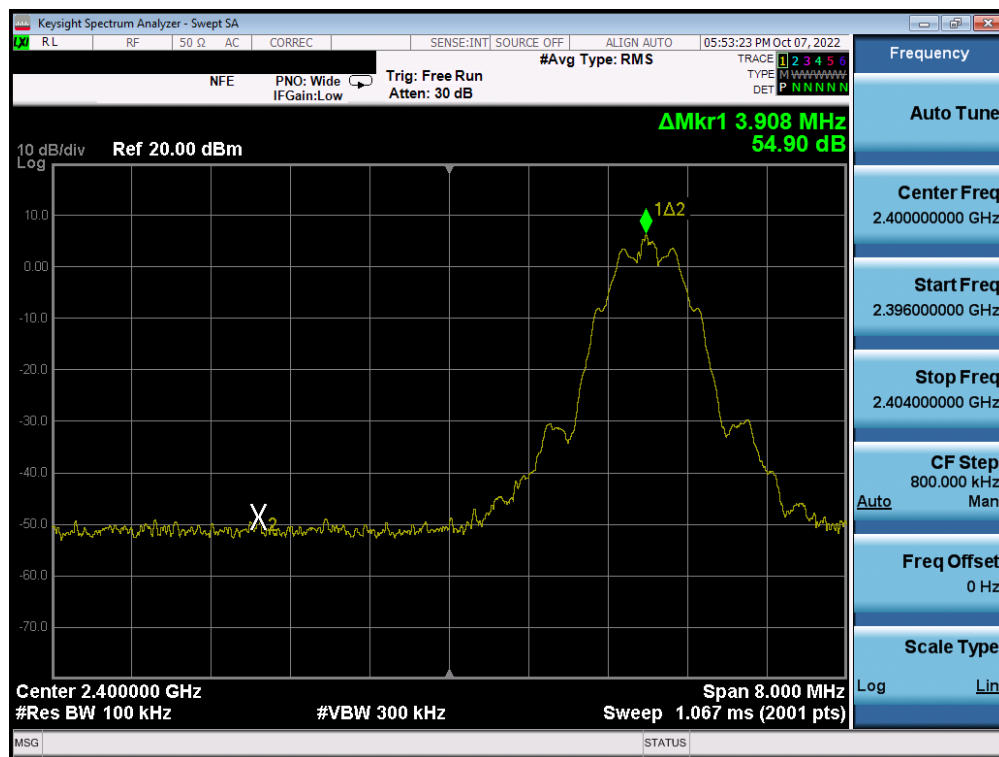
Plot 7-55. Band Edge Plot (Bluetooth (LE), 125kbps – Ch. 0) – ANT 1
