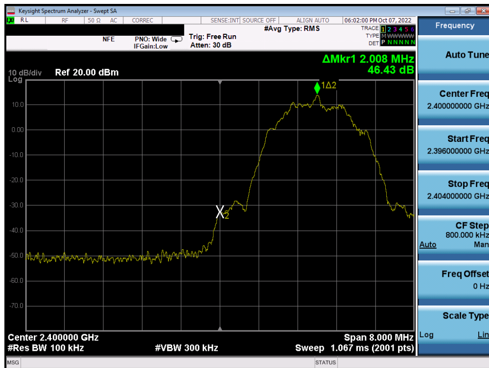
Plot 7-61. Band Edge Plot (Bluetooth (LE), 2Mbps - Ch. 0) - ANT 1
