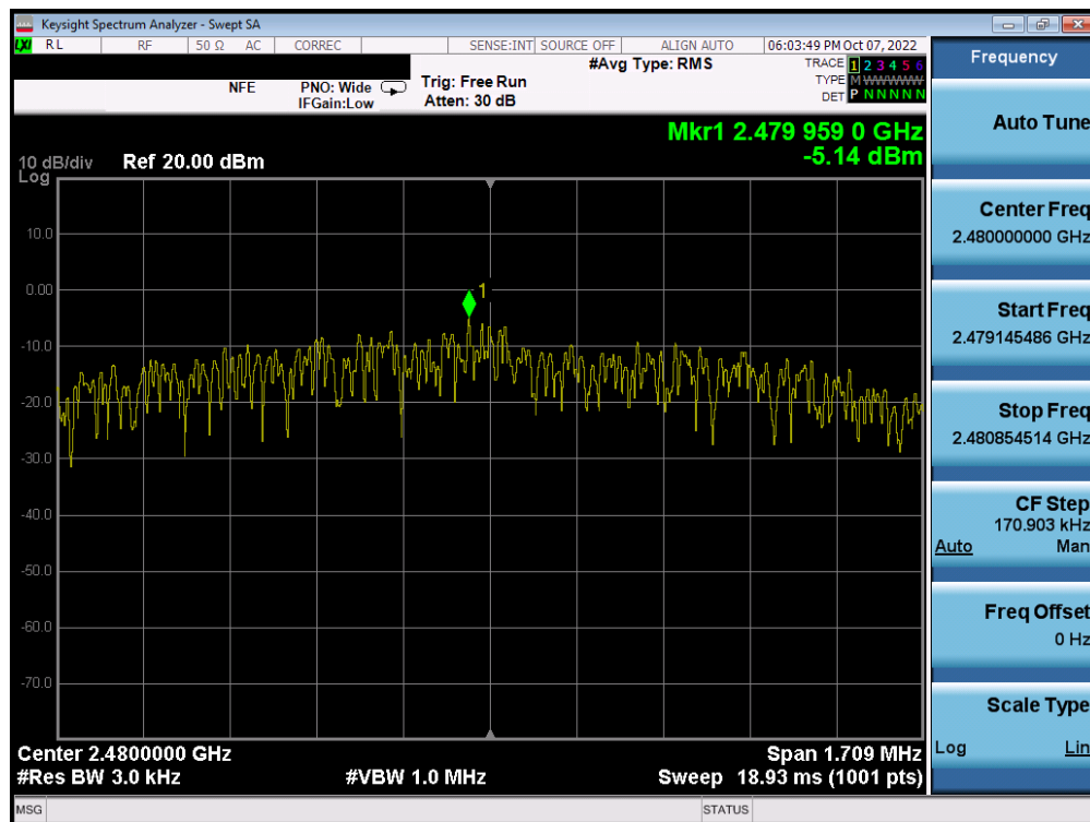
Plot 7-48. Power Spectral Density Plot (Bluetooth (LE), 2Mbps – Ch. 39) – ANT 1
