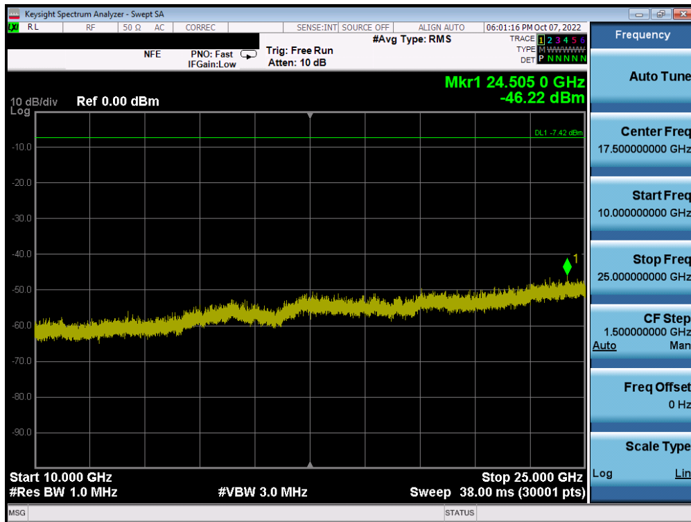
Plot 7-72. Conducted Spurious Plot (Bluetooth (LE), 1Mbps - Ch. 39) - ANT 1
