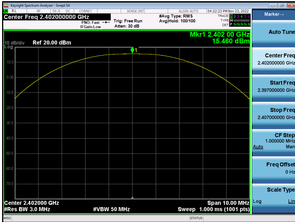
Plot 7-34. Peak Power Plot (Bluetooth (LE), 2Mbps – Ch. 0) – ANT 2
