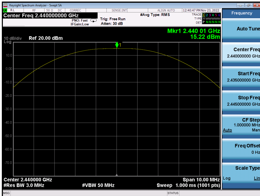
Plot 7-35. Peak Power Plot (Bluetooth (LE), 2Mbps – Ch. 19) – ANT 2
