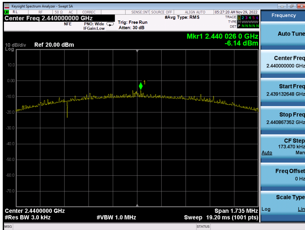
Plot 7-53. Power Spectral Density Plot (Bluetooth (LE), 2Mbps – Ch. 19) – ANT 2
