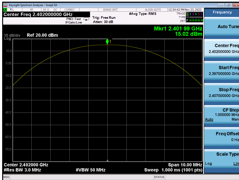
Plot 7-31. Peak Power Plot (Bluetooth (LE), 1Mbps – Ch. 0) – ANT 2
