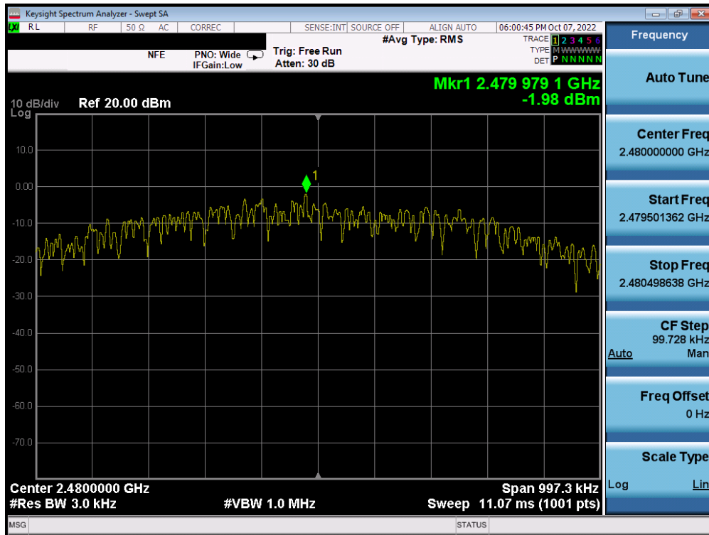
Plot 7-45. Power Spectral Density Plot (Bluetooth (LE), 1Mbps – Ch. 39) – ANT 1
