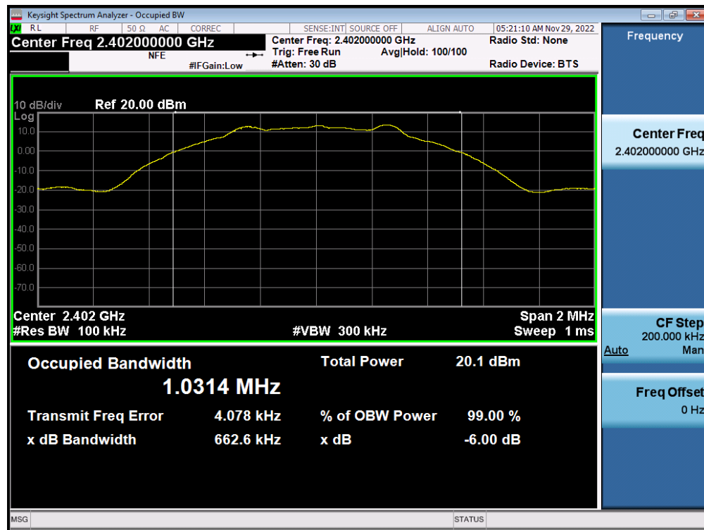
Plot 7-13. 6dB Bandwidth Plot (Bluetooth (LE), 1Mbps – Ch. 0) – ANT 2
