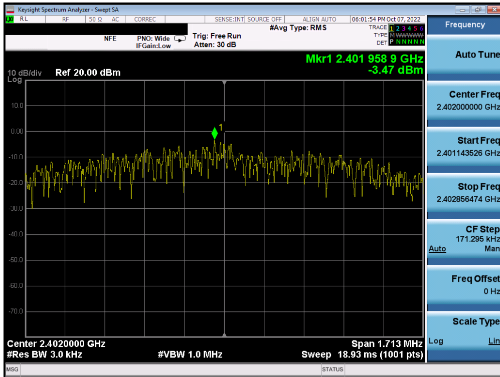
Plot 7-46. Power Spectral Density Plot (Bluetooth (LE), 2Mbps – Ch. 0) – ANT 1
