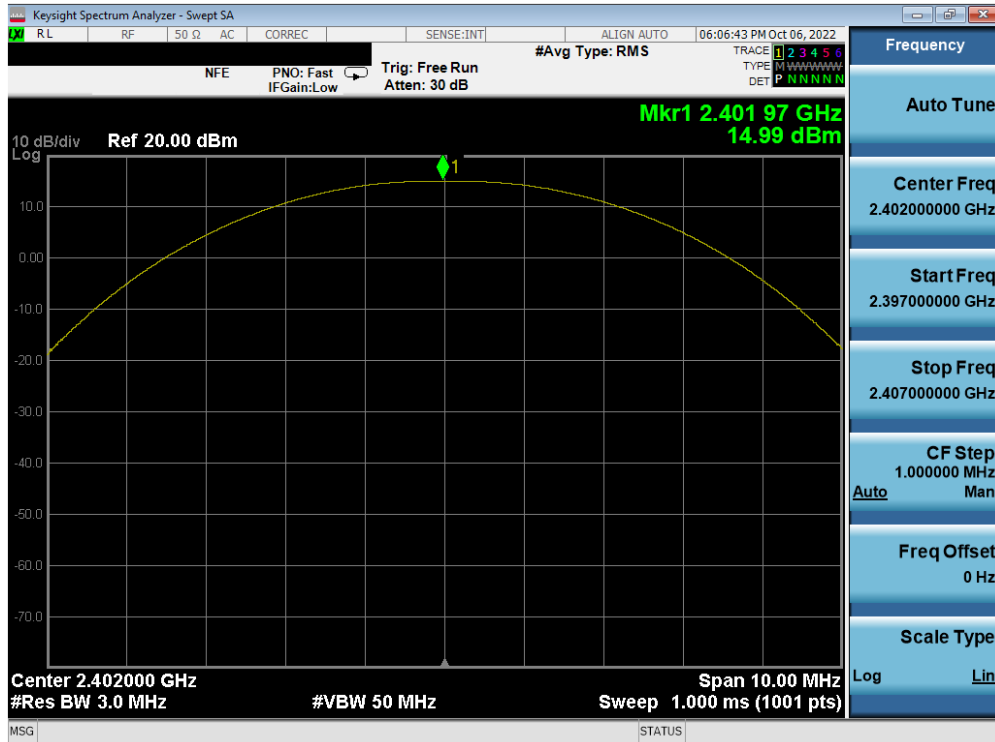
Plot 7-25. Peak Power Plot (Bluetooth (LE), 1Mbps – Ch. 0) – ANT 1
