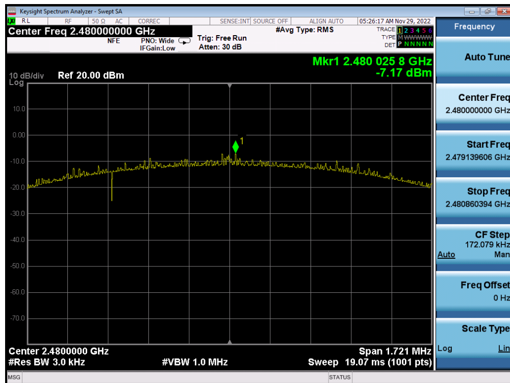
Plot 7-54. Power Spectral Density Plot (Bluetooth (LE), 2Mbps – Ch. 39) – ANT 2
