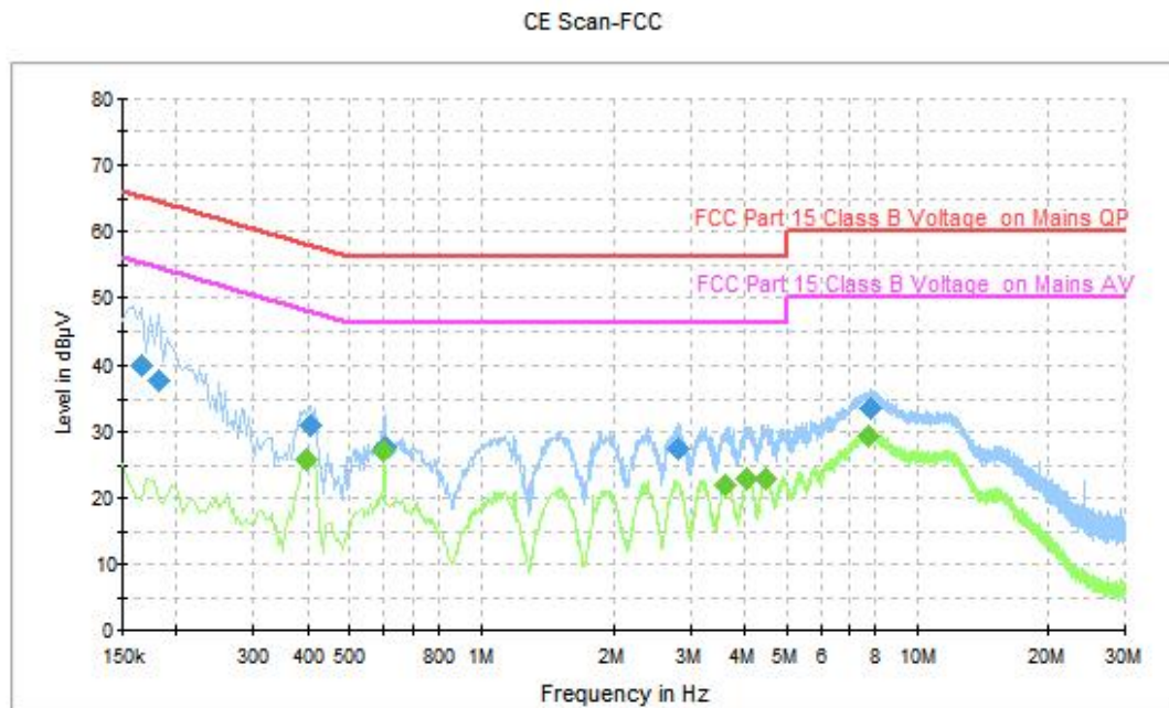
Fig.70 AC Power line Conducted Emission (Traffic)
