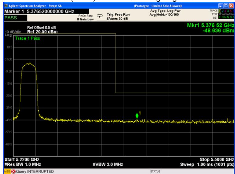
802.11ac(HT20) U-NII-1 Band edge-right side
