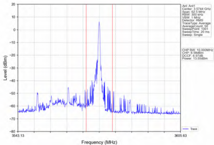
n78d_15kHz_SISO_NTNV_25MHz_CP-OFDM QPSK_3562.5MHz_Edge_1RB_Right
