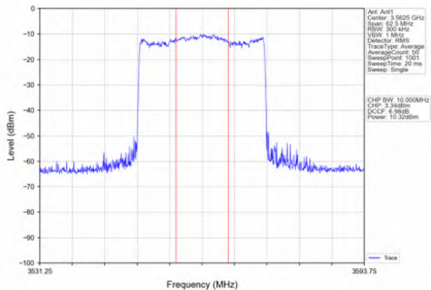
n78d 15kHz SISO NTNv 25MHz CP-OFDM 16 QAM 3562.5MHz Inner Full
