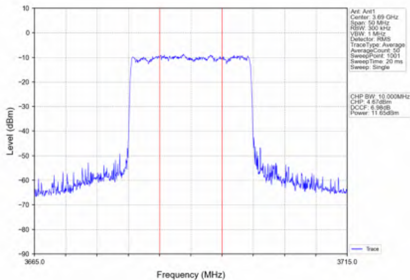
n78d_15kHz_SISO_NTV_20MHz_CP-OFDM_16_QAM_3690MHz_Inner_Full
