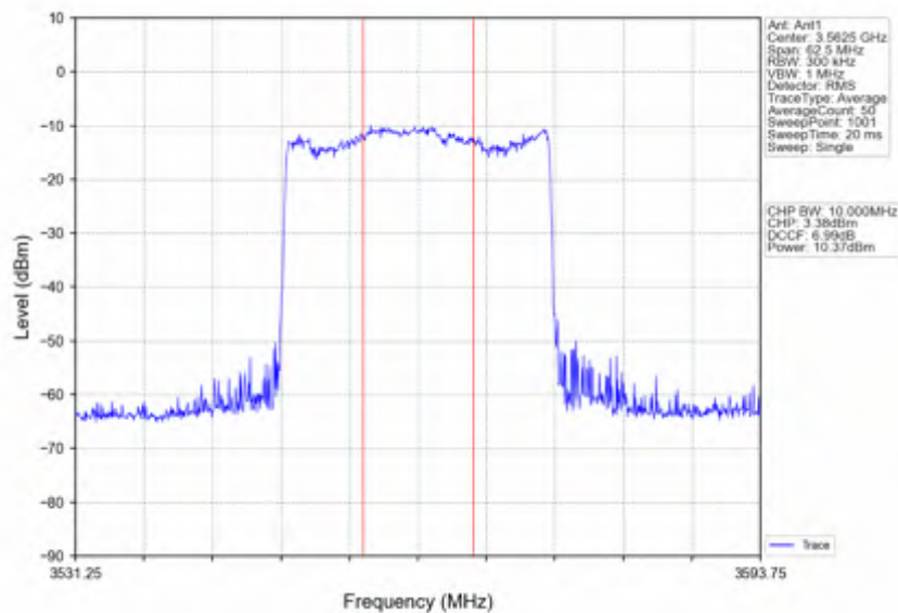
n78d_15kHz_SISO_NTNV_25MHz_CP-OFDM_256_QAM_3562.5MHz_Inner_Full
