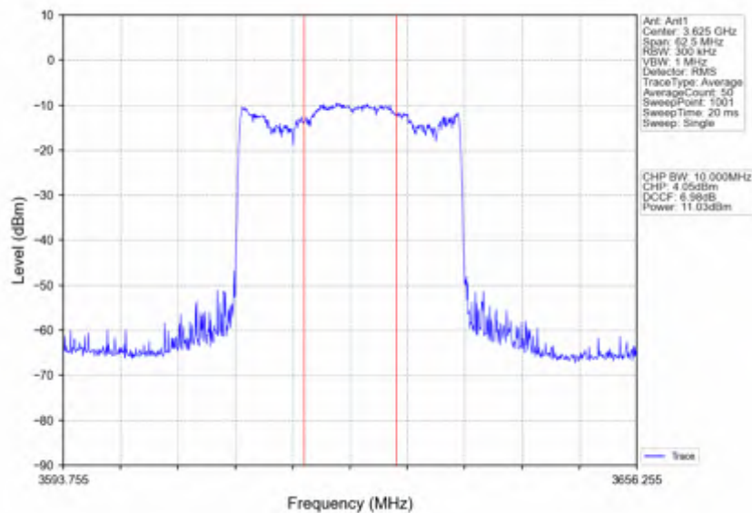
n78d_15kHz_SISO_NTNV_25MHz_CP-OFDM QPSK_3625.005MHz_Inner_Full
