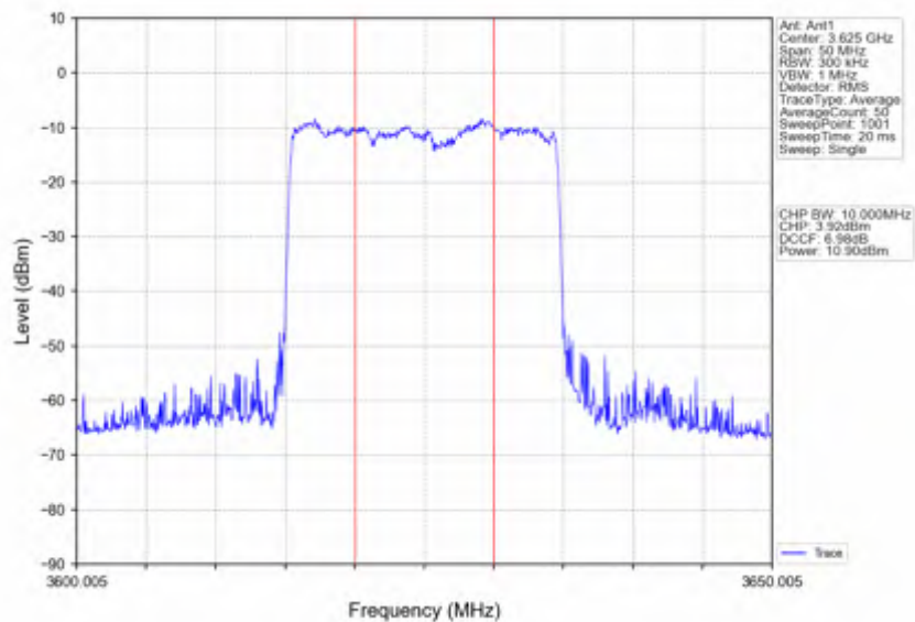
n78d_15kHz_SISO_NTNV_20MHz_CP-OFDM 256 QAM_3625.005MHz_Inner_Full
