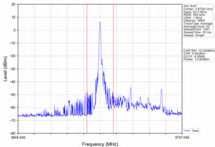
n78d_15kHz_SISO_NTNV_25MHz_DFT-s-OFDM_QPSK_3687.495MHz_Inner_1RB_Right
