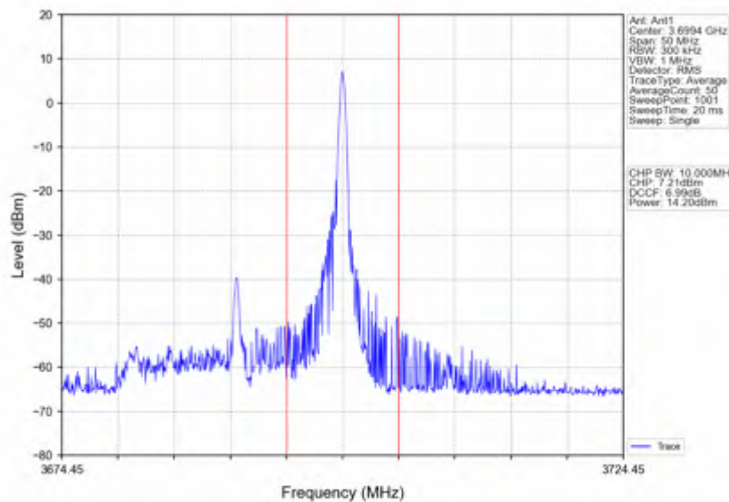
n78d_15kHz_SISO_NTNV_20MHz_DFT-s-OFDM_256_QAM_3690MHz_Edge_1RB_Right
