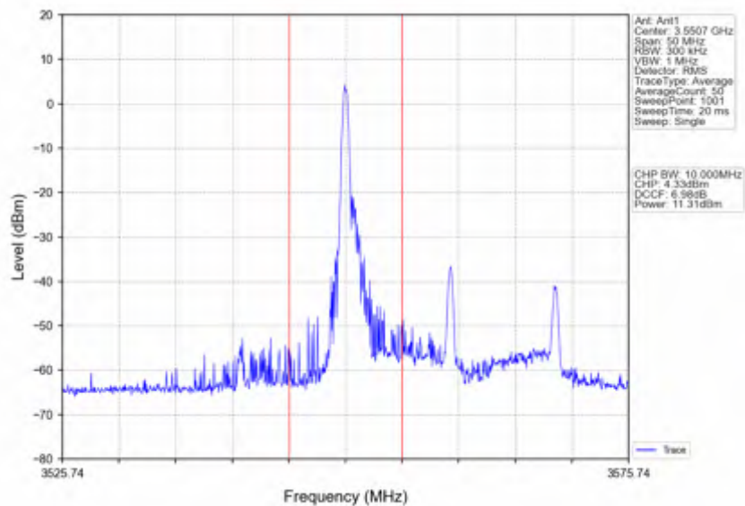
n78d_15kHz_SISO_NTNV_20MHz_CP-OFDM_16_QAM_3560.01MHz_Inner_1RB_Right
