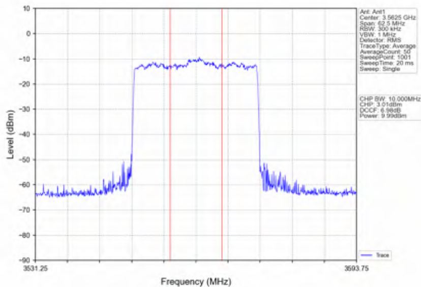
n78d_15kHz_SISO_NTNV_25MHz_CP-OFDM_QPSK_3562.5MHz_Inner_Full
