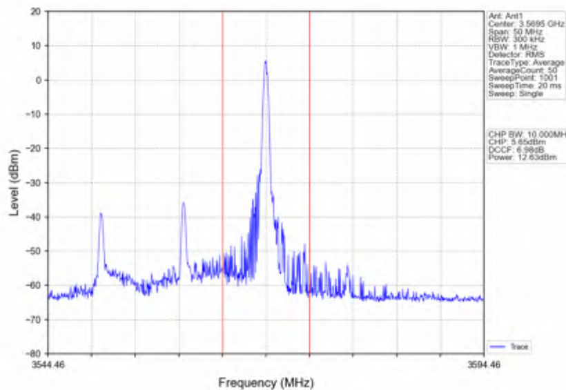
n78d_15kHz_SISO_NTNV_20MHz_CP-OFDM 16 QAM_3560.01MHz_Edge_1RB_Right
