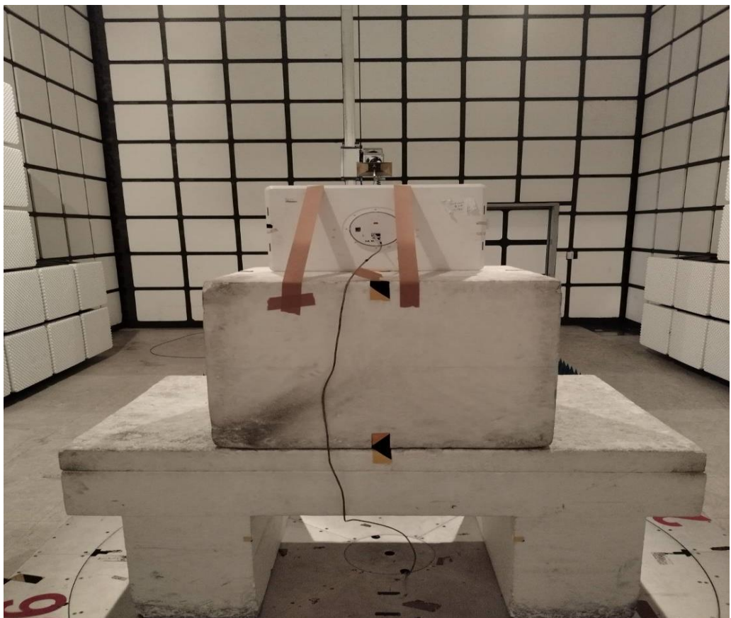
Rear View
