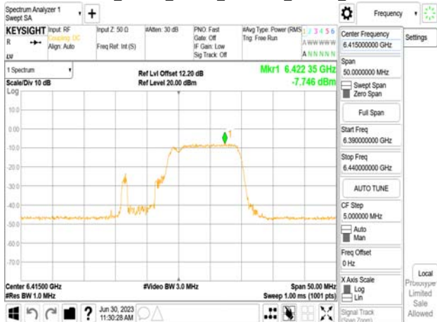
802.11be_20MHz_Chain0_6415MHz_106+26_MR02
